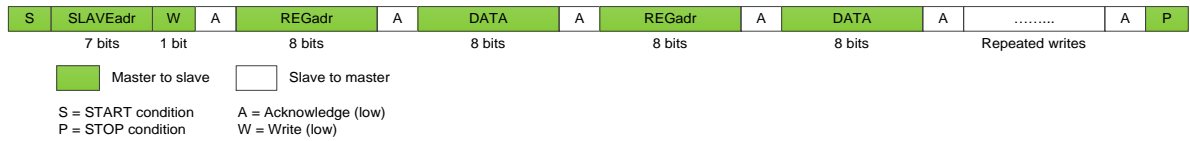
Figure 31: 2-WIRE Repeated Write (SI/DATA Line)
