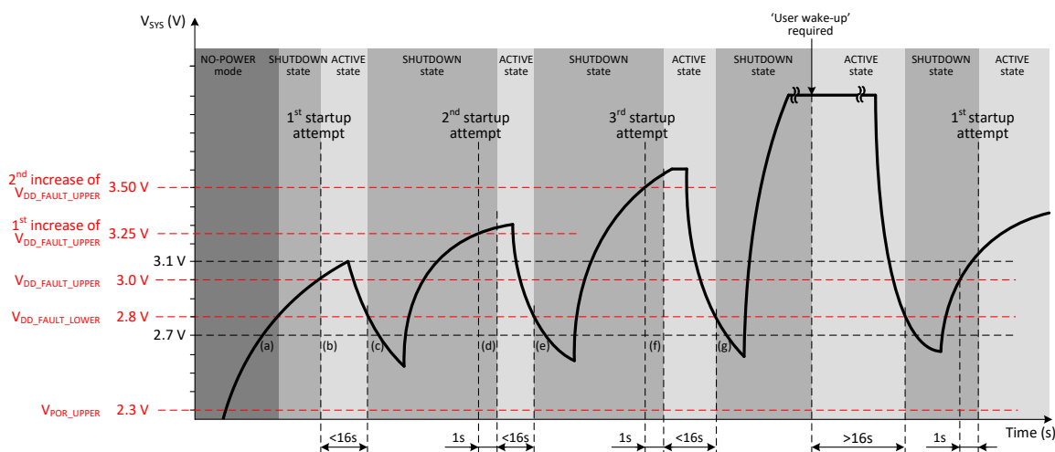
Figure 16: VDD START Faults
