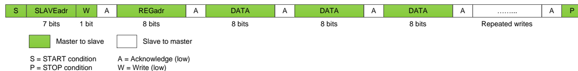
Figure 30: 2-WIRE Page Write (SI/DATA Line)
