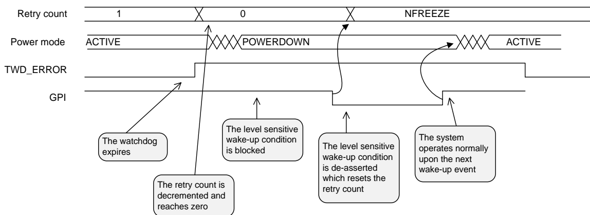
Figure 18: Freeze Function
