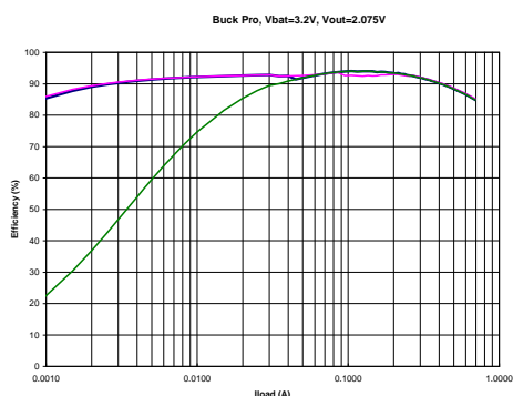
Figure 10: BUCKPRO efficiency curves
