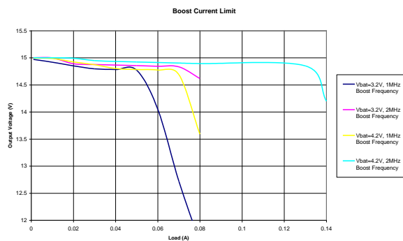
Figure 28: Boost regulation voltages
