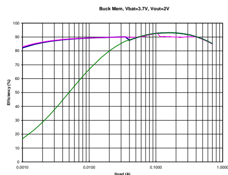
Figure 11: BUCKMEM efficiency curves
