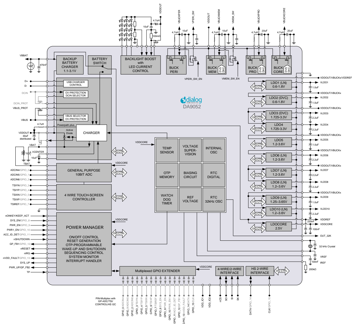
Figure 1: Block diagram
