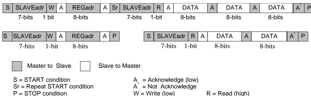
Figure 38: Examples of 2-wire page read (SO/DATA line)
