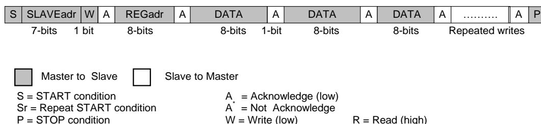
Figure 39: 2-wire page write (SO/DATA line)
