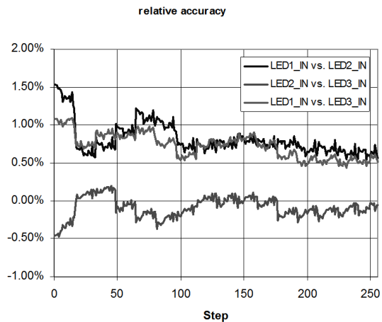
Figure 26: Relative accuracy
