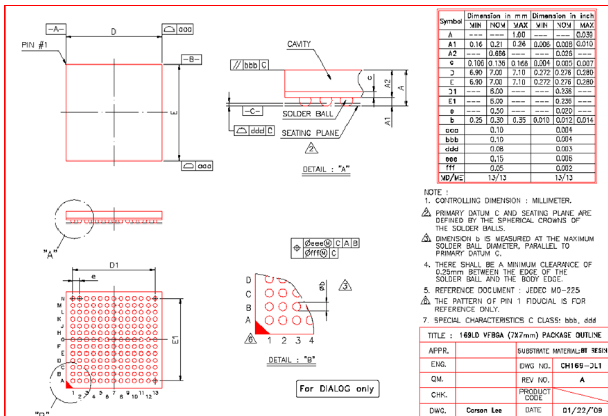
Figure 59: 169 BGA (7 x 7 mm), bottom view
