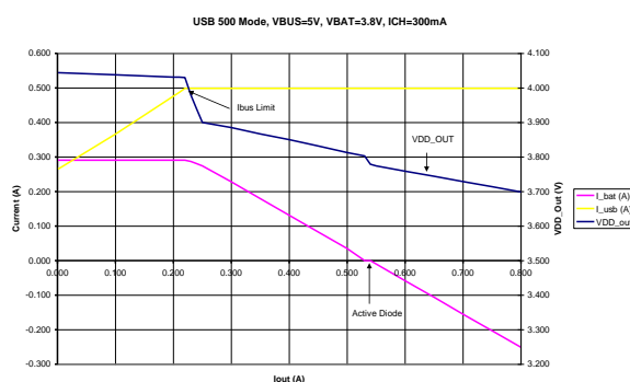
Figure 22: Power path behaviour USB500 mode
