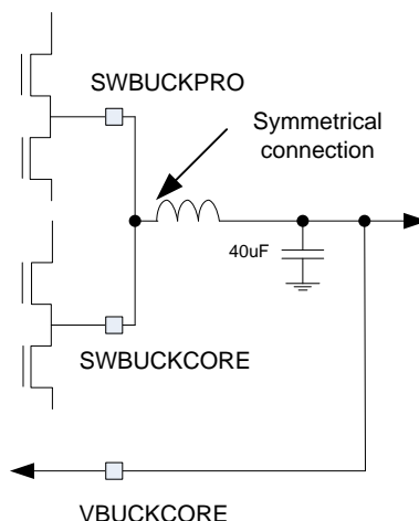
Figure 49: BUCKCORE merged with BUCKPRO
