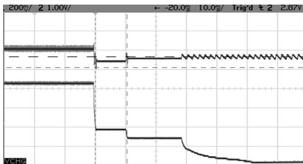
Figure 24: Transitioning supply from USB 5 V (via VBUS) to VBAT
