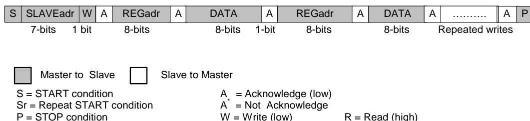
Figure 40: 2-wire repeated write (SO/DATA line)
