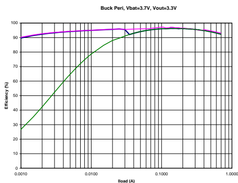
Figure 8: BUCKPERI efficiency curves
