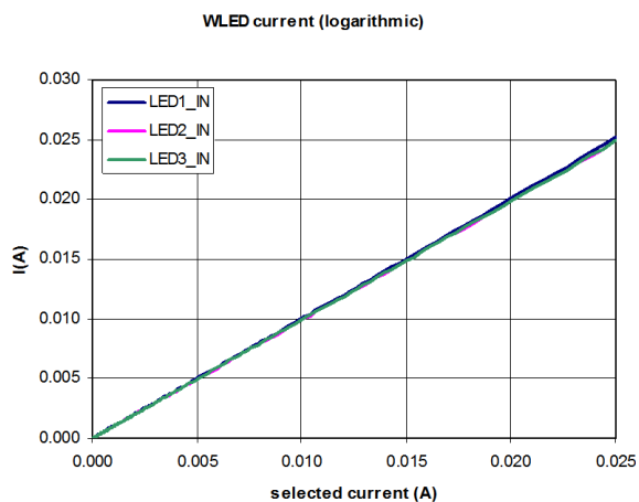
Figure 25: WLED current (logarithmic)
