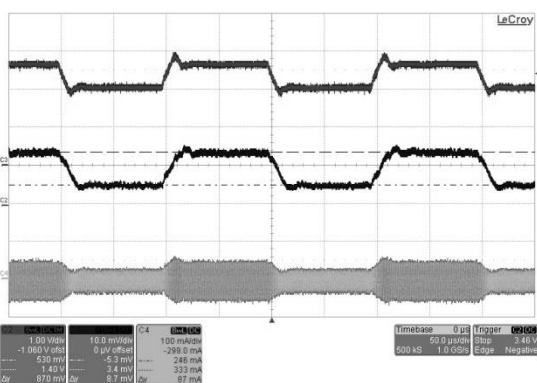
Figure 12: Typical buck line transient
