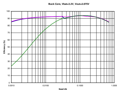
Figure 9: BUCKCORE efficiency curves
