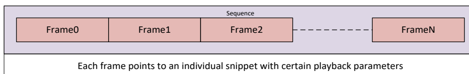
Figure 28: Sequence Structure
