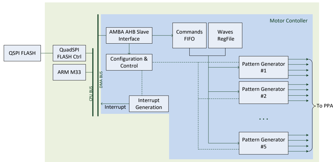
Figure 47: Motor Controller Block Diagram
