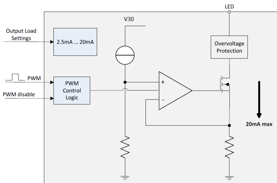
Figure 105: LED Driver Block Diagram
