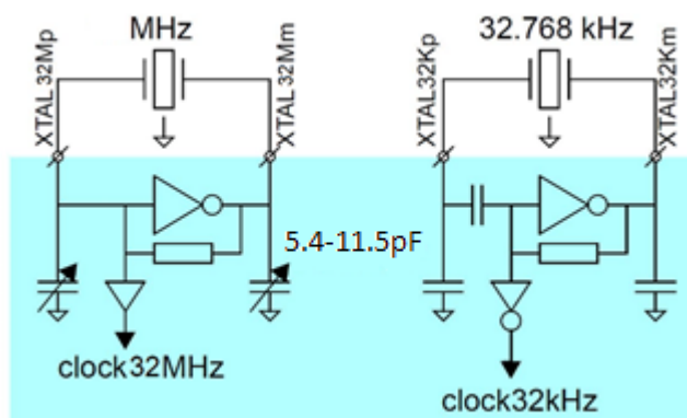
Figure 36: Crystal Oscillator Circuits
