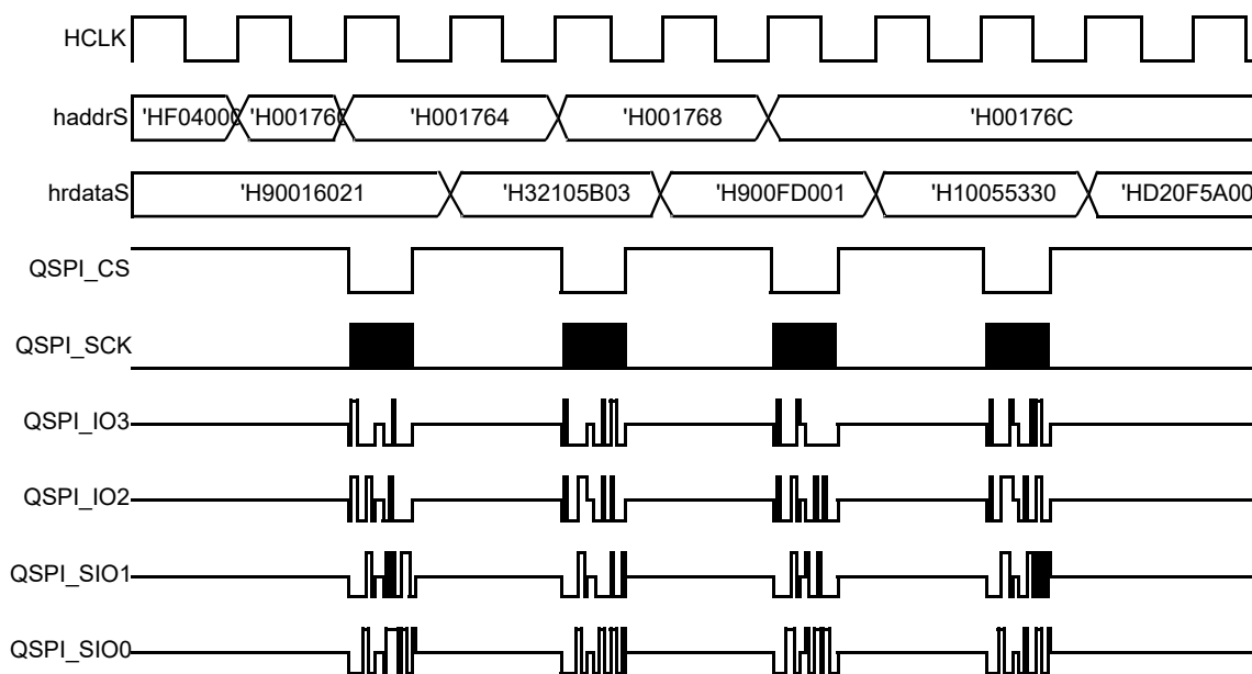
Figure 45: QSPI Split Burst Timing for Low Power (QSPI_FORENSEQ_EN=1)
