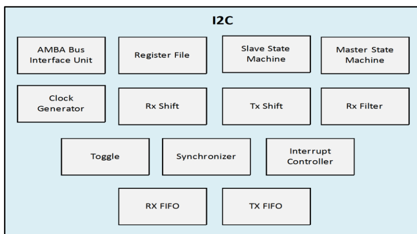
Figure 69: I2C Controller Block Diagram
