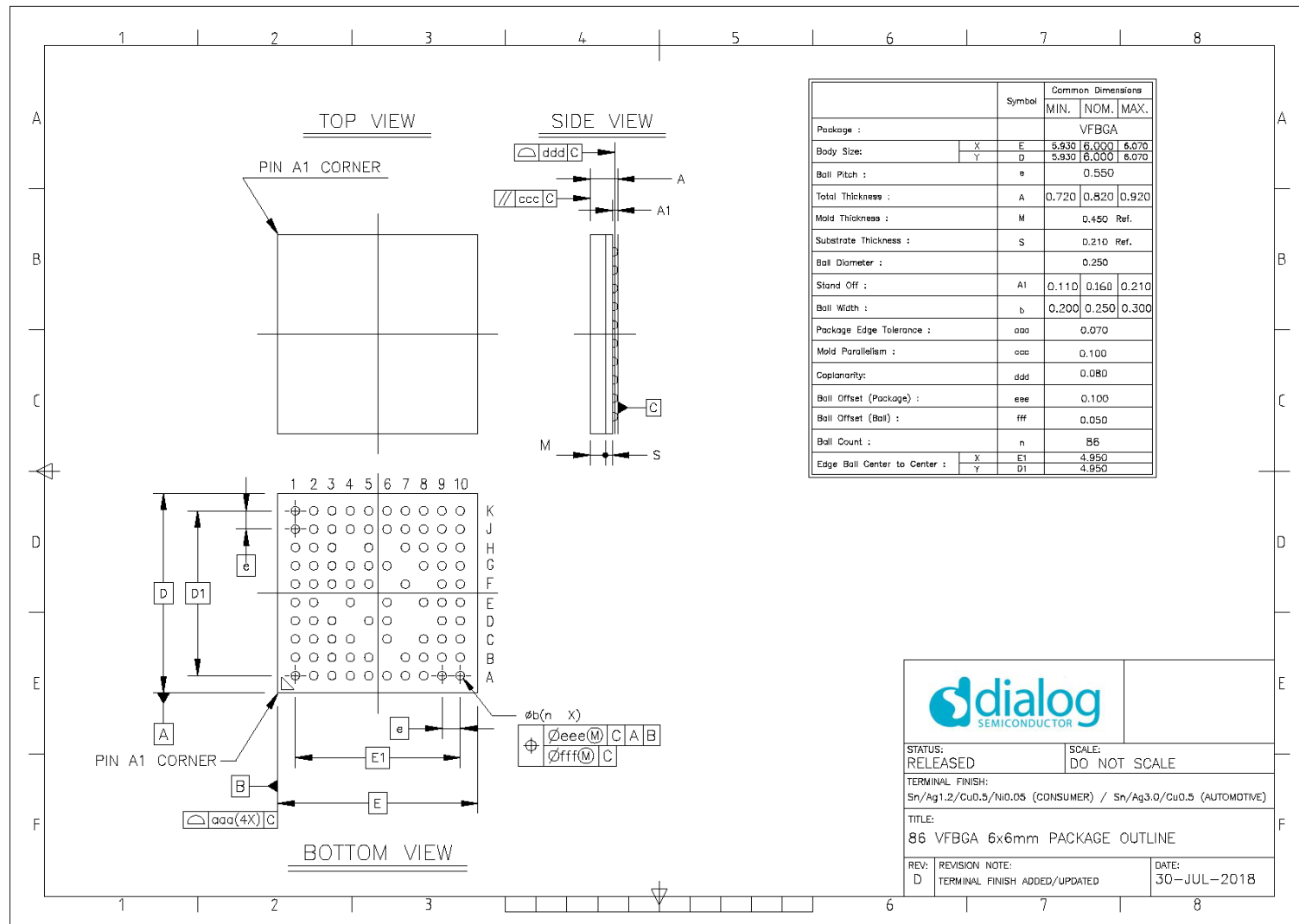
Figure 110: VFBGA86 Package Outline Drawing
