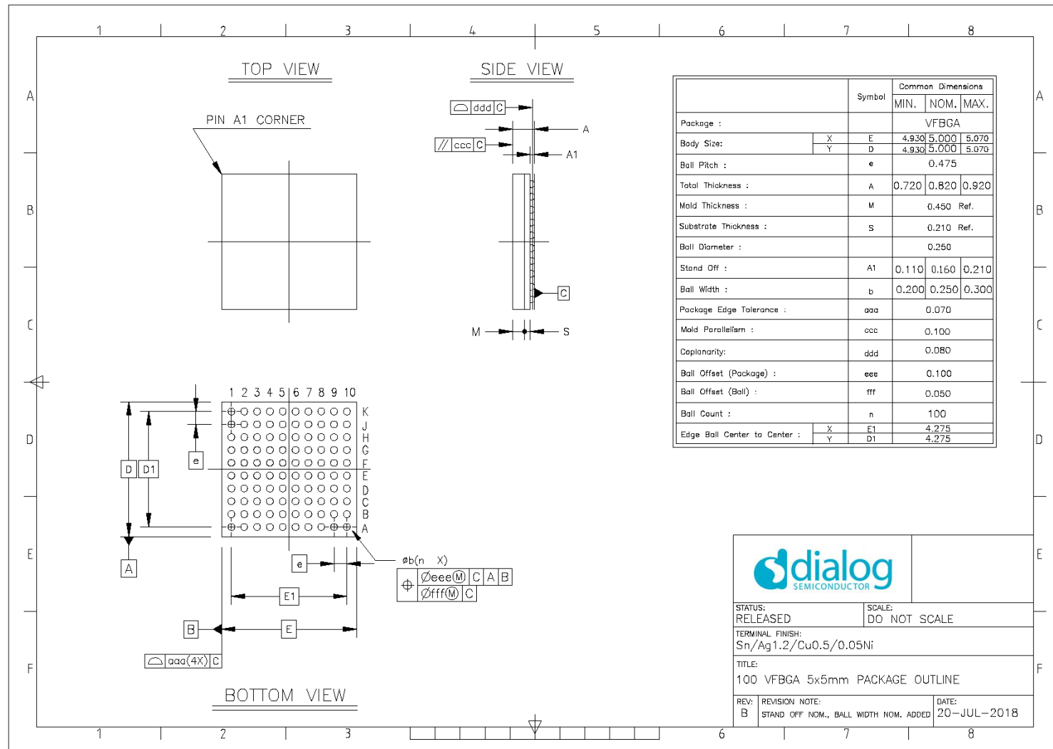
Figure 111: VFBGA100 Package Outline Drawing
