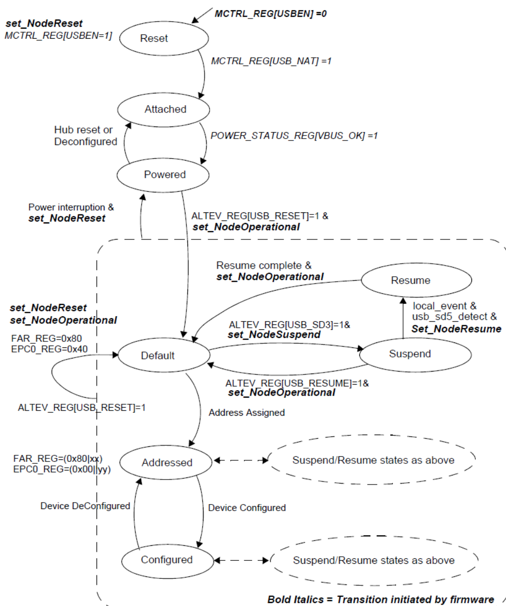
Figure 95: Node Functional State Diagram
