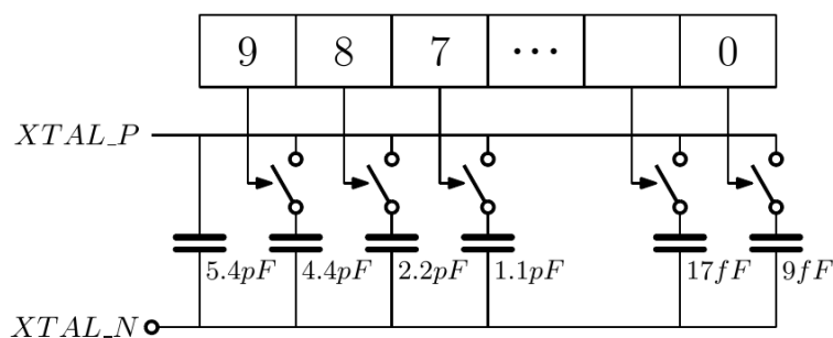
Figure 37: XTAL32MHz Oscillator Frequency Trimming
