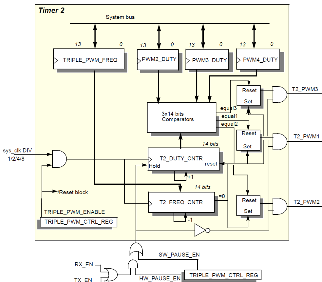
Figure 58: Timer 2 PWM Block Diagram
