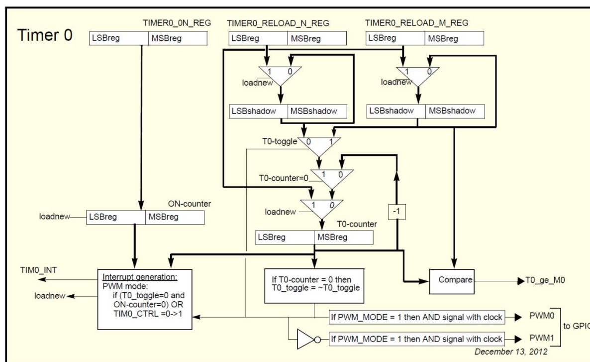
Figure 56: Timer 0 Block Diagram
