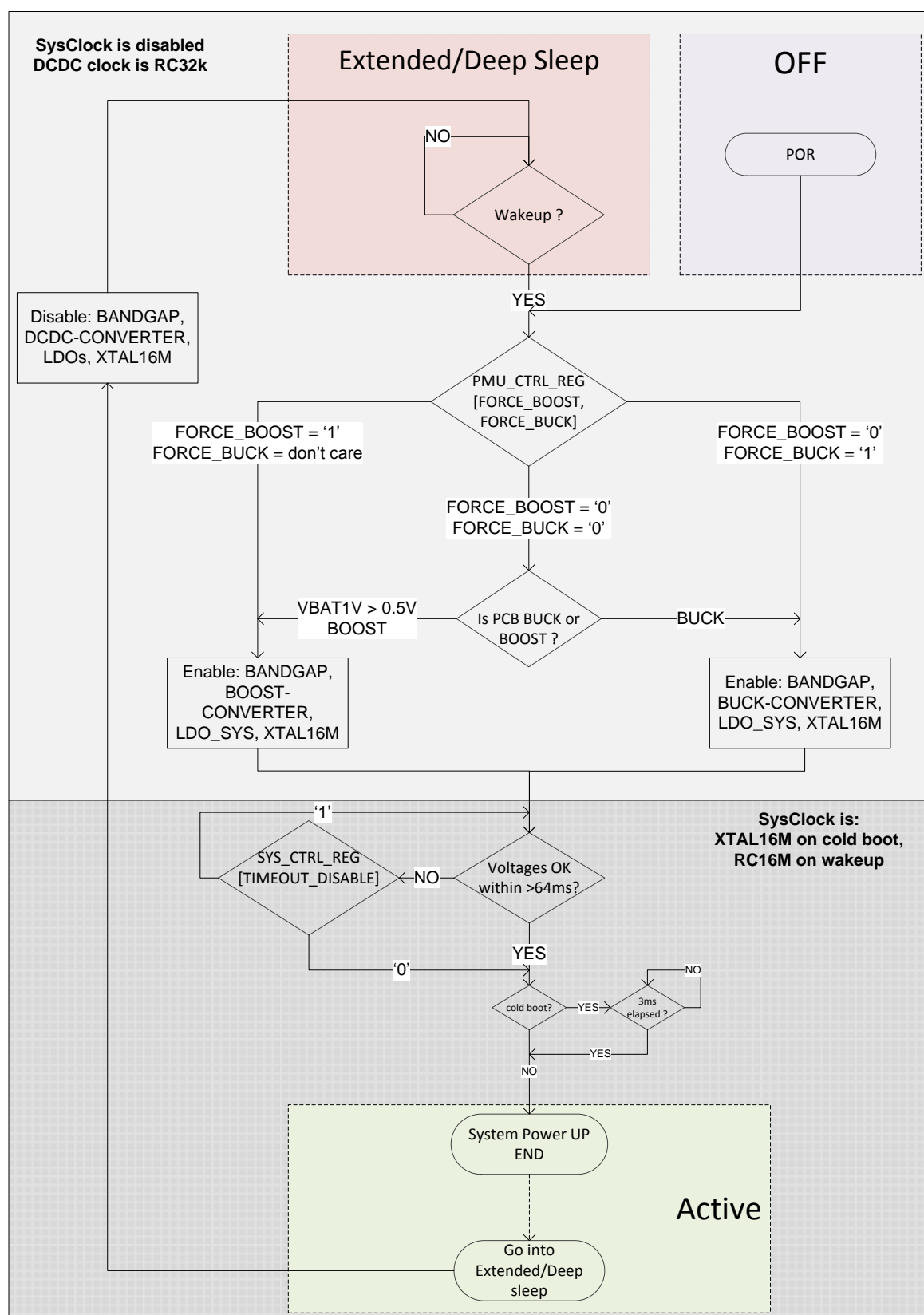
Figure 10: Power/Wake-Up Sequence
