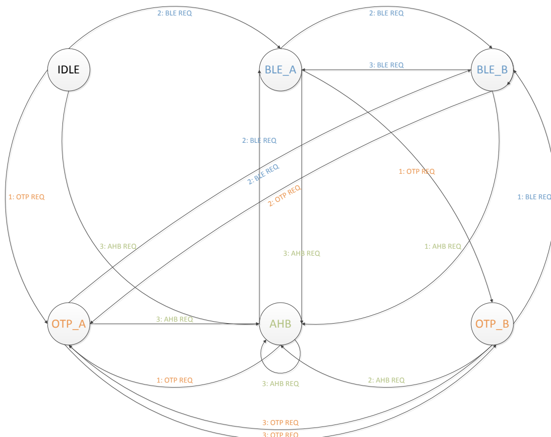
Figure 20: Arbitration Scheme
