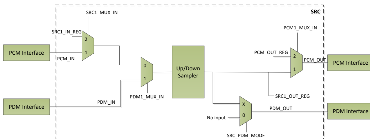
Figure 66: Audio Unit Block Diagram
