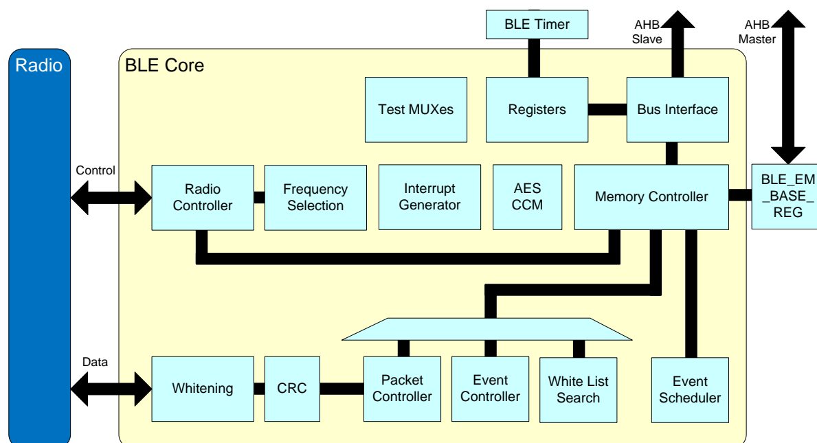
Figure 78: BLE Core Block Diagram
