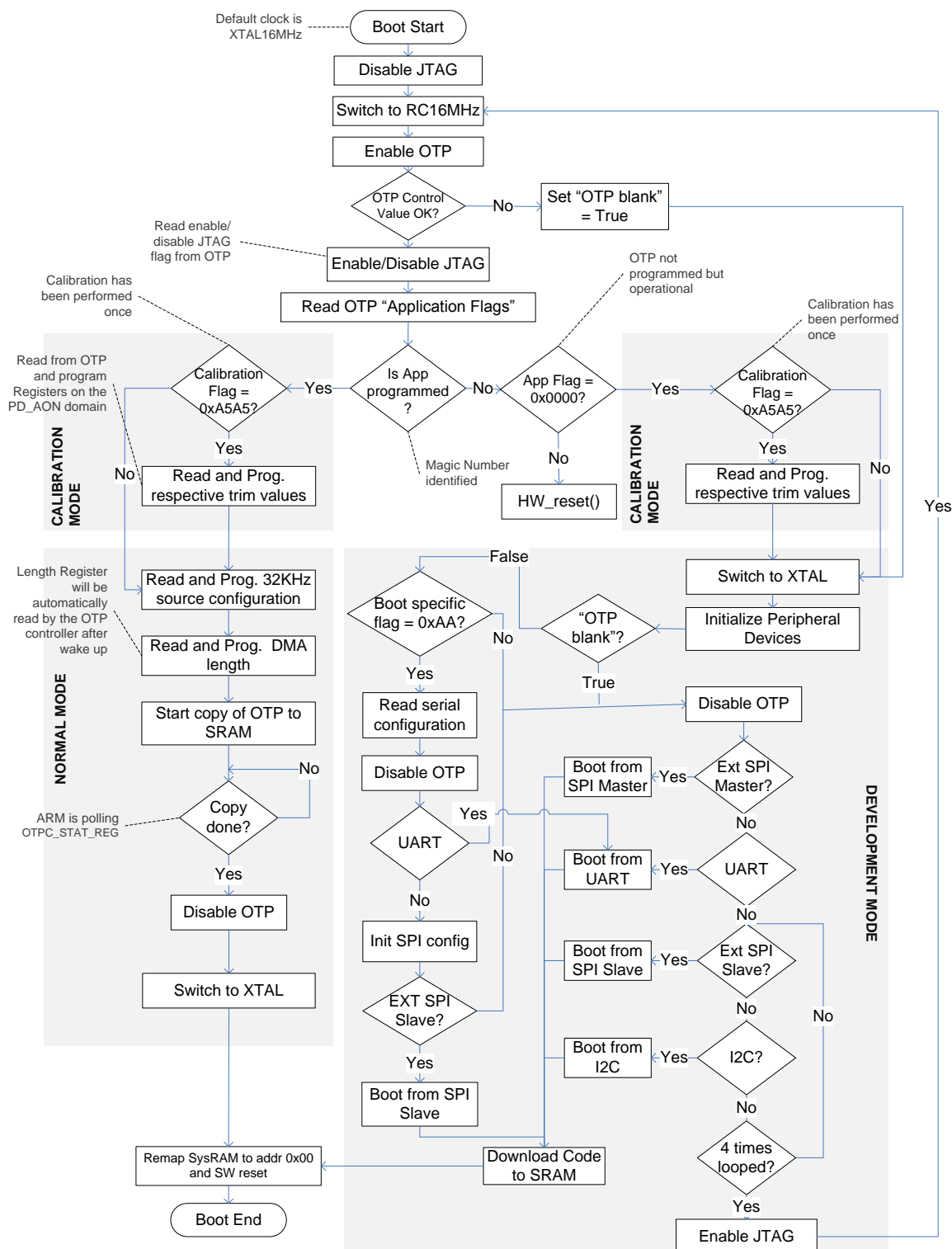
Figure 12: BootROM Sequence
