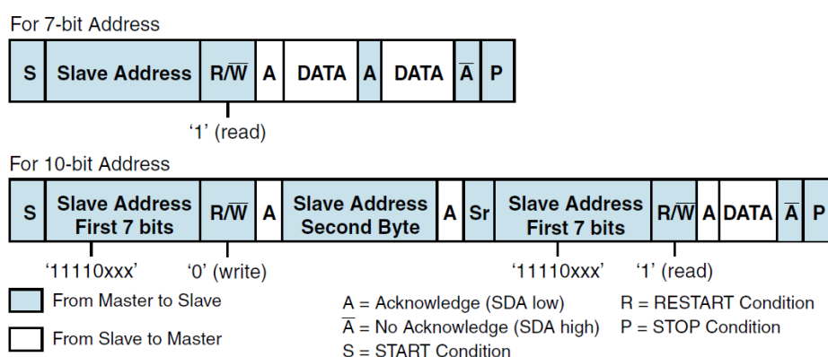
Figure 35: Master-Receiver Protocol
