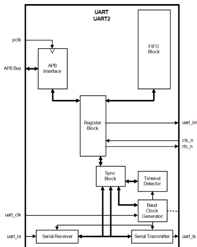
Figure 39: UART Block Diagram
