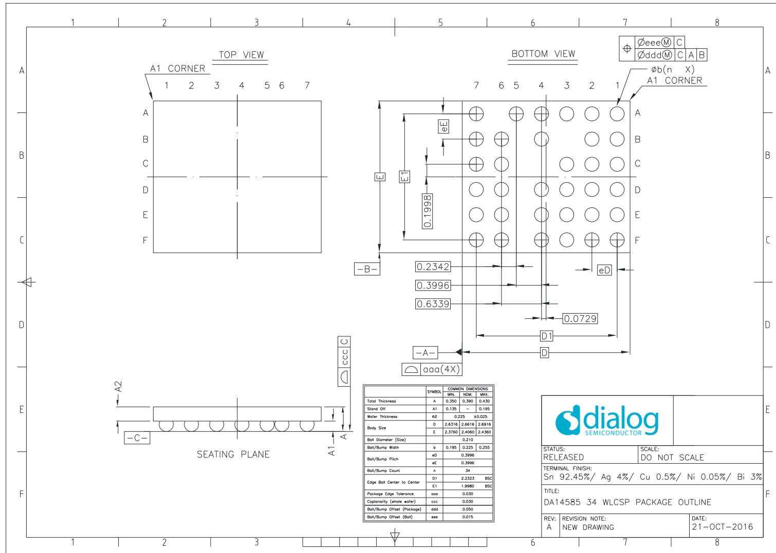
Figure 85: WLCSP34 Package Outline Drawing
