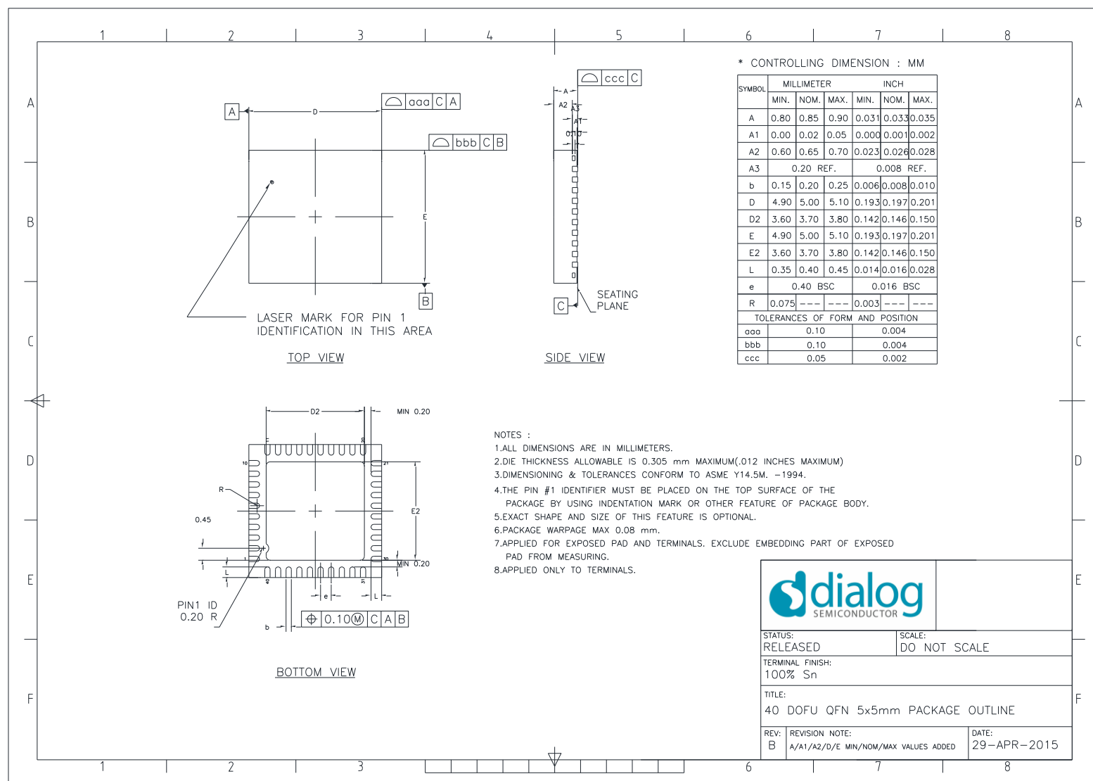
Figure 86: QFN40 Package Outline Drawing
