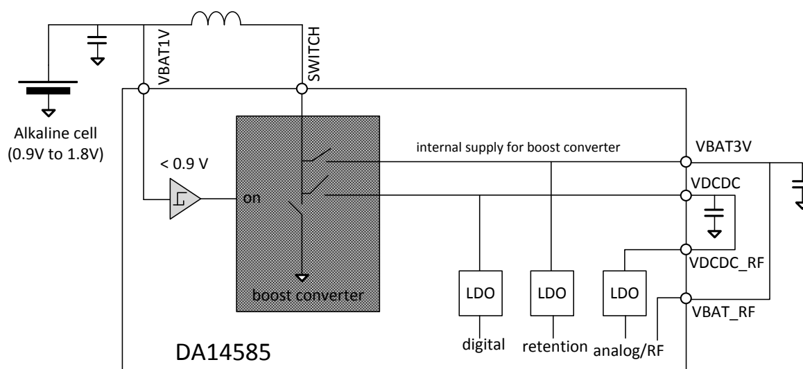
Figure 76: Supply Overview, Alkaline-Cell Application
