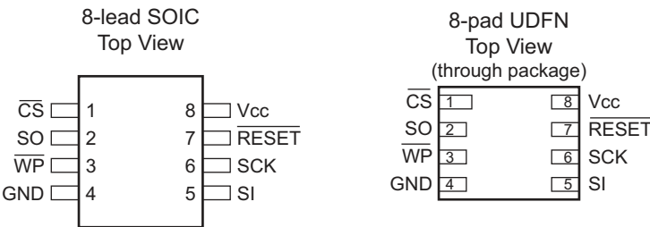
Figure 1-1. Pinouts
