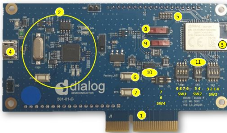
Figure 1: Hardware Configuration
