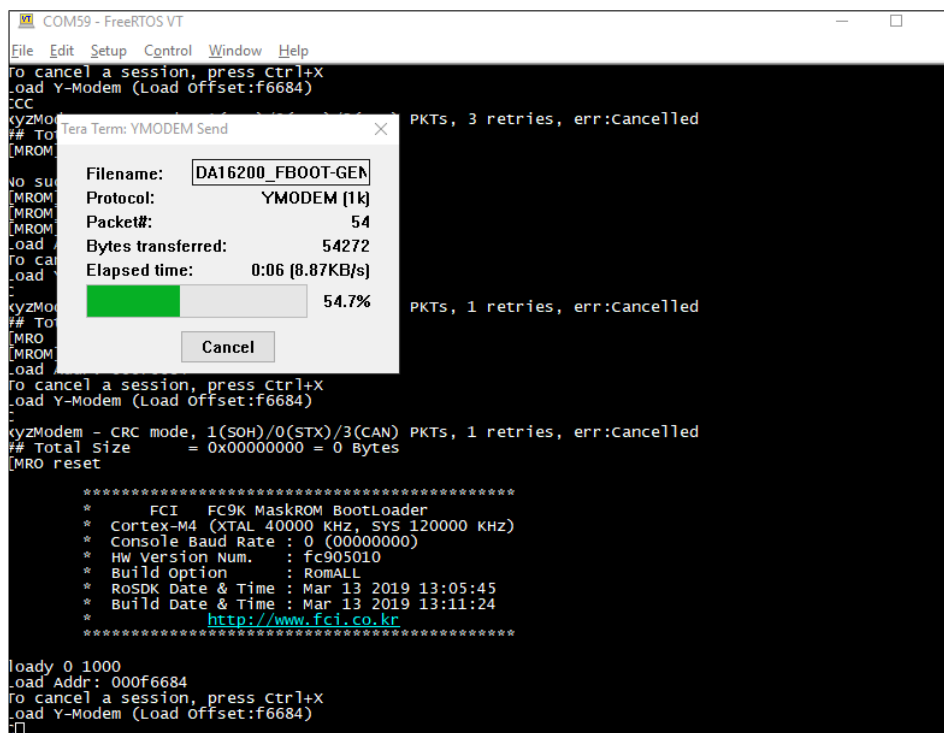
Figure 39: Download Bootloader
