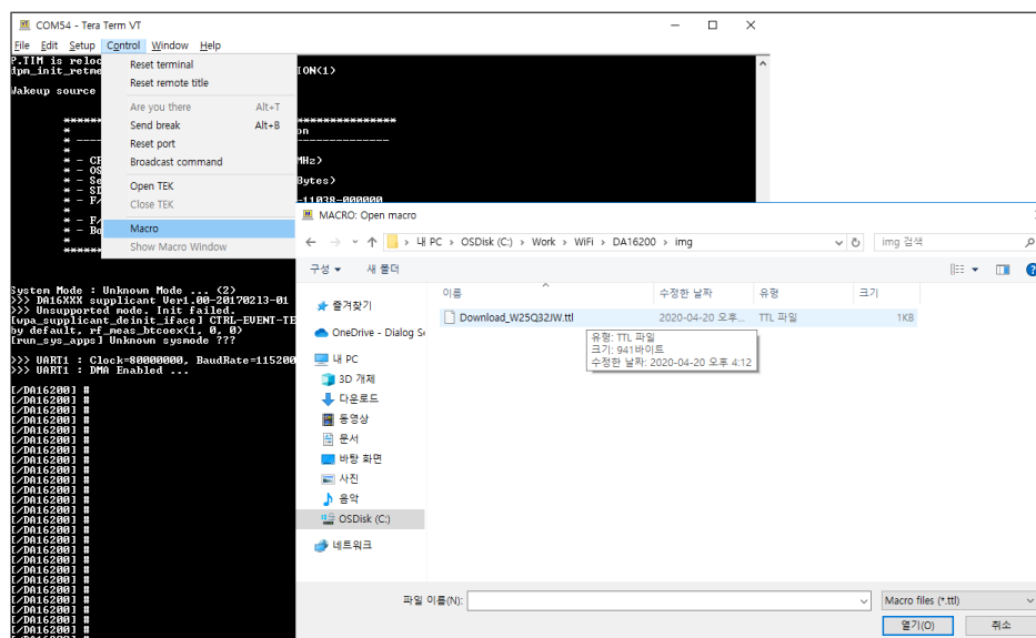
Figure 38: Load Macro
