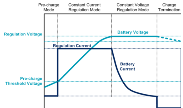
Figure 20: Pre-Charge and Charge Voltage/Current Diagram
