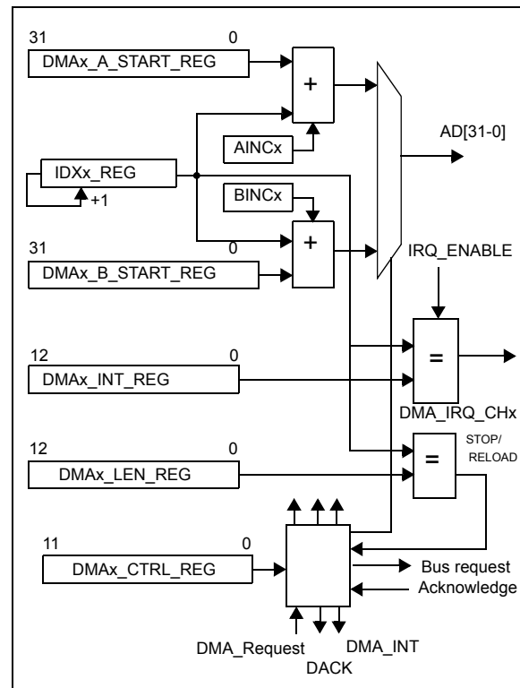
Figure 44: DMA channel diagram
