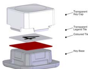
Keypad Assembly
