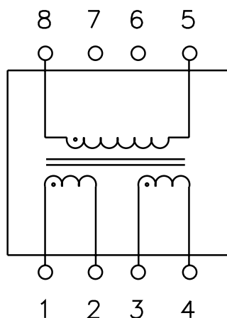
Circuit A
