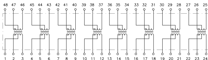
Circuit C
