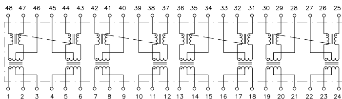
Circuit A
