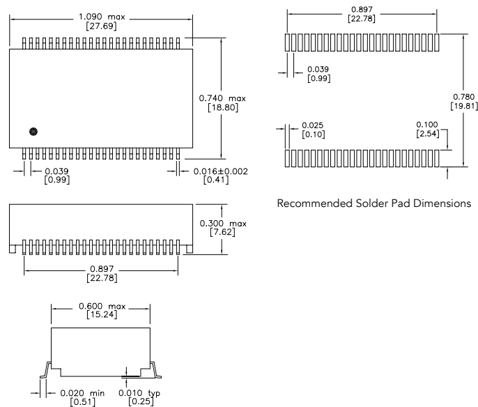
NV Package
