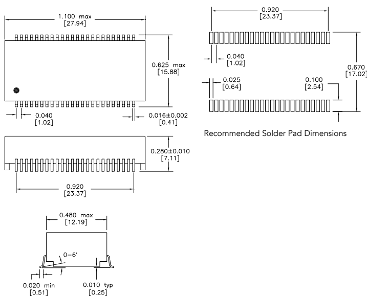
NV6 Package
