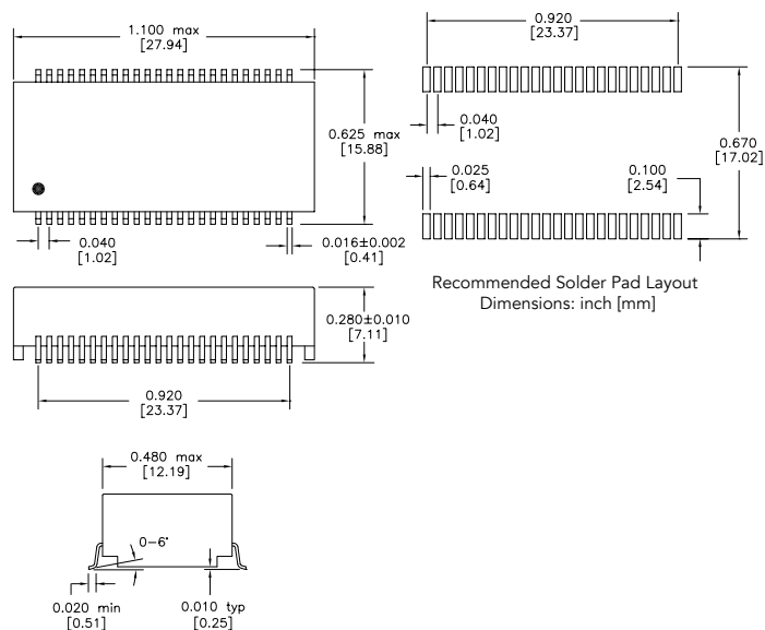
NV6 Package
