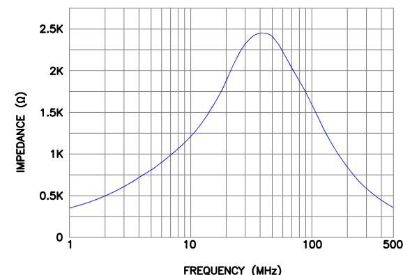
TYPICAL IMPEDANCE CURVE
