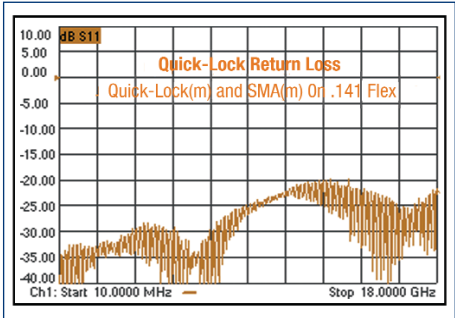
Quick-Lock™ Return Loss
