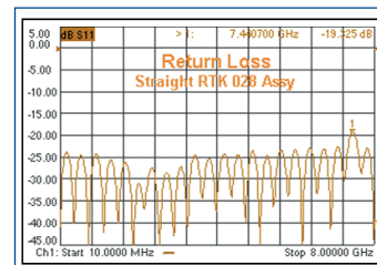
Return Loss-Straight RTK-028
