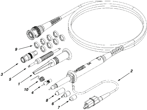
Figure 1: Accessory Diagram
