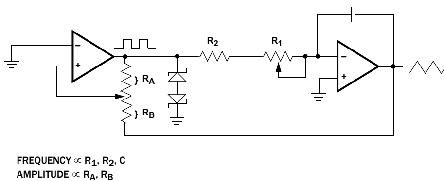
FIGURE 22. FUNCTION GENERATOR
