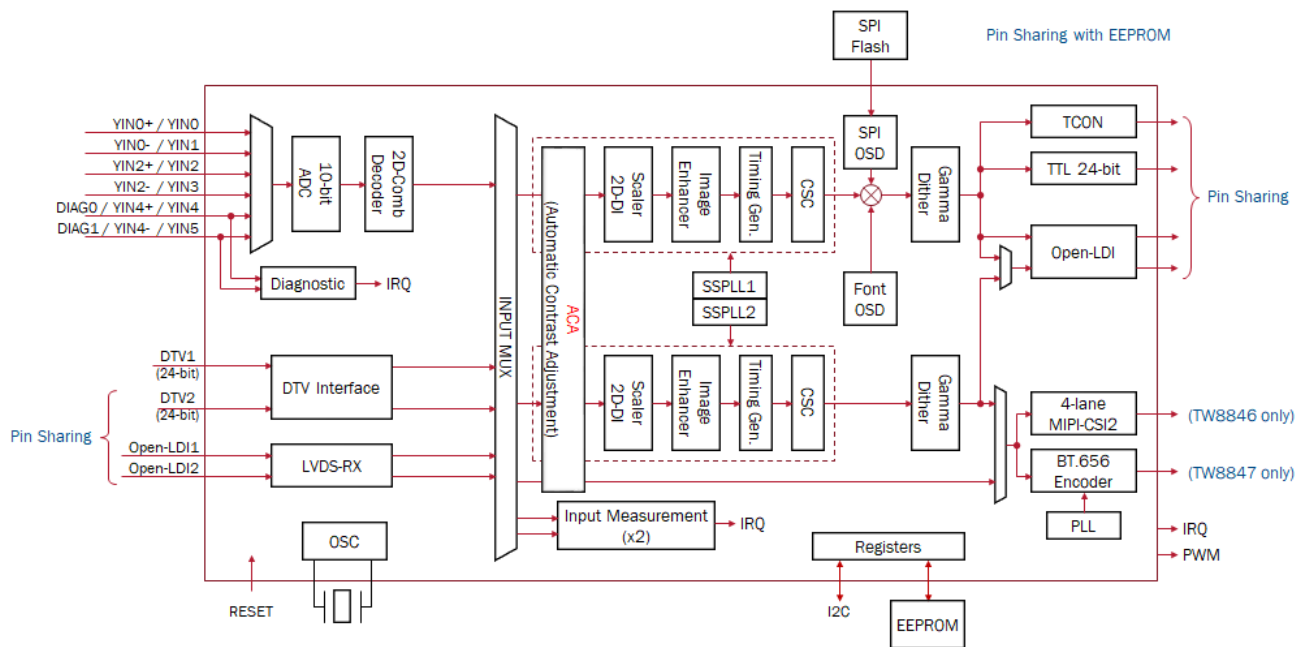
Figure 1. TW8846, TW8847 Functional Block Diagram
