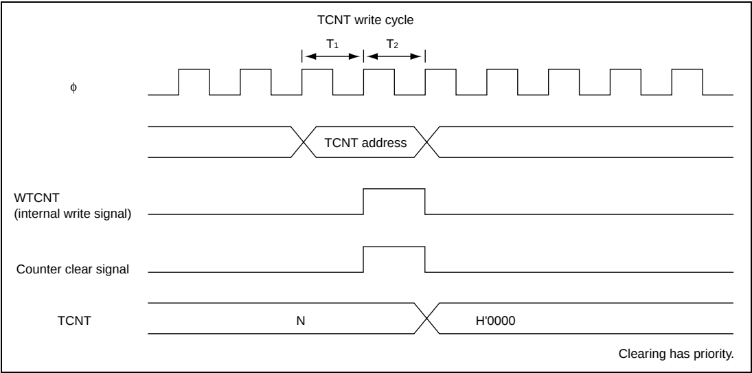
Figure 13.52 Contention between TCNT Write and Clear Operations
