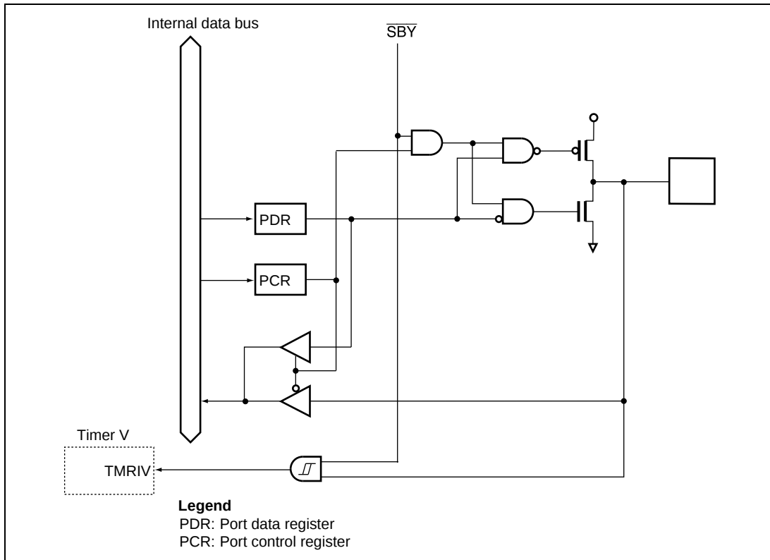
Figure B.17 Port 7 Block Diagram (P74)
