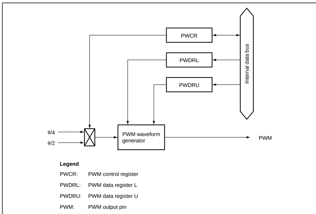
Figure 15.1 Block Diagram of 14-Bit PWM
