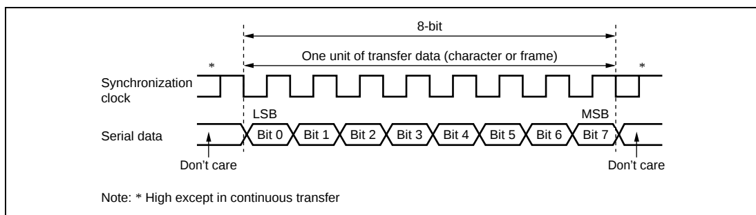
Figure 16.9 Data Format in Clocked Synchronous Communication
