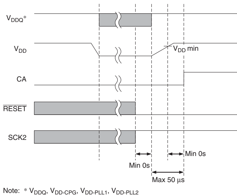
Figure 9.14 Timing When Power Other than VDD-RTC Is Off
