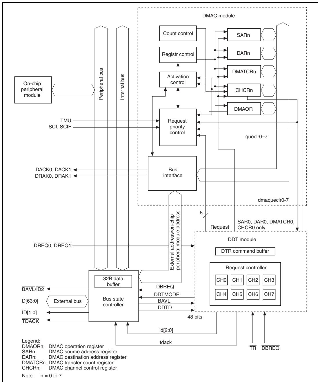
Figure 14.53 Block Diagram of the DMAC
