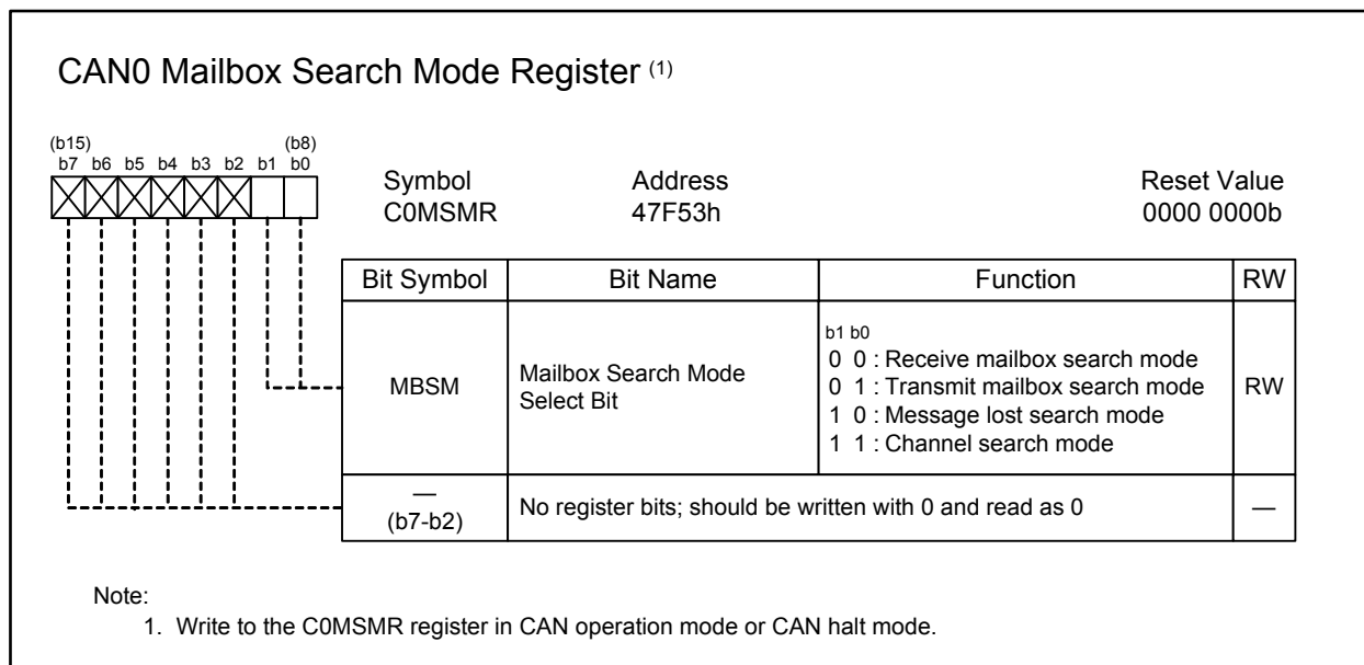
Figure 25.18 C0MSMR Register
