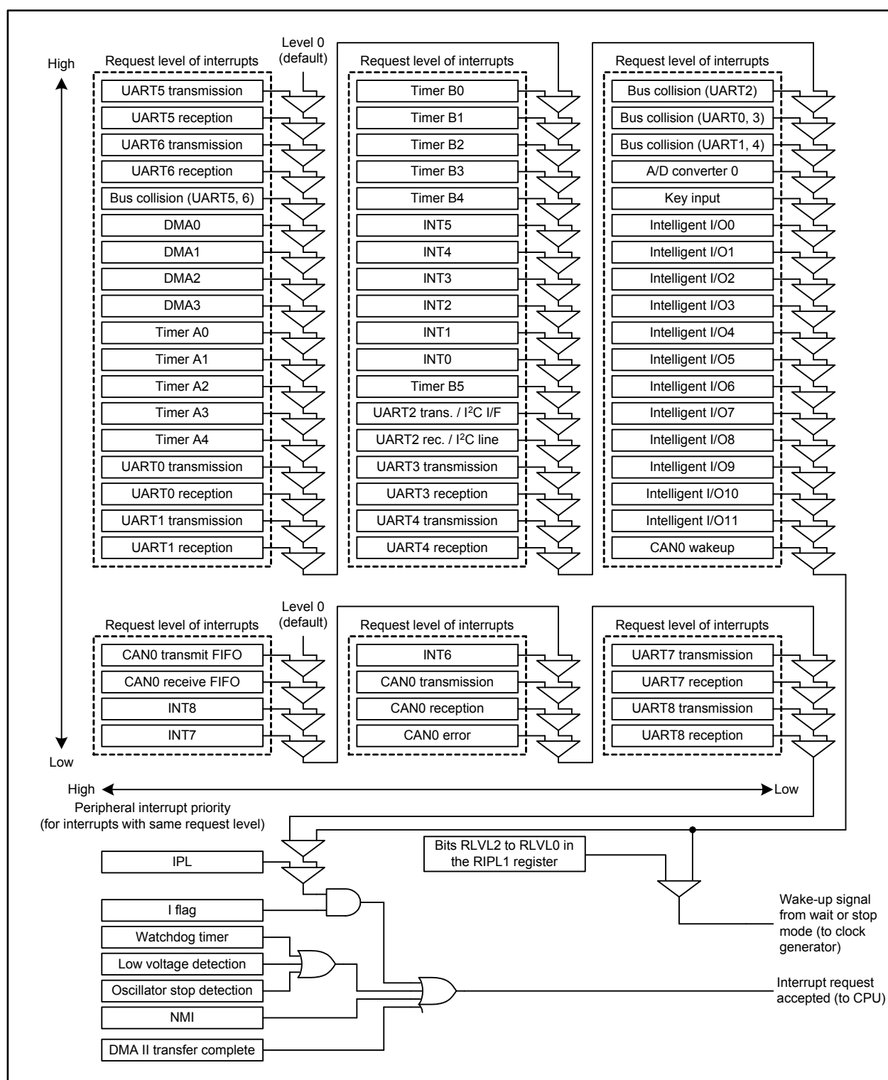
Figure 11.8 Priority Resolver
