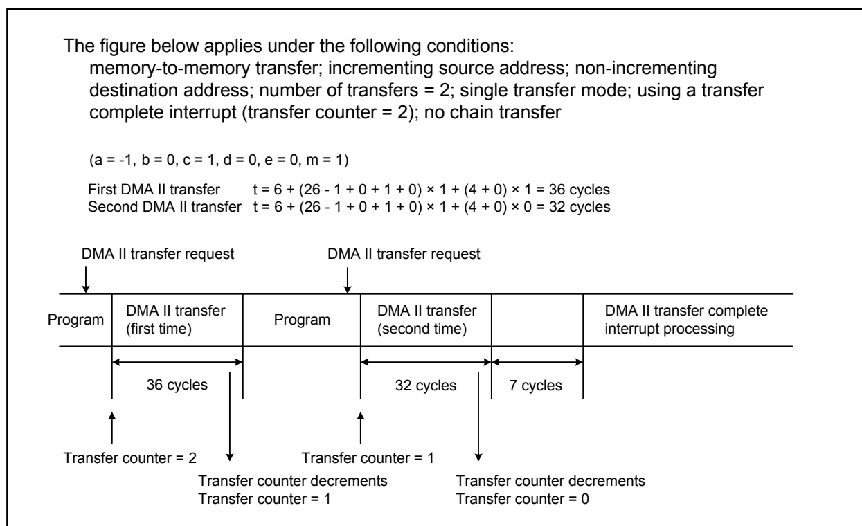
Figure 14.5 Transfer Cycles
