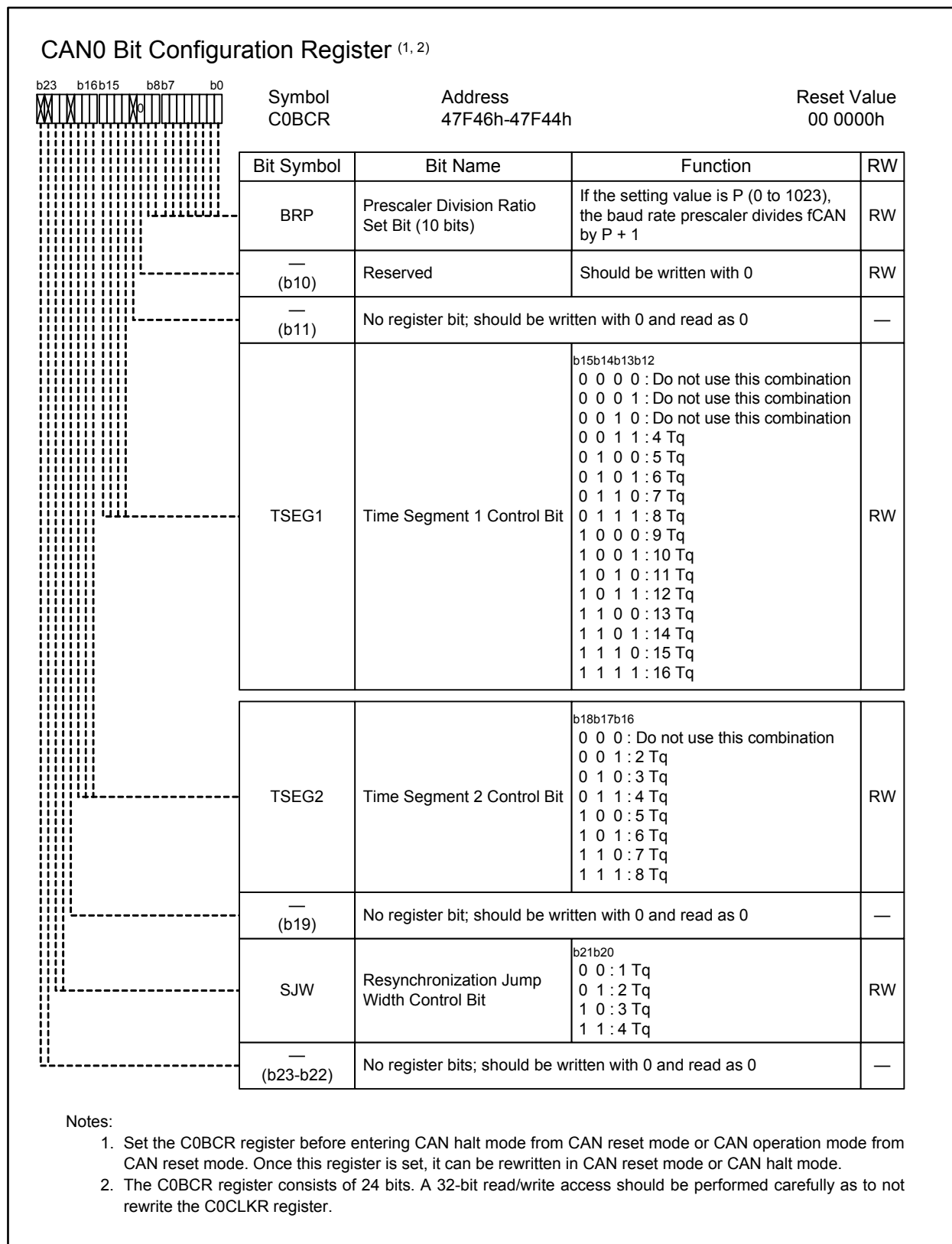
Figure 25.4 C0BCR Register
