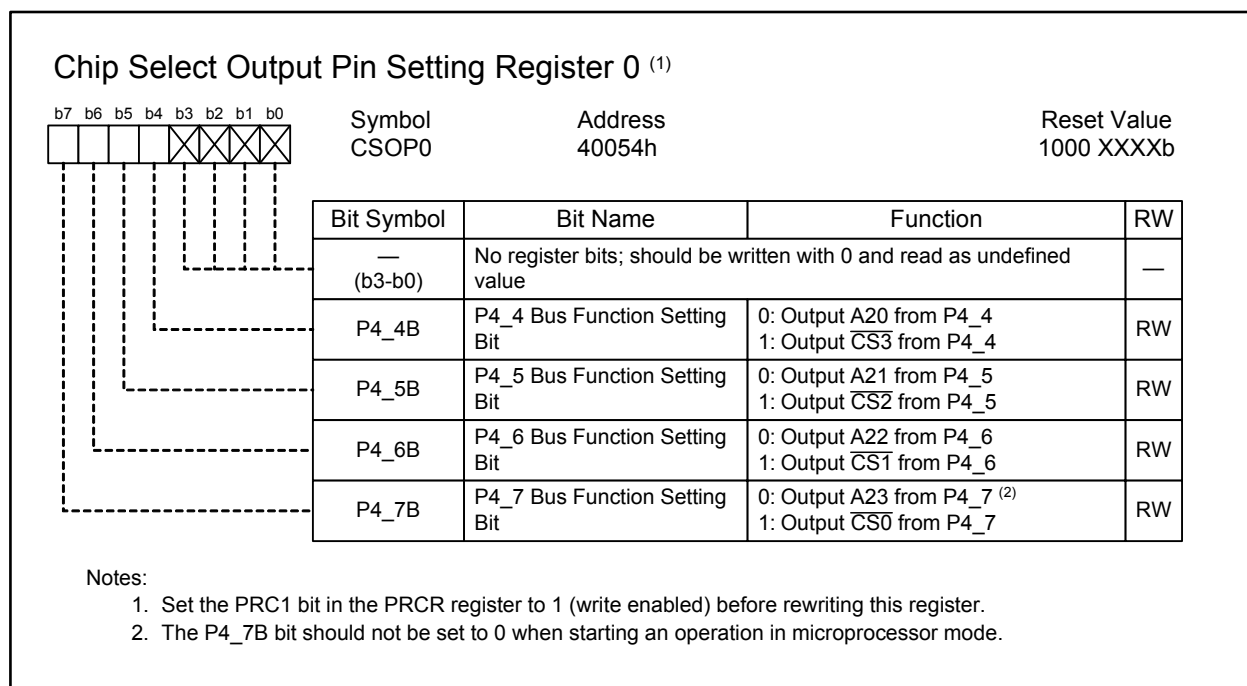
Figure 9.4 CSOP0 Register
