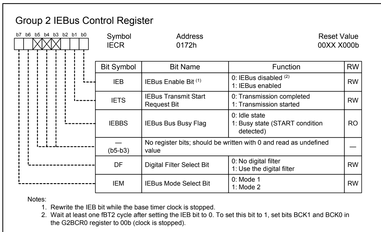
Figure 23.37 IECR Register
