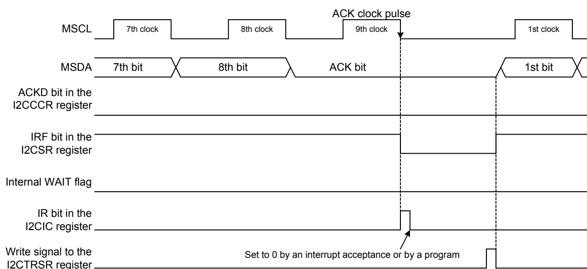
(B) When the RIE bit is 1 (receive mode, ACK clock generated)
