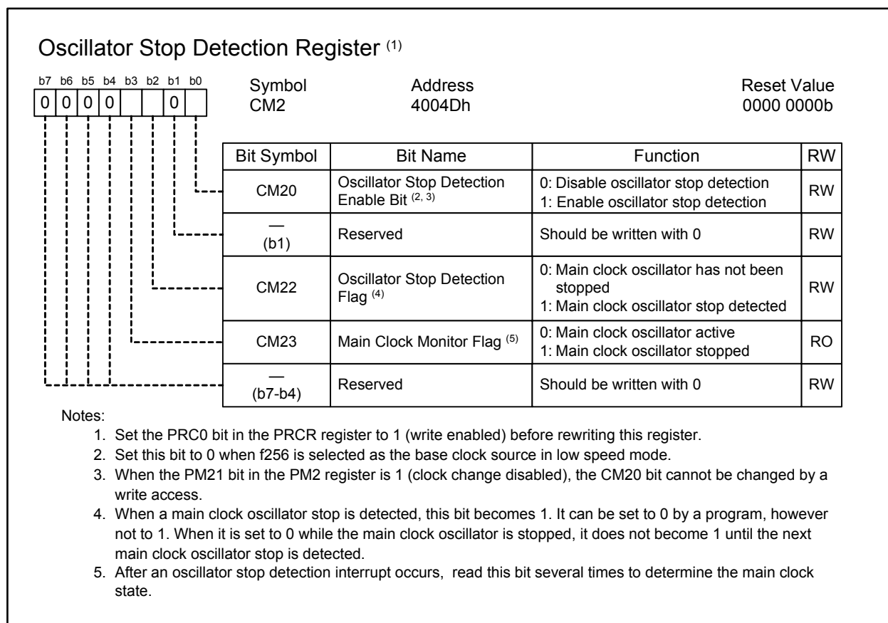
Figure 8.5 CM2 Register
