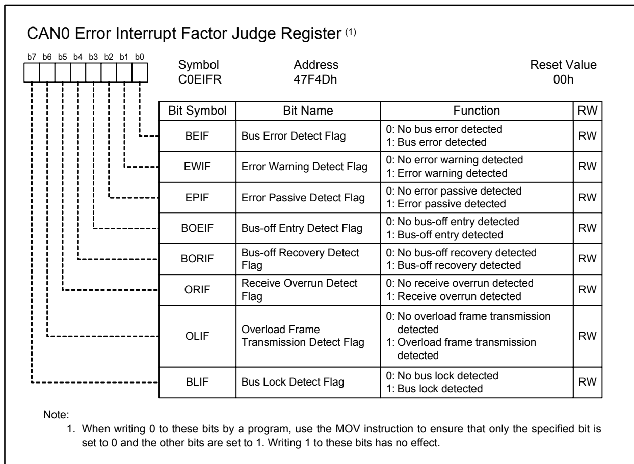
Figure 25.25 C0EIFR Register
