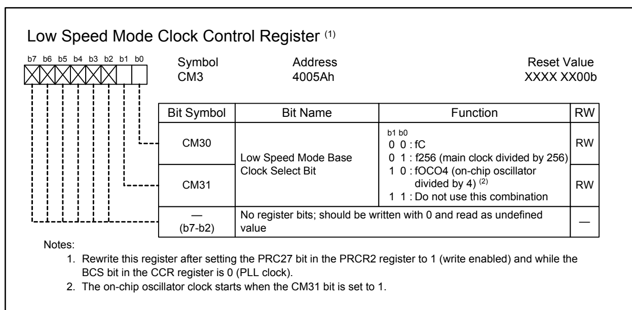
Figure 8.6 CM3 Register
