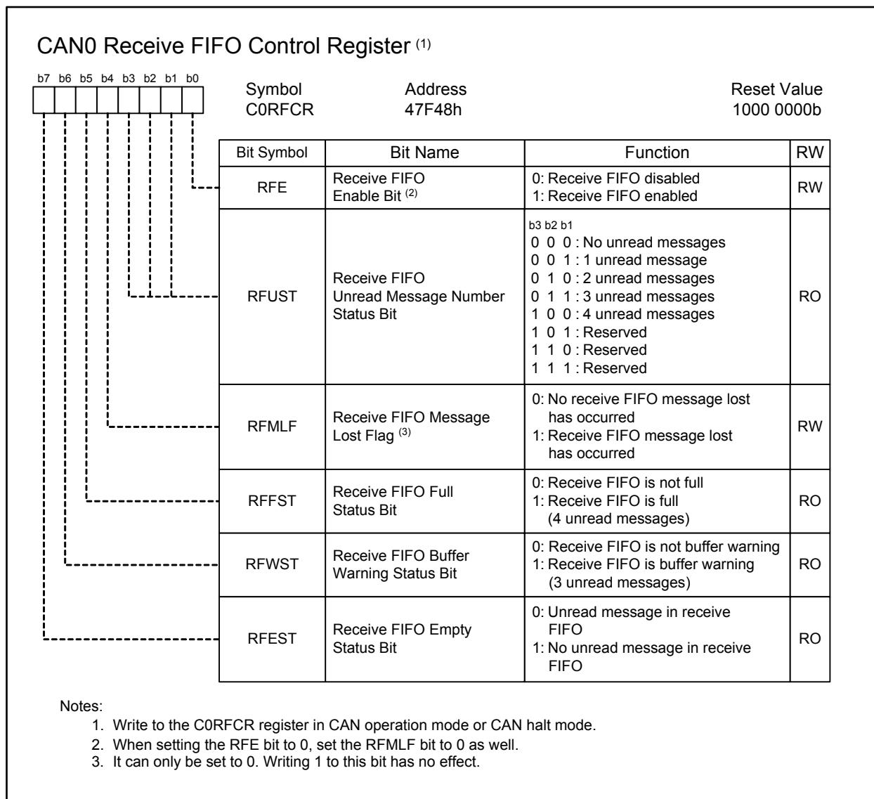
Figure 25.11 C0RFCR Register
