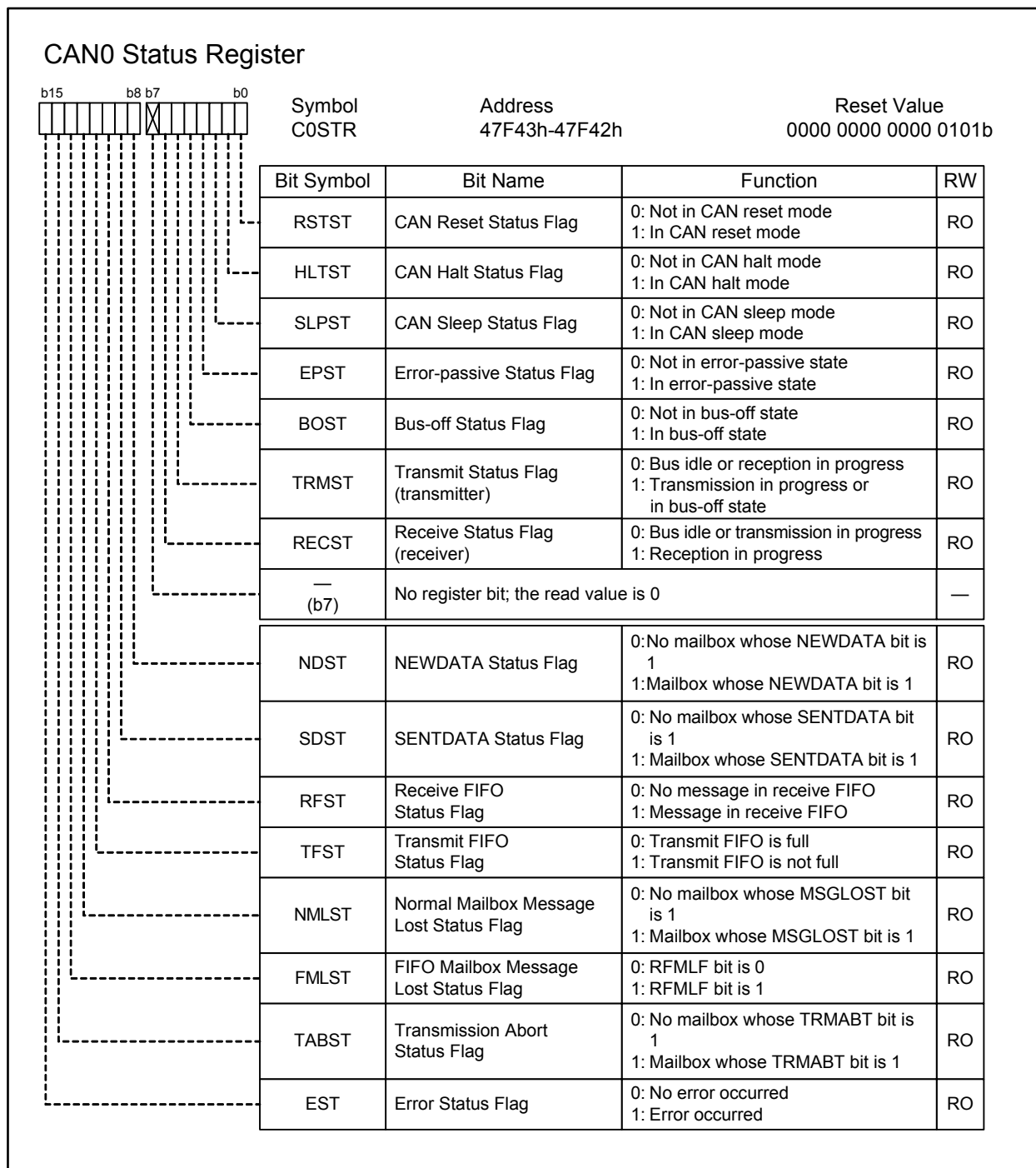
Figure 25.17 C0STR Register
