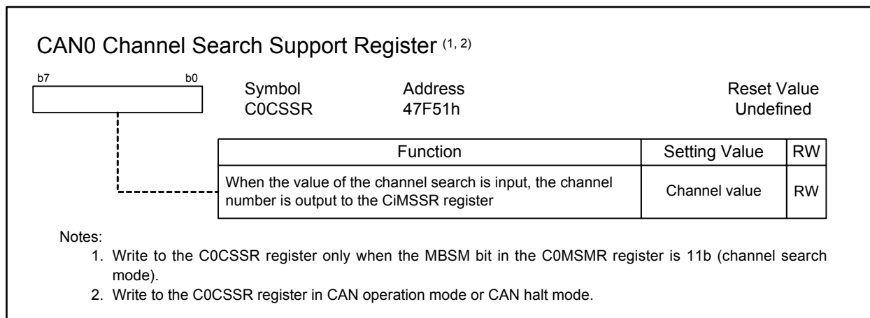
Figure 25.20 C0CSSR Register
