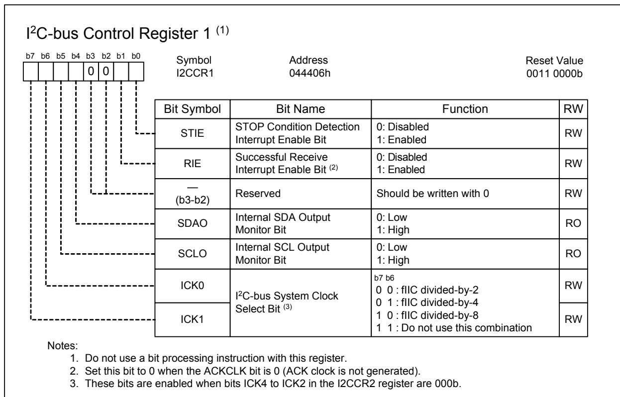
Figure 24.9 I2CCR1 Register
