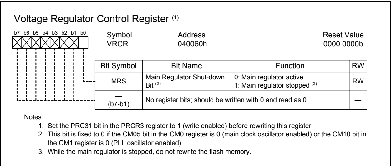
Figure 6.2 VRCR Register
