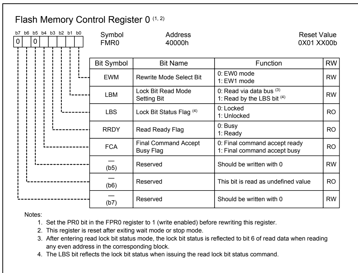
Figure 27.7 FMR0 Register
