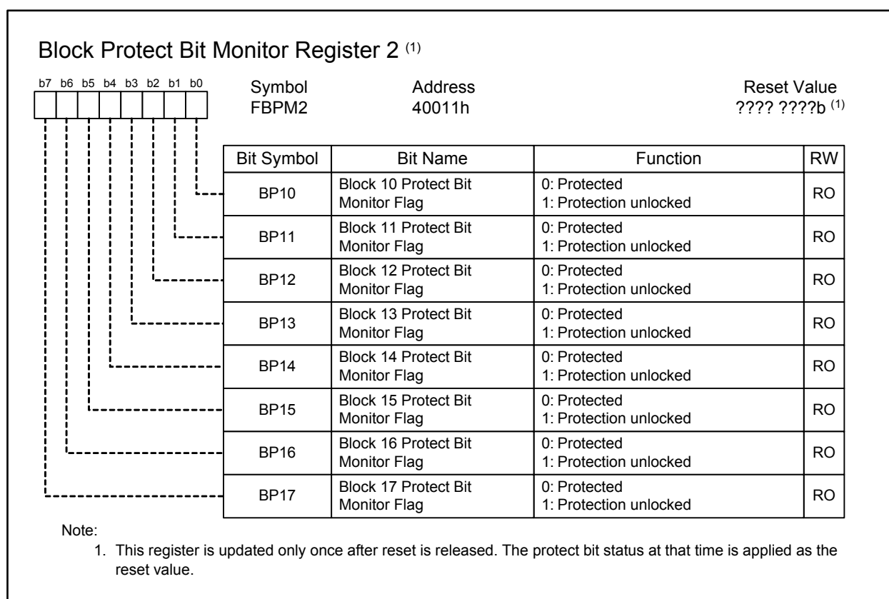
Figure 27.12 FBPM2 Register
