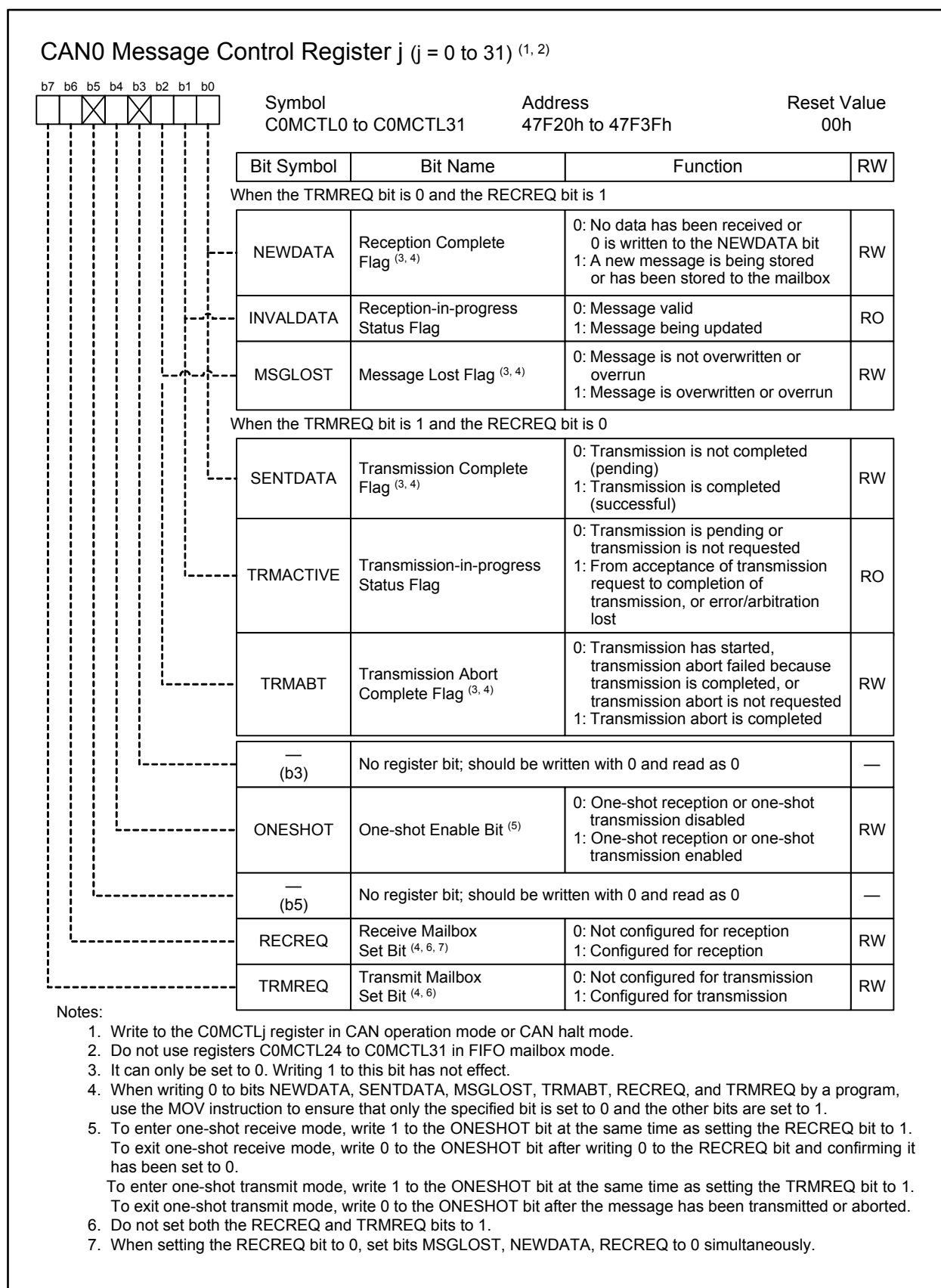
Figure 25.10 C0MCTLj Register
