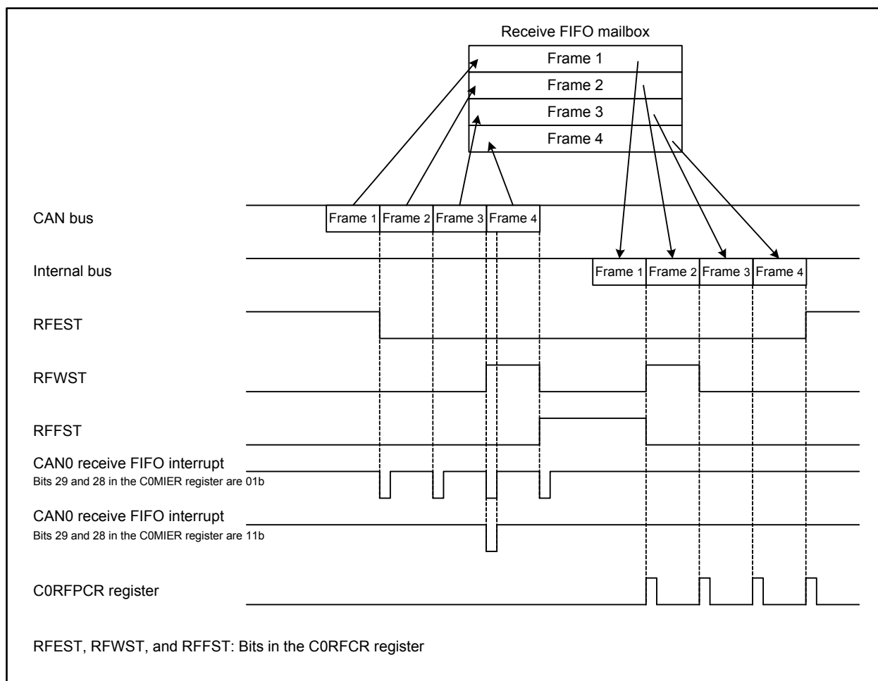
Figure 25.12 Receive FIFO Mailbox Operation (Bits 29 and 28 in C0MIER Register are 01b and 11b)
