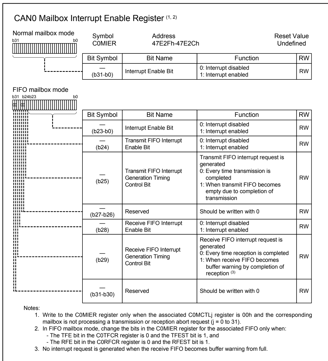
Figure 25.9 C0MIER Register
