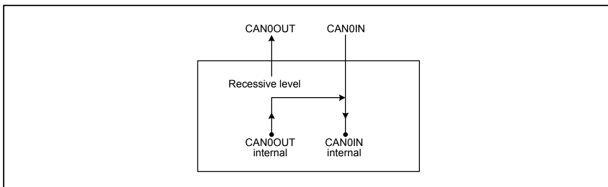
Figure 25.31 Connection when Listen Only Mode is Selected
