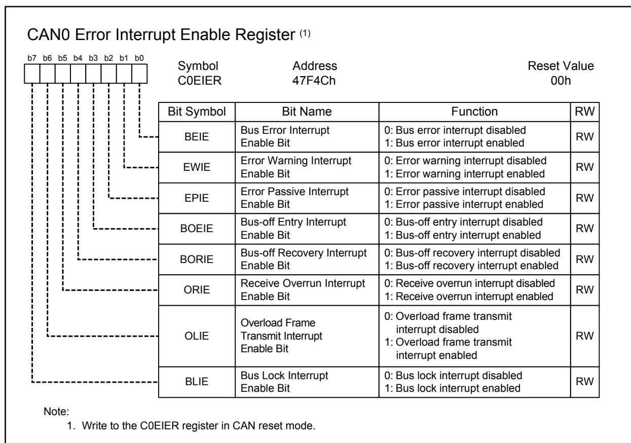
Figure 25.24 C0EIER Register
