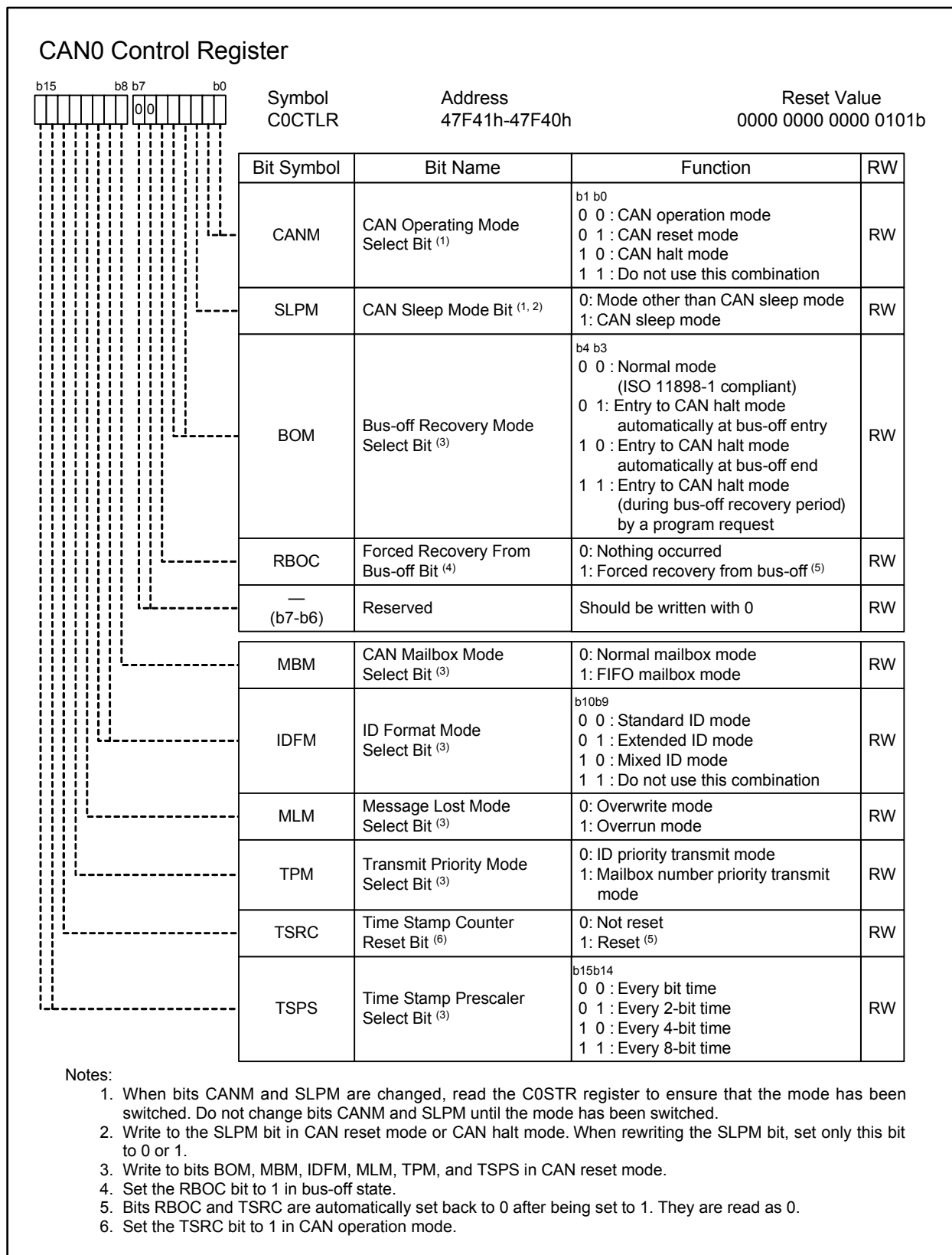
Figure 25.2 C0CTLR Register
