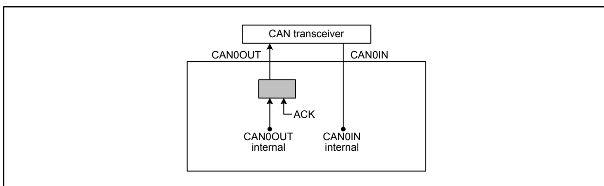
Figure 25.32 Connection when Self Test Mode 0 is Selected
