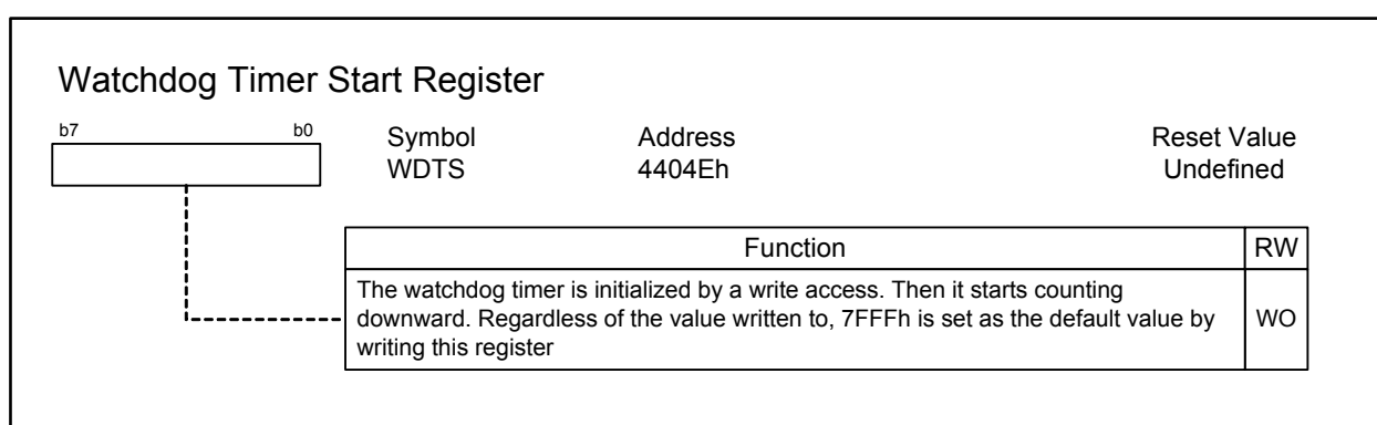
Figure 12.3 WDTS Register
