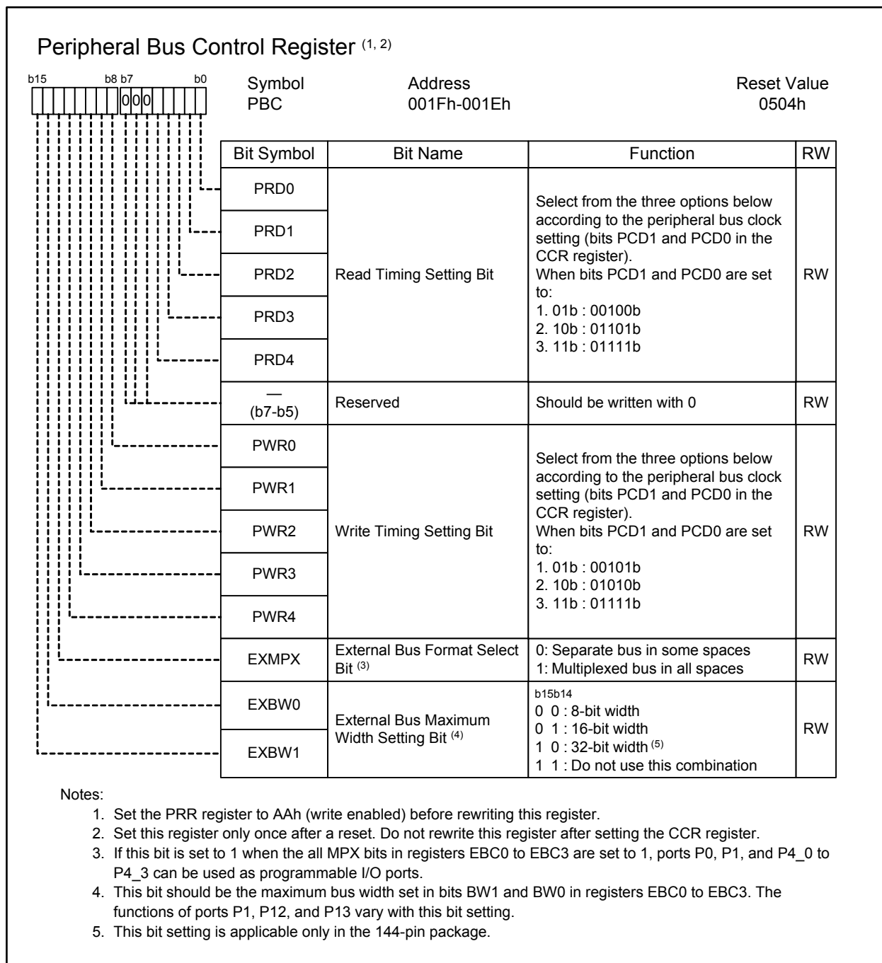
Figure 9.2 PBC Register
