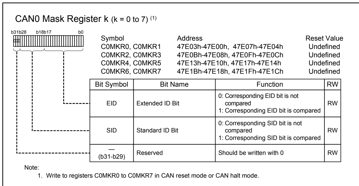
Figure 25.5 Registers C0MKR0 to C0MKR7
