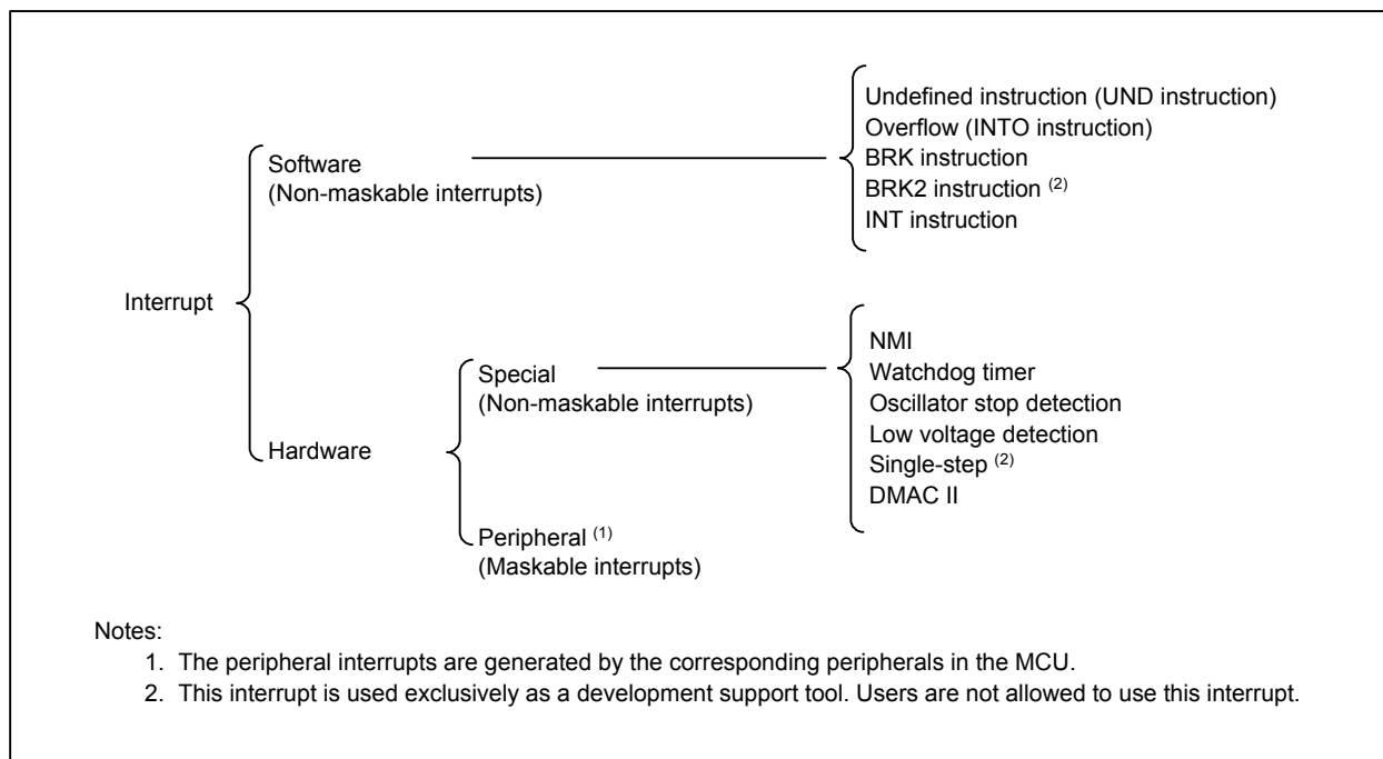
Figure 11.1 Interrupts
