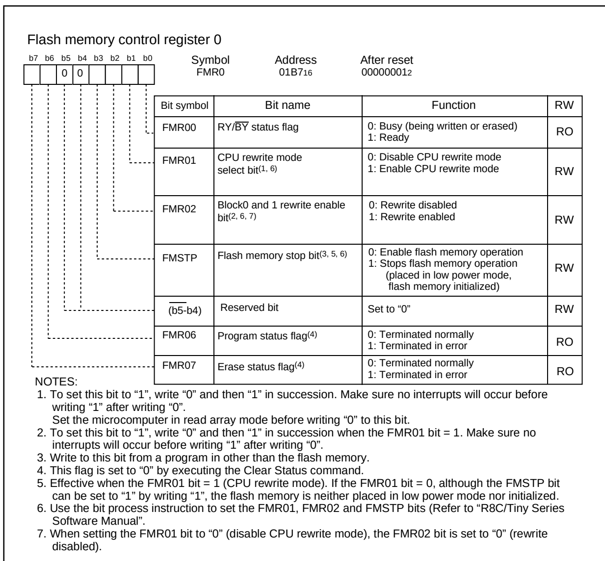
Figure 17.3 FMR0 Register
