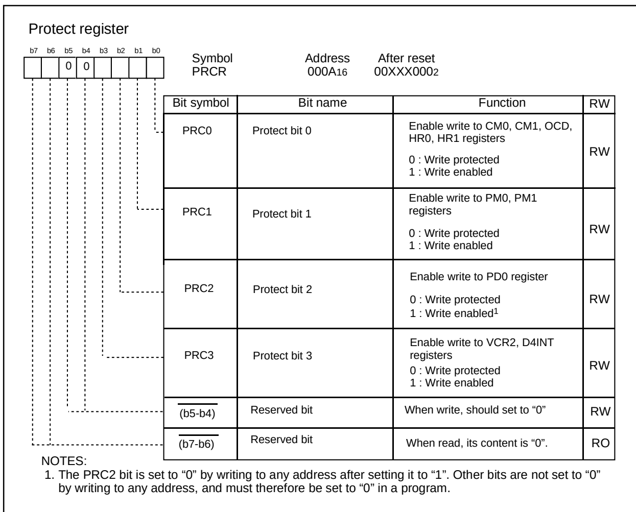
Figure 7.1 PRCR Register
