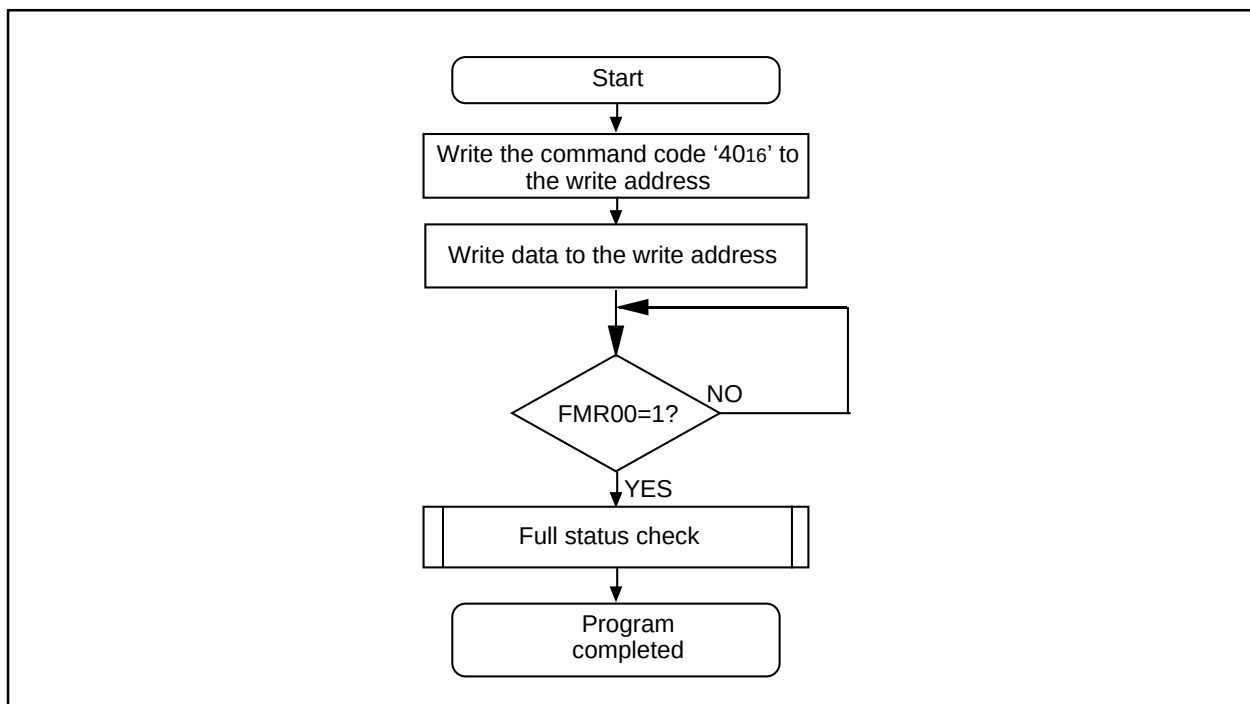
Figure 17.9 Program Command
