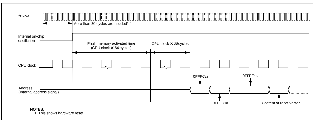
Figure 5.2 Reset Sequence
