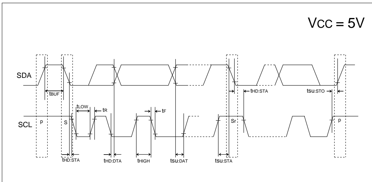
Figure 19.4 Timing Diagram (3)
