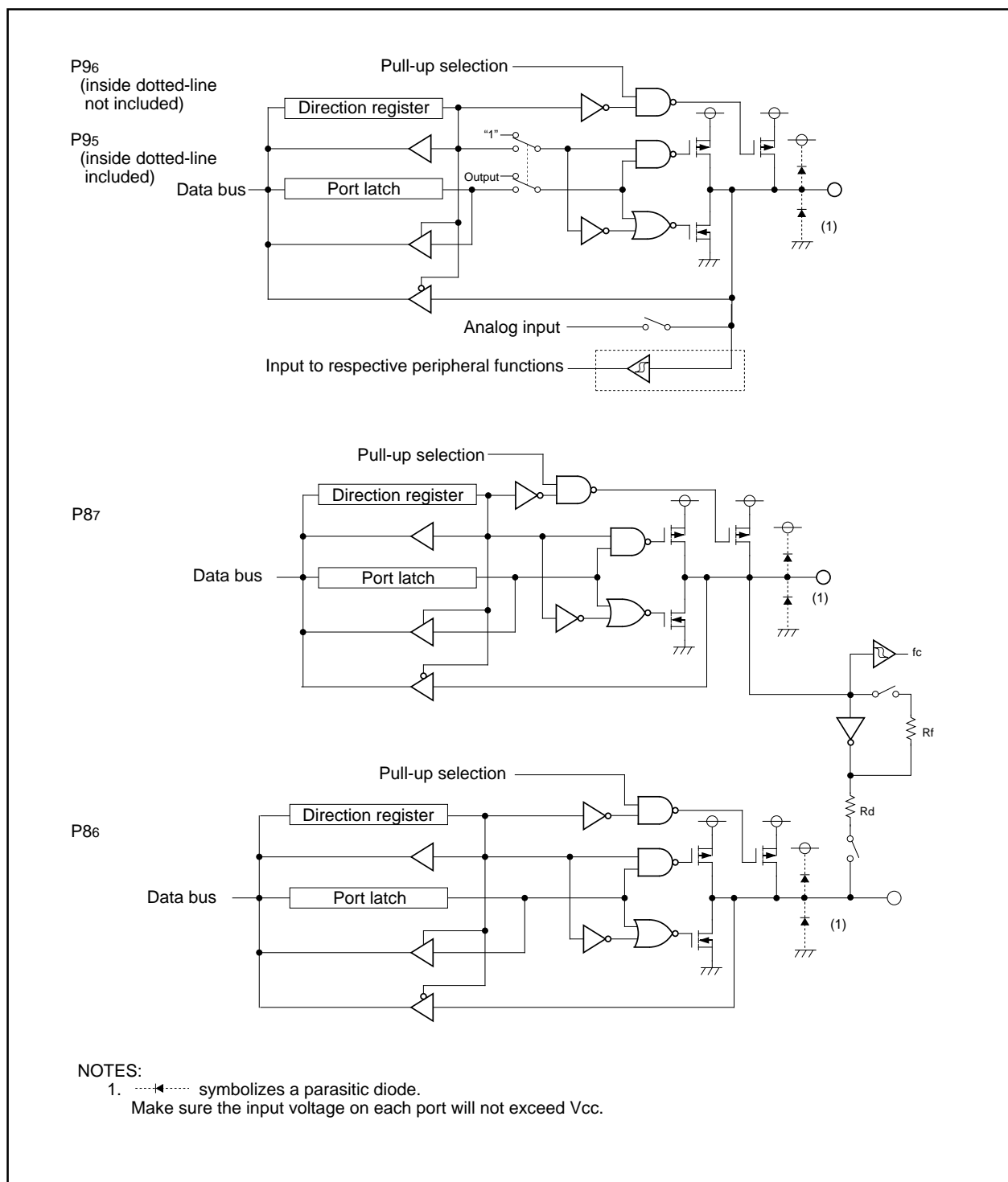
Figure 17.4 I/O Ports (4)
