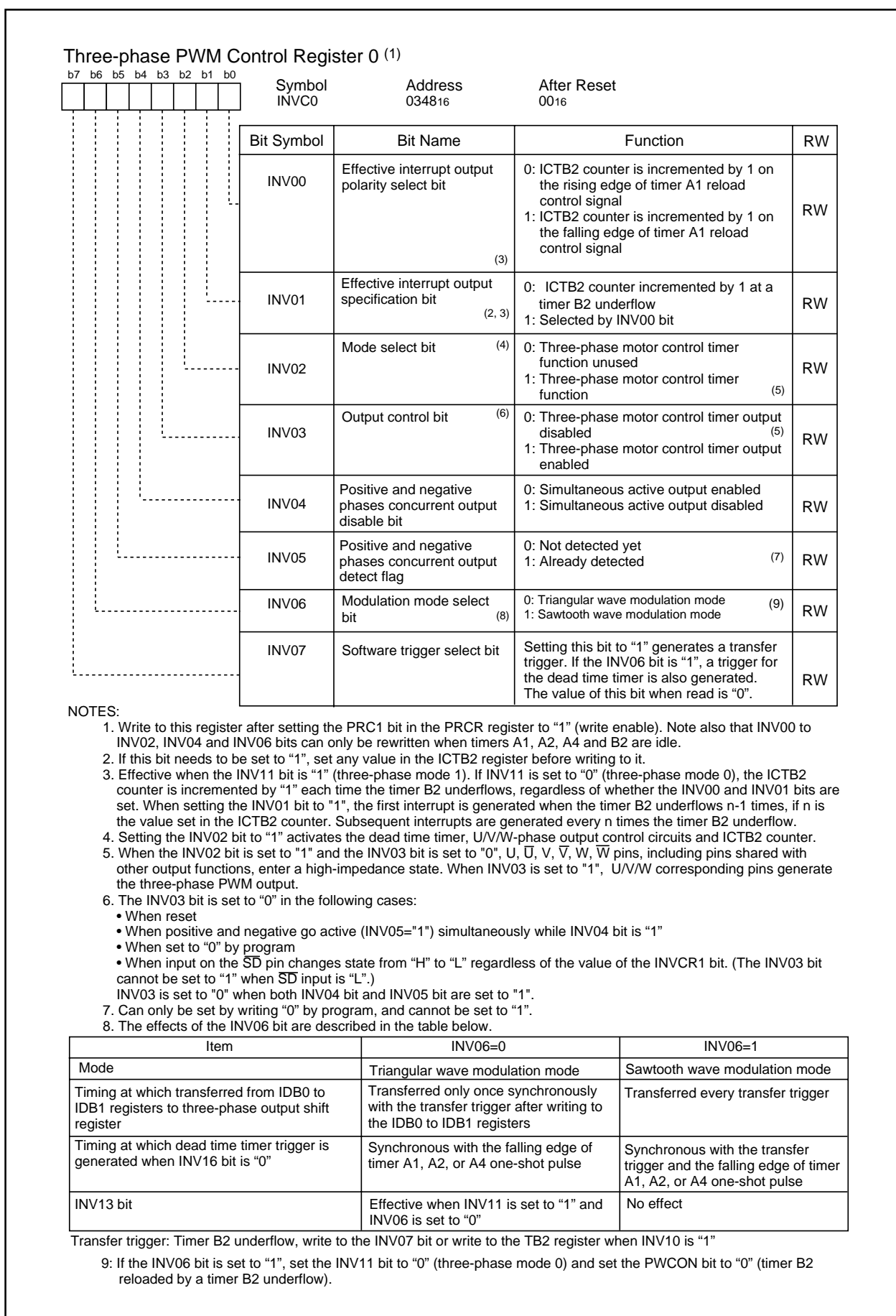
Figure 12.26 INV0 Register
