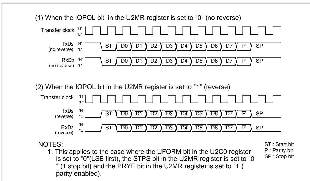
Figure 14.20 TxD and RxD I/O Polarity Inverse
