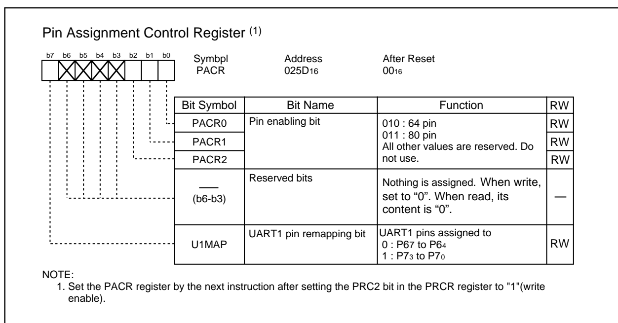
Figure 17.10 PACR Register
