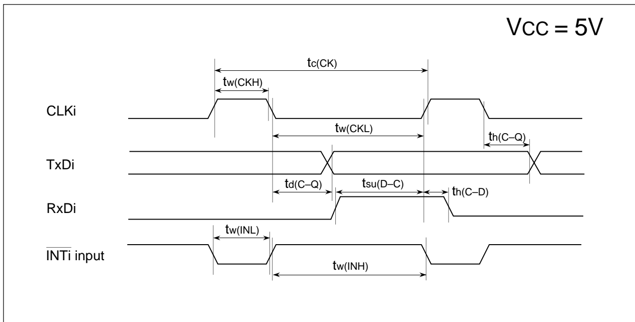
Figure 19.3. Timing Diagram (2)
