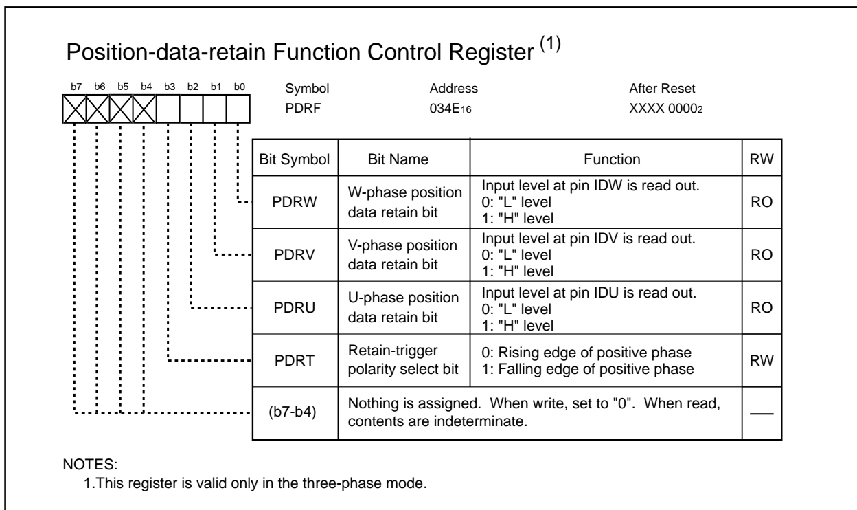
Figure 12.36 PDRF Register
