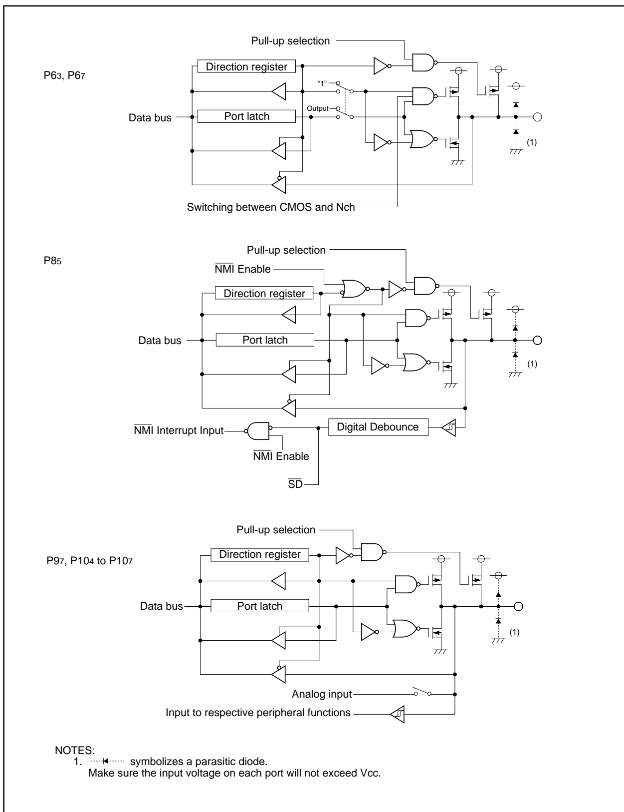
Figure 17.3 I/O Ports (3)
