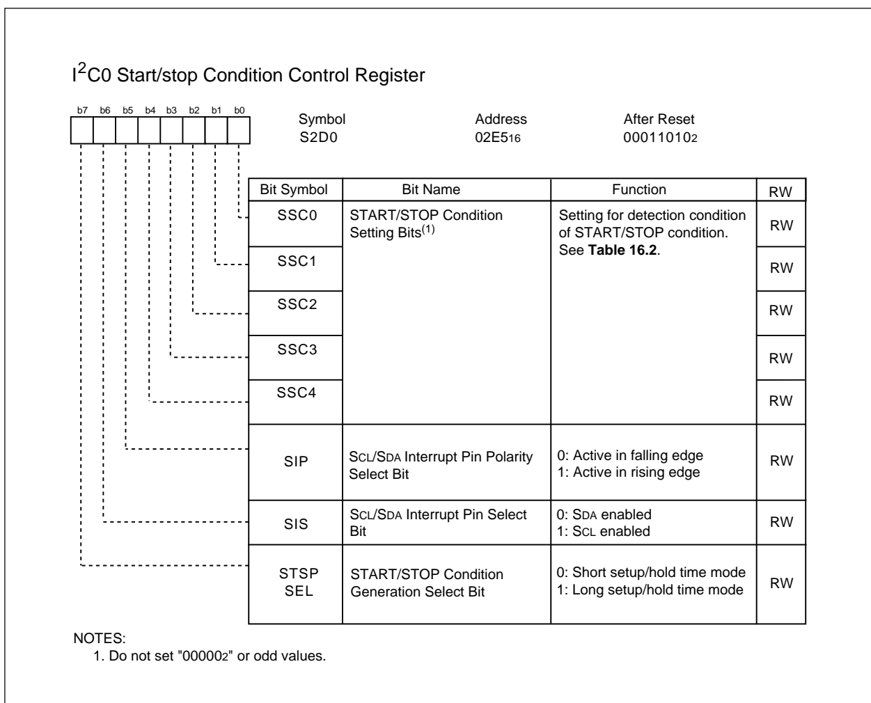
Figure 16.8 S2D0 Register
