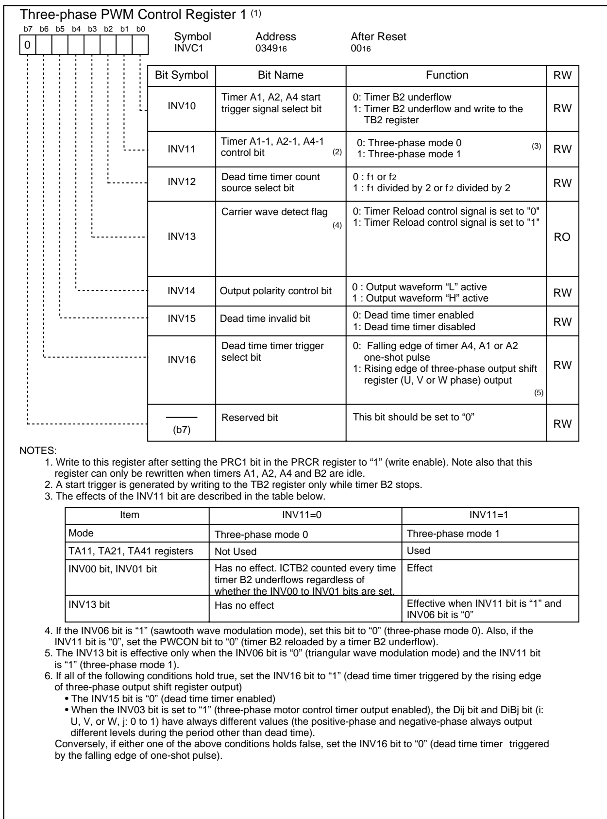
Figure 12.27 INVC1 Register
