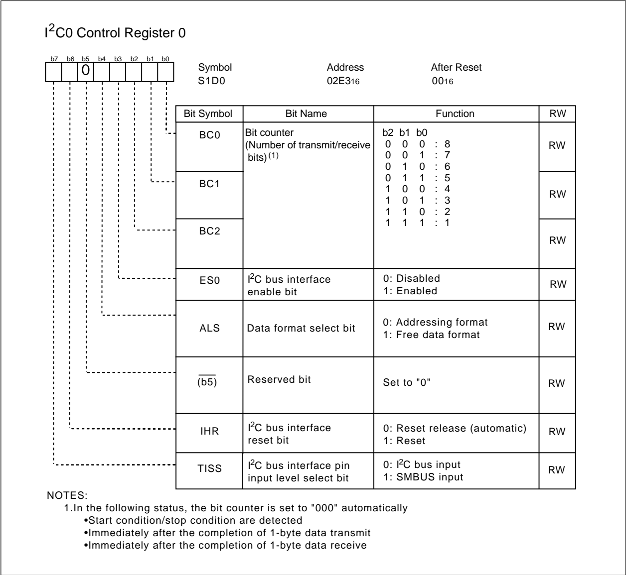
Figure 16.4 S1D0 Register
