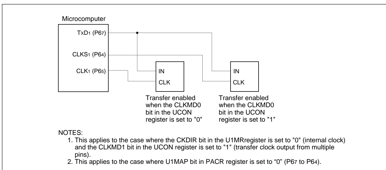
Figure 14.14 Transfer Clock Output From Multiple Pins
