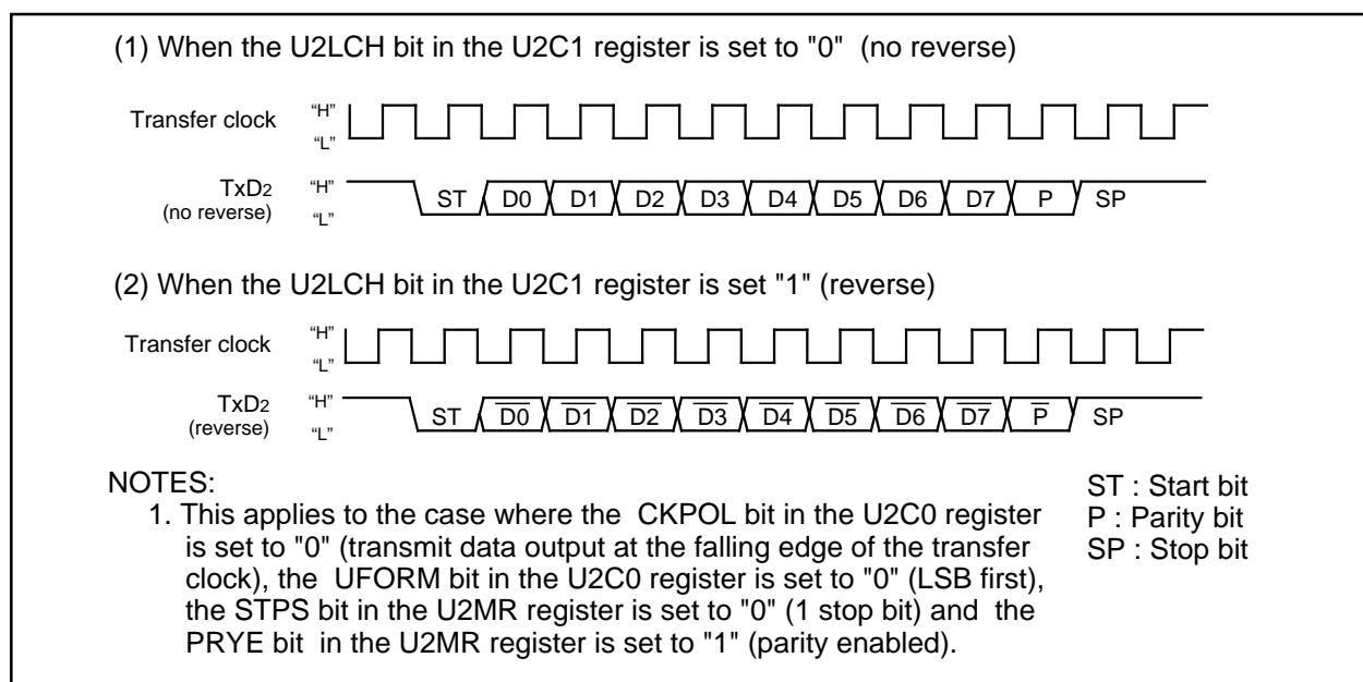
Figure 14.19 Serial Data Logic Switching
