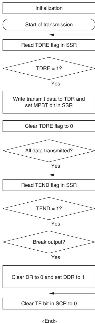
Figure 15.11 Sample Multiprocessor Serial Transmission Flowchart
