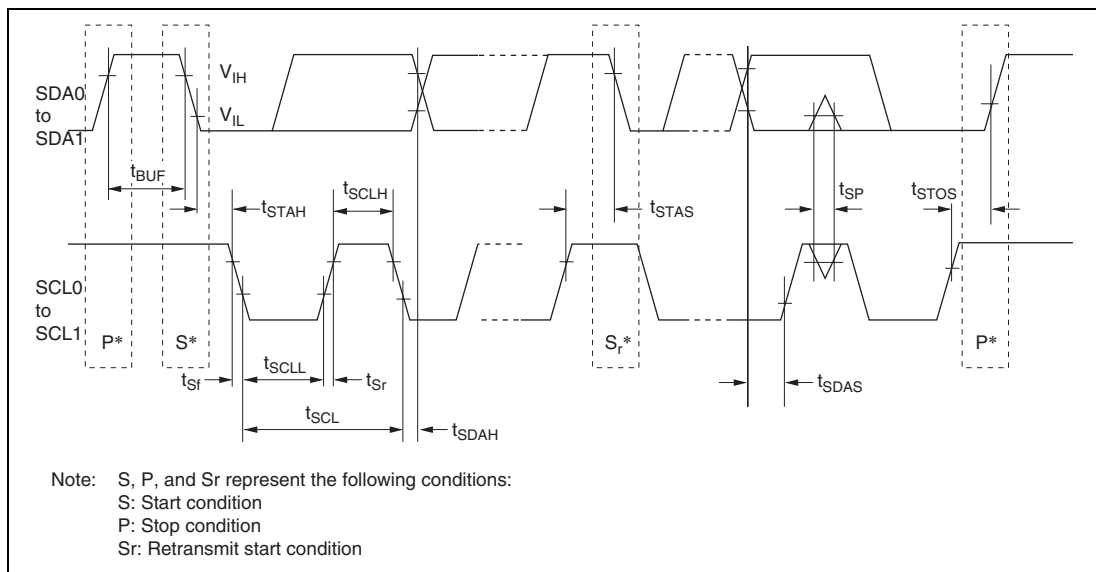
Figure 25.85 I²C Bus Interface 2 Input/Output Timing
