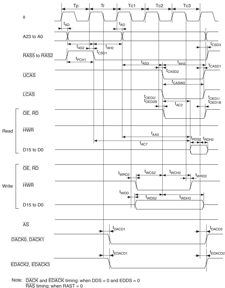
Figure 25.18 DRAM Access Timing: Three-State Access (RAST = 1)
