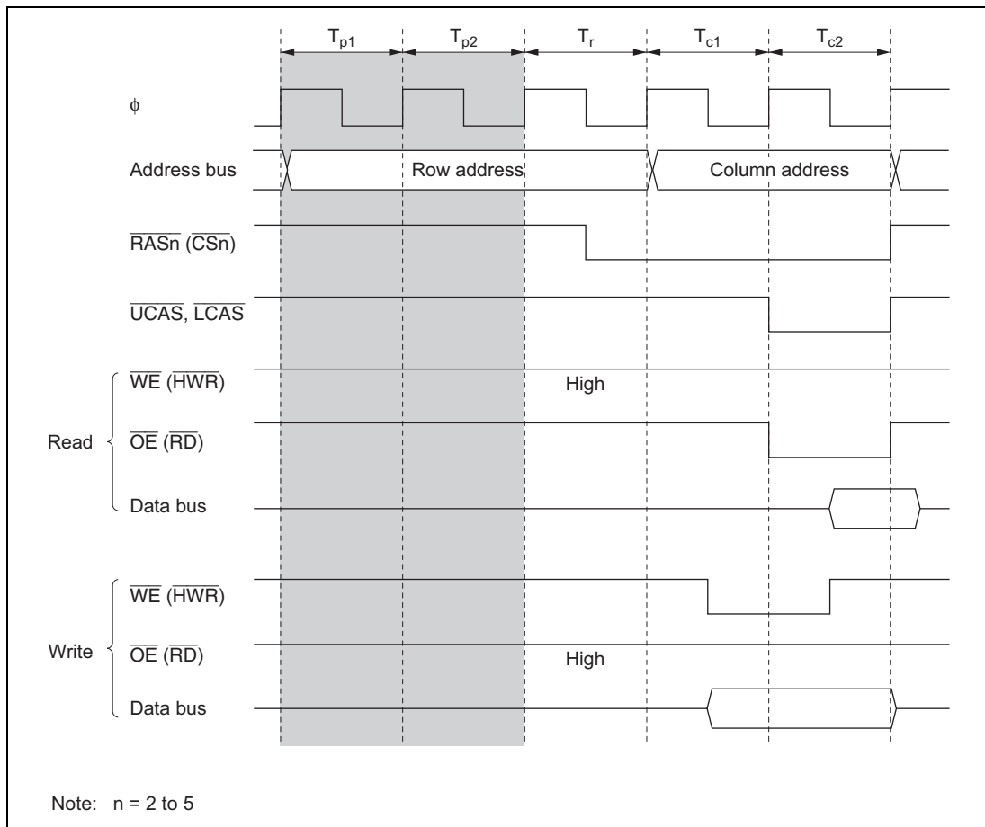
Figure 6.37 Example of Timing with Two-State Precharge Cycle ( \text{RAST} = 0 , \text{CAST} = 0 )
