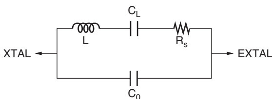
Figure 22.3 Crystal Resonator Equivalent Circuit
