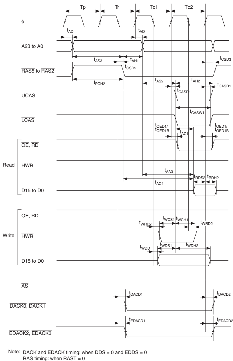
Figure 25.15 DRAM Access Timing: Two-State Access
