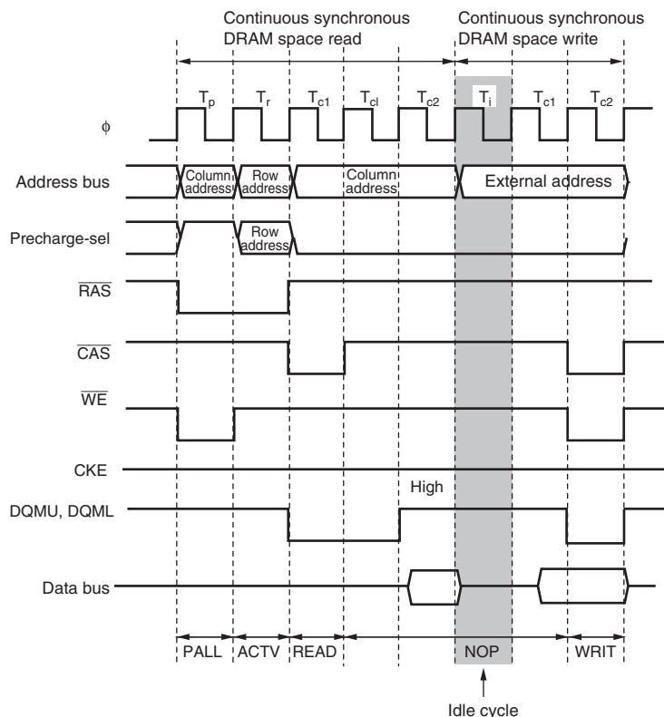
Figure 6.94 Example of Timing for Idle Cycle Insertion in Case of Consecutive Read and Write Accesses to Continuous Synchronous DRAM Space in RAS Down Mode (SDWCD = 1, CAS Latency 2)
