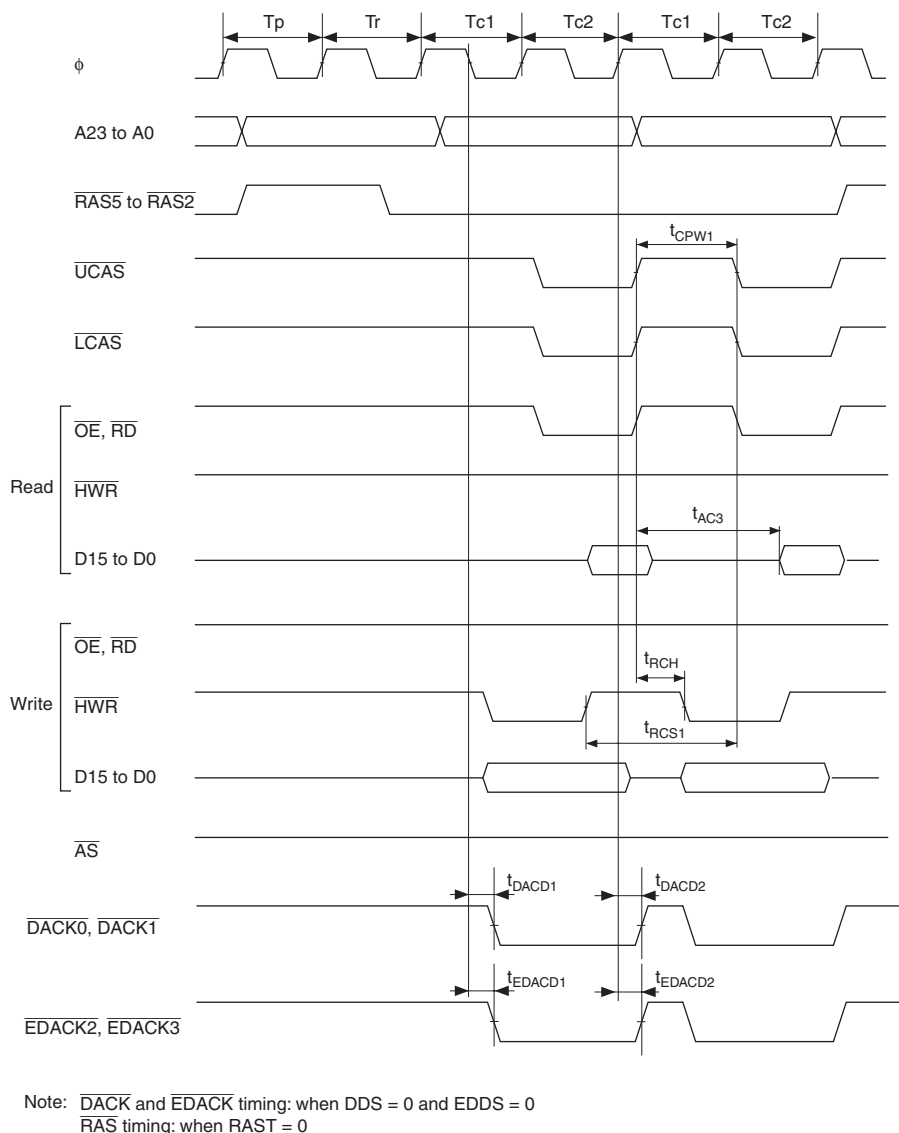
Figure 25.17 DRAM Access Timing: Two-State Burst Access
