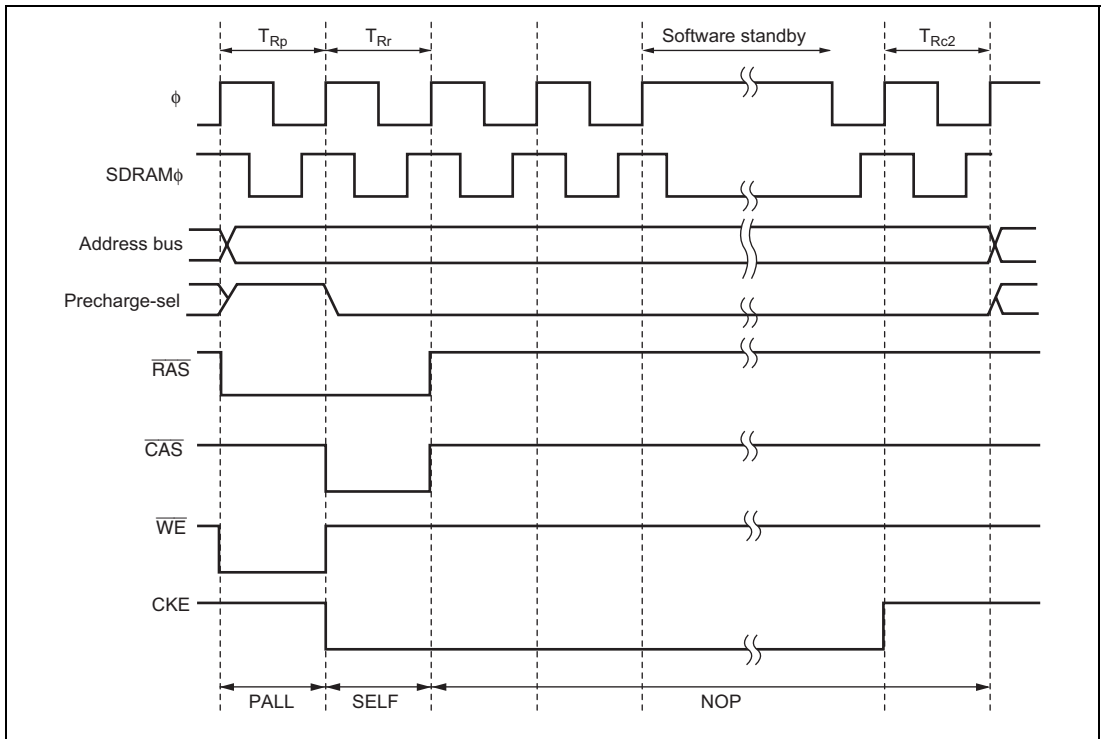
Figure 6.69 Self-Refresh Timing
