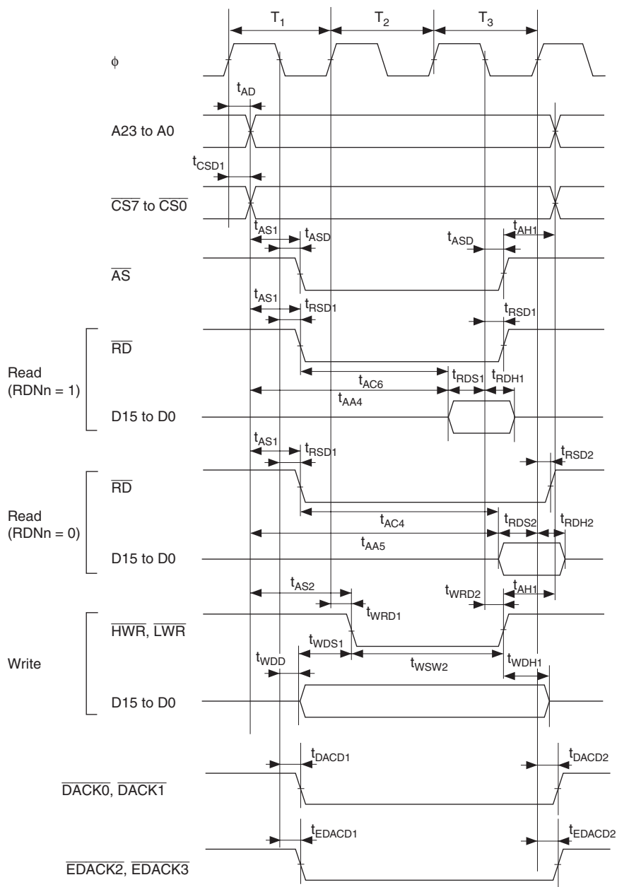
Figure 25.59 Basic Bus Timing: Three-State Access
