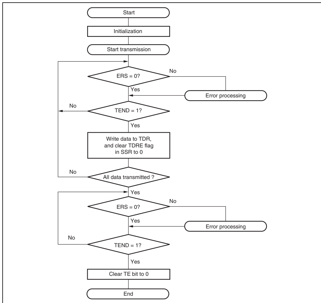
Figure 15.28 Example of Transmission Processing Flow
