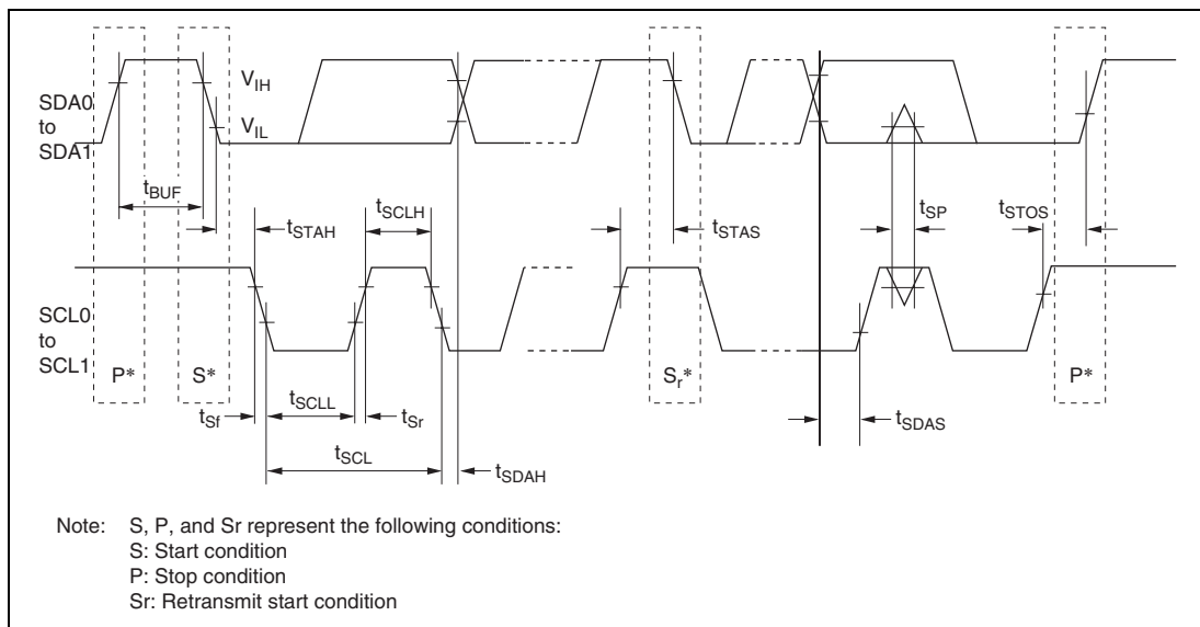
Figure 25.47 I²C Bus Interface 2 Input/Output Timing
