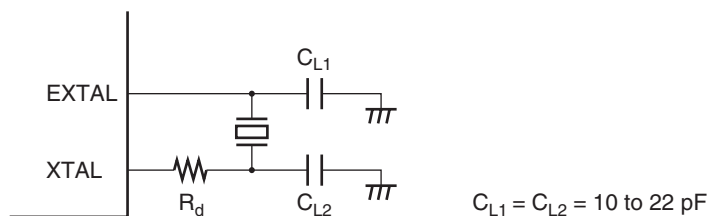
Figure 22.2 Connection of Crystal Resonator (Example)
