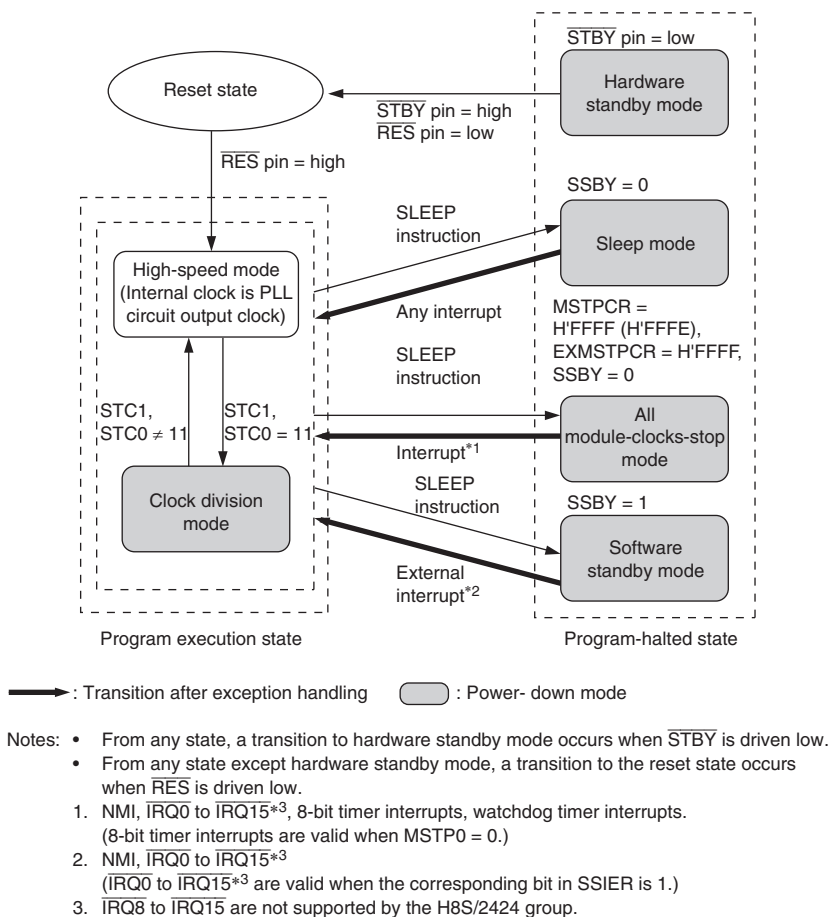
Figure 23.1 Mode Transitions
