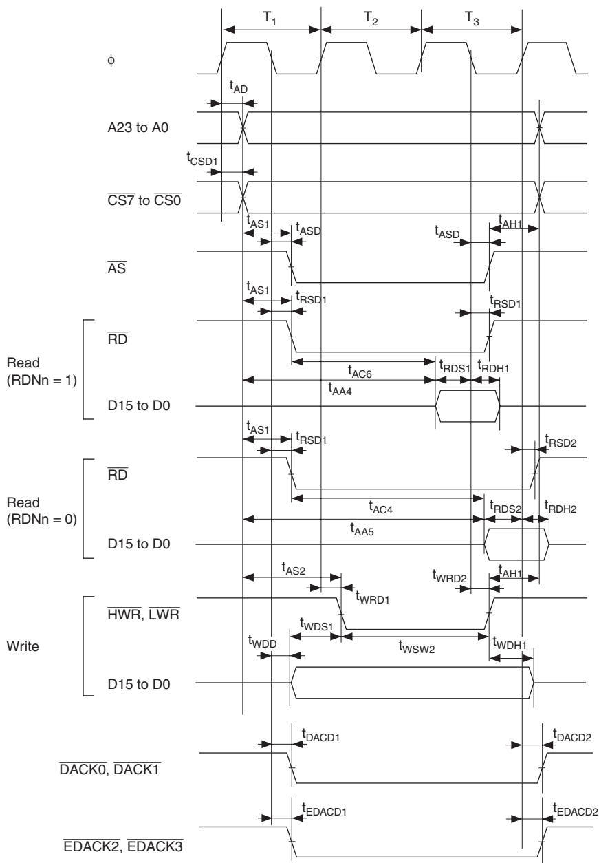
Figure 25.9 Basic Bus Timing: Three-State Access
