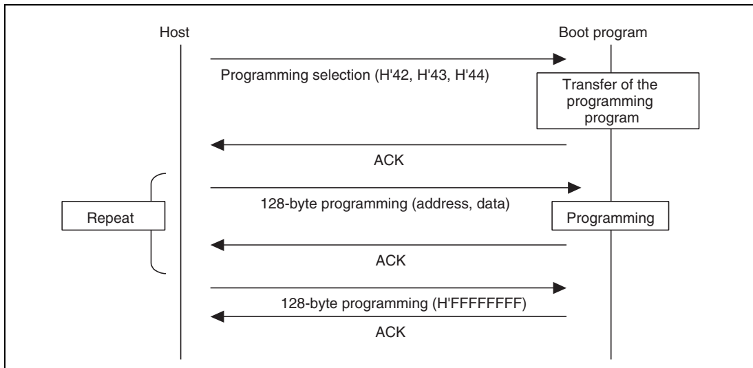
Figure 21.12 Programming Sequence
