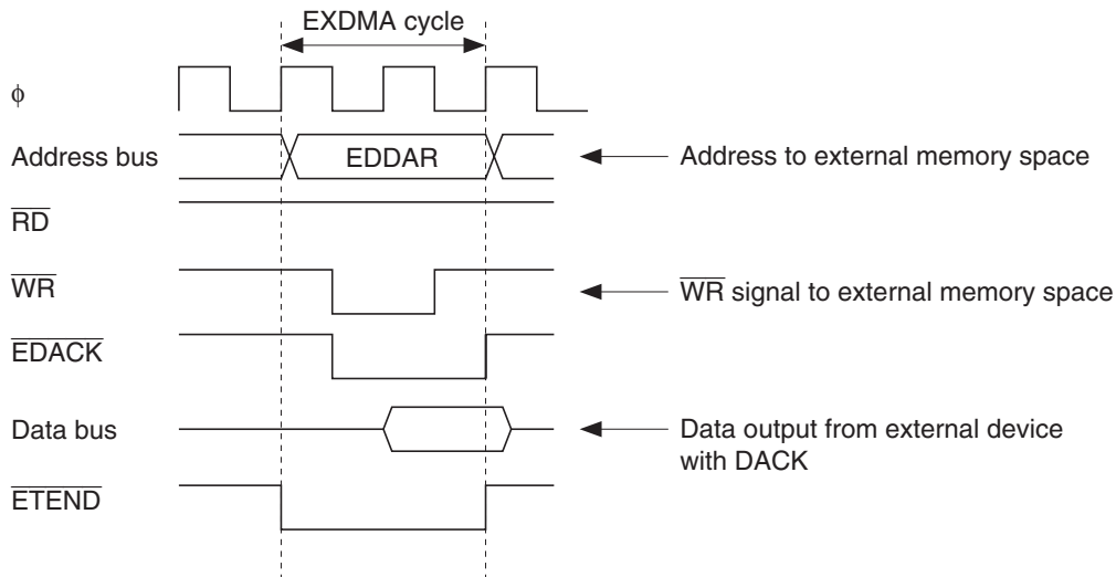
Figure 8.4 Example of Timing in Single Address Mode
