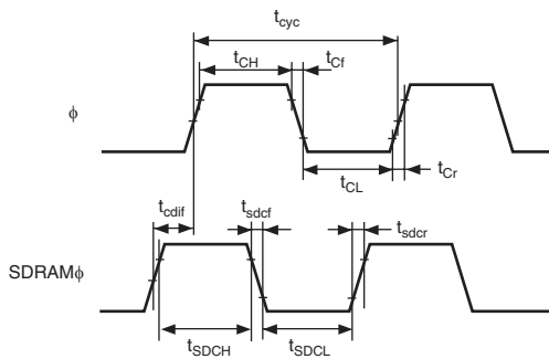
Figure 25.4 SDRAMφ Timing
