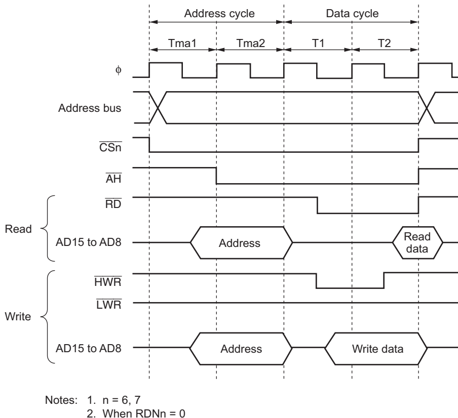
Figure 6.21 Bus Timing for 8-Bit, 2-State Data Access Space
