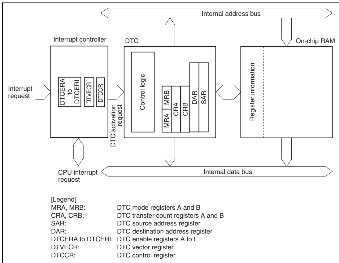
Figure 9.1 Block Diagram of DTC
