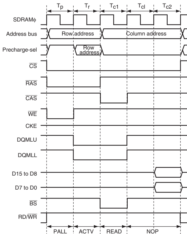
Figure 9.60 SDRAM Basic Read Access Timing (CAS Latency = 2)
