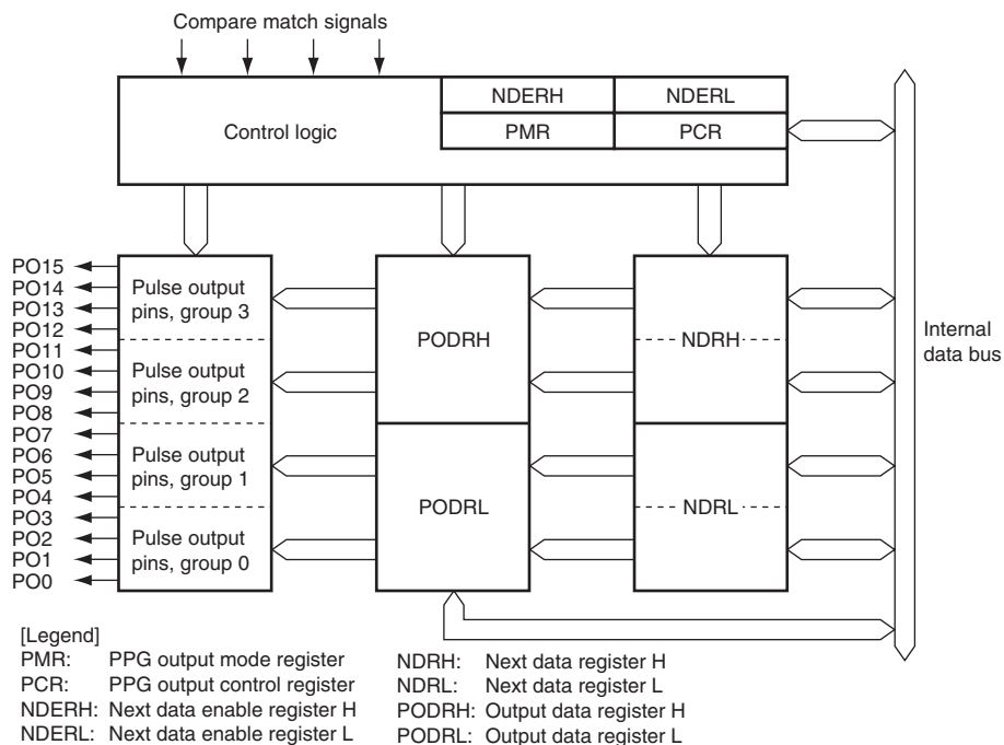
Figure 15.1 Block Diagram of PPG (Unit 0)
