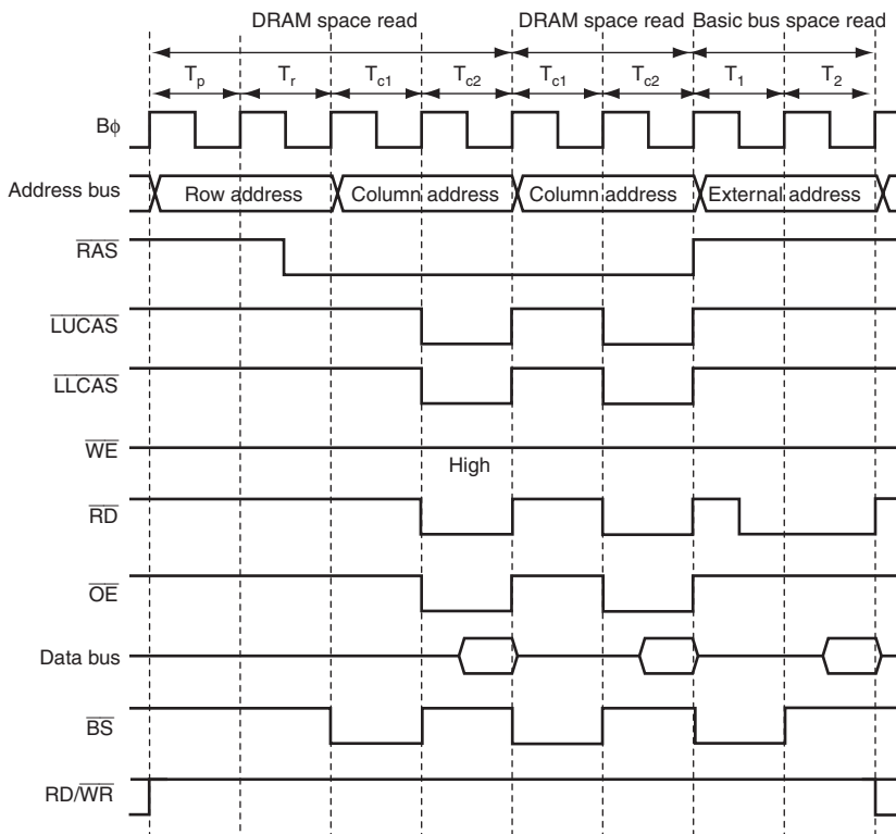
Figure 9.51 Timing Example of RAS Up Mode ( \text{RAST} = 0 , \text{CAST} = 0 )
