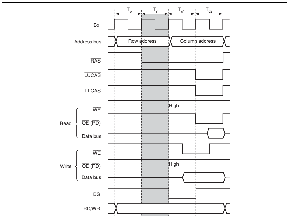
Figure 9.40 Access Timing Example of \overline{\text{RAS}} Signal Driven Low at Start of T_r Cycle ( \text{CAST} = 0 )
