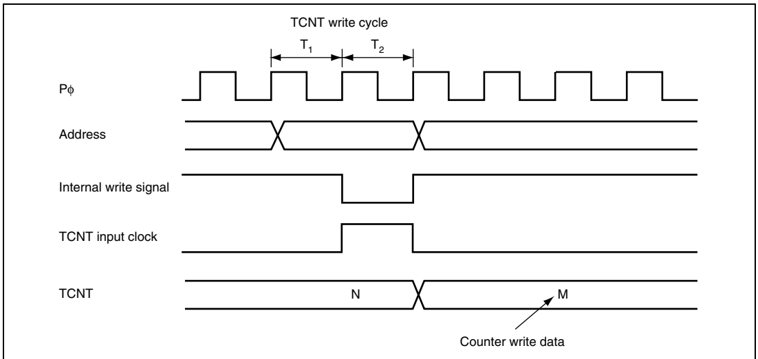
Figure 13.5 Conflict between TCNT Write and Increment
