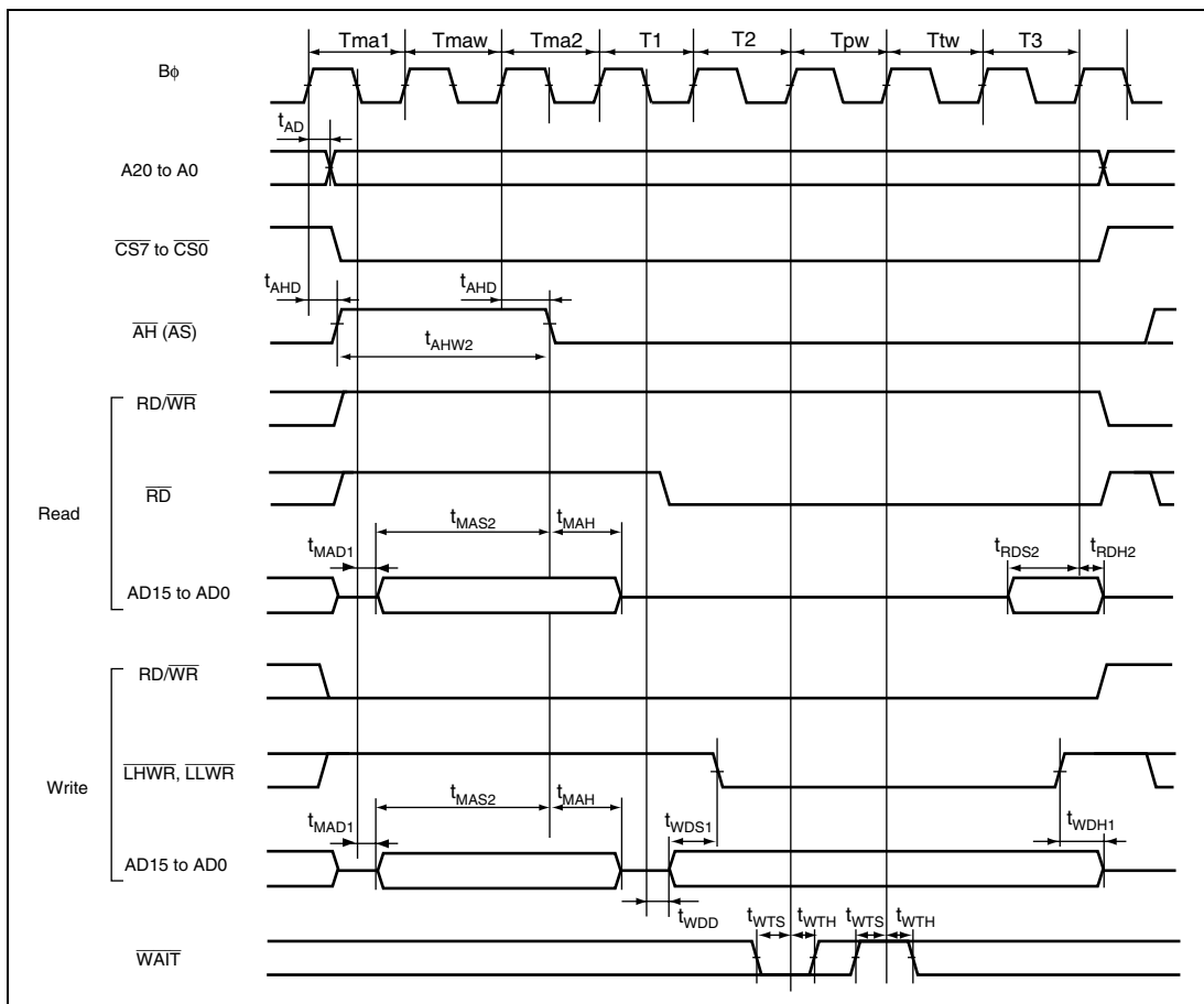
Figure 24.18 Address/Data Multiplexed Access Timing (Wait Control) (Address Cycle Program Wait \times 1 + Data Cycle Program Wait \times 1 + Data Cycle Pin Wait \times 1)
