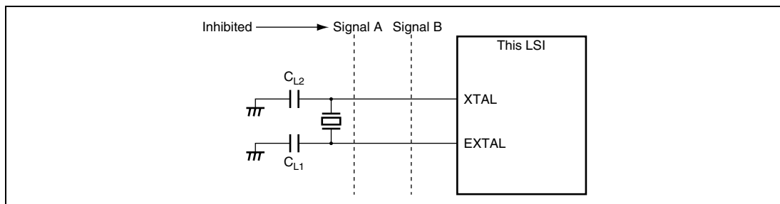
Figure 21.7 Note on Board Design for Oscillation Circuit
