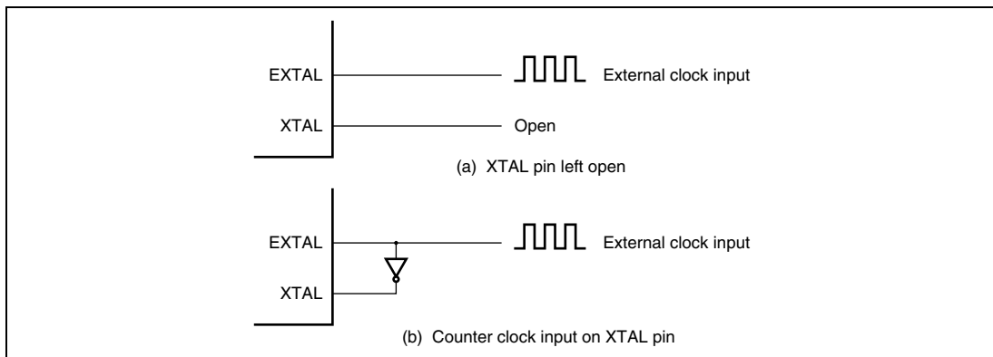
Figure 21.4 External Clock Input (Examples)
