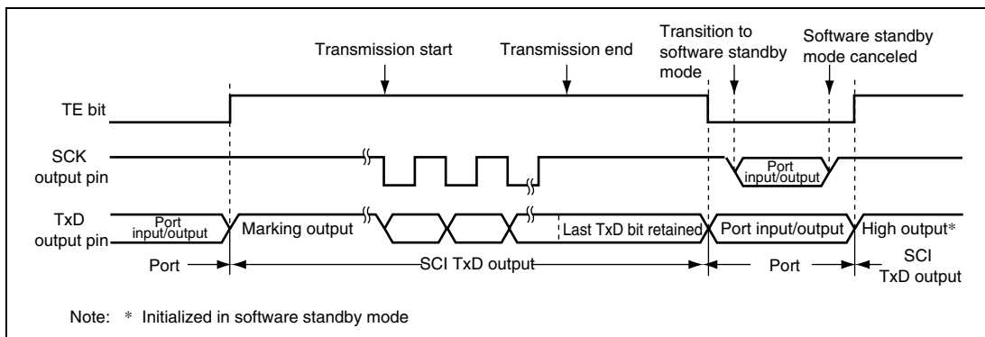
Figure 14.41 Port Pin States during Mode Transition (Internal Clock, Clocked Synchronous Transmission) (Setting is Prohibited in SCI_5 and SCI_6)
