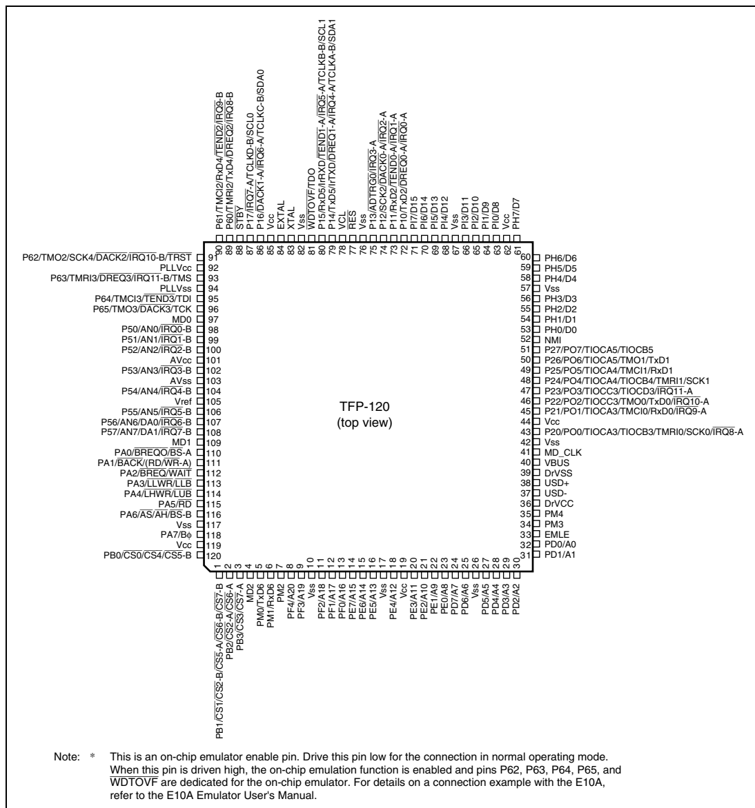
Figure 1.2 Pin Assignments
