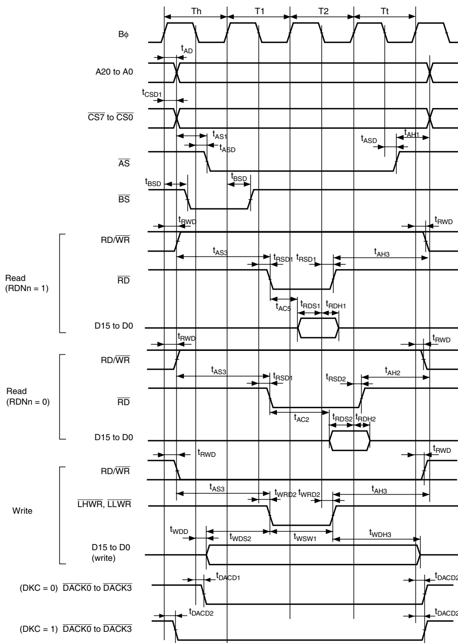
Figure 24.11 Basic Bus Timing: Two-State Access ( \overline{CS} Assertion Period Extended)
