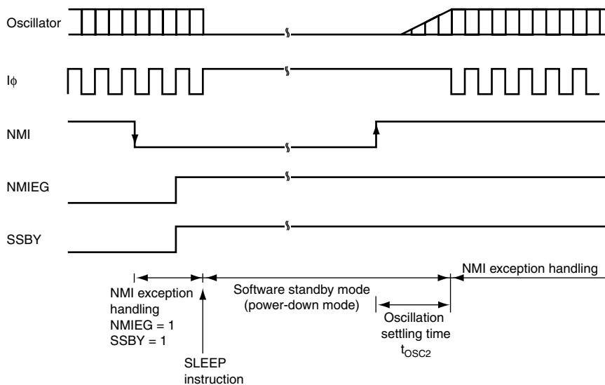
Figure 24.3 Oscillation Settling Timing after Software Standby Mode
