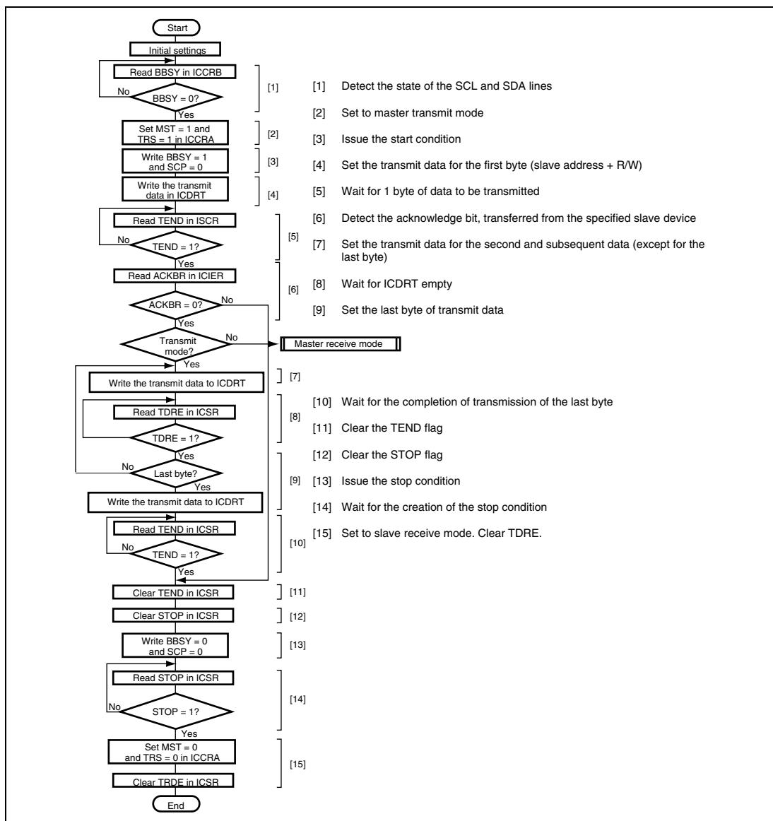
Figure 16.14 Sample Flowchart of Master Transmit Mode
