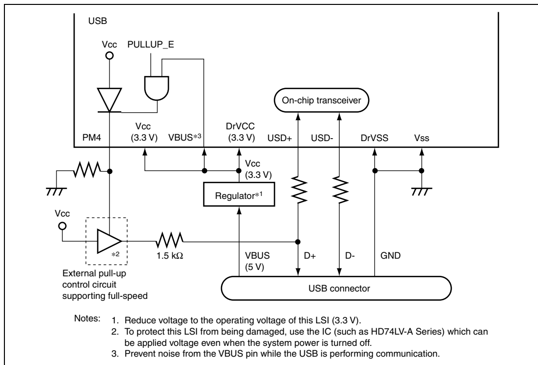
Figure 15.22 Example of Circuitry in Bus Power Mode
