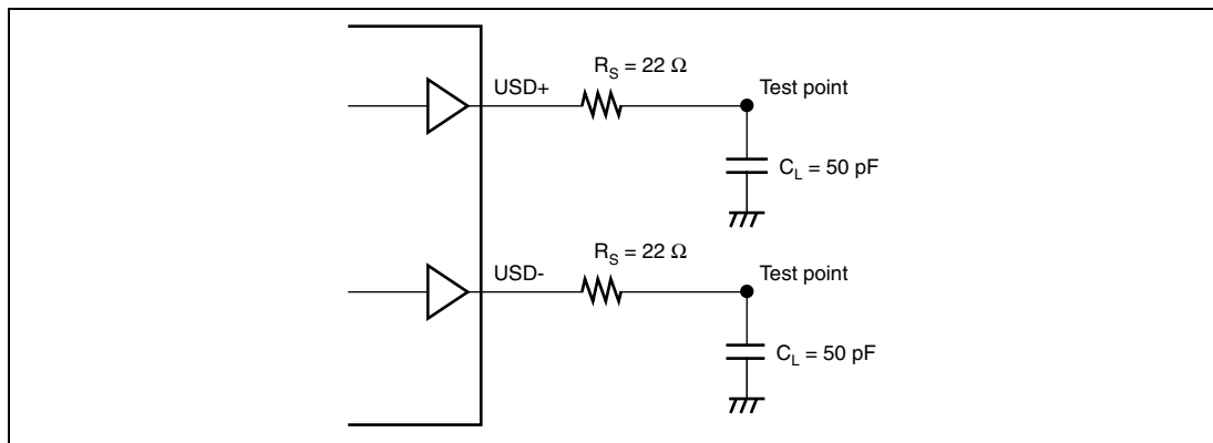
Figure 24.38 Load Condition
