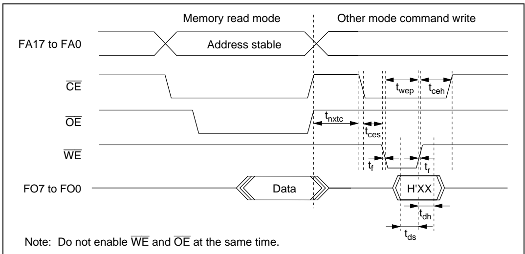
Figure 23.17 Timing Waveforms when Entering Another Mode from Memory Read Mode
