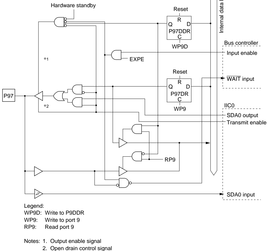
Figure C.33 Port 9 Block Diagram (Pin P97)
