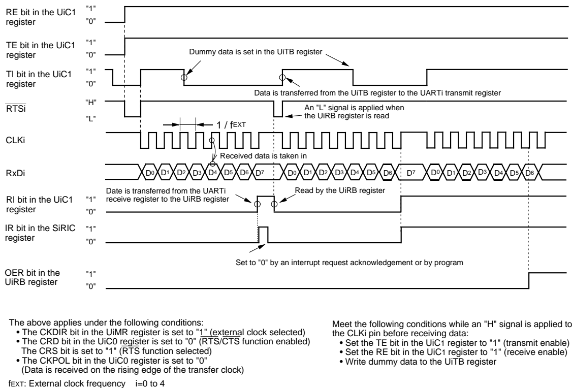
Figure 16.10 Transmit and Receive Operation
