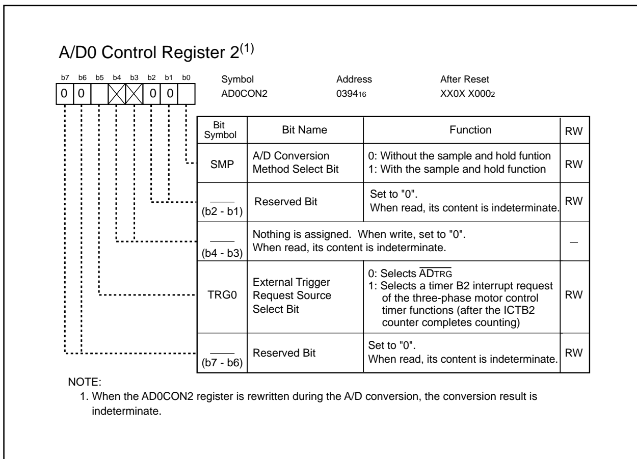
Figure 17.4 AD0CON2 Register
