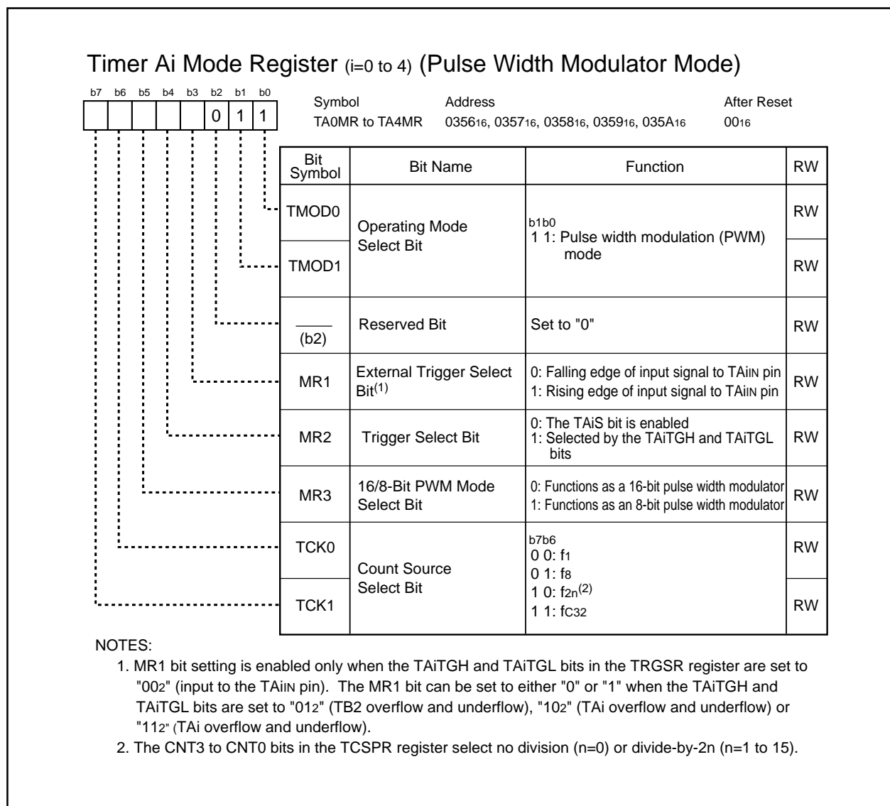
Figure 14.13 TA0MR to TA4MR Registers
