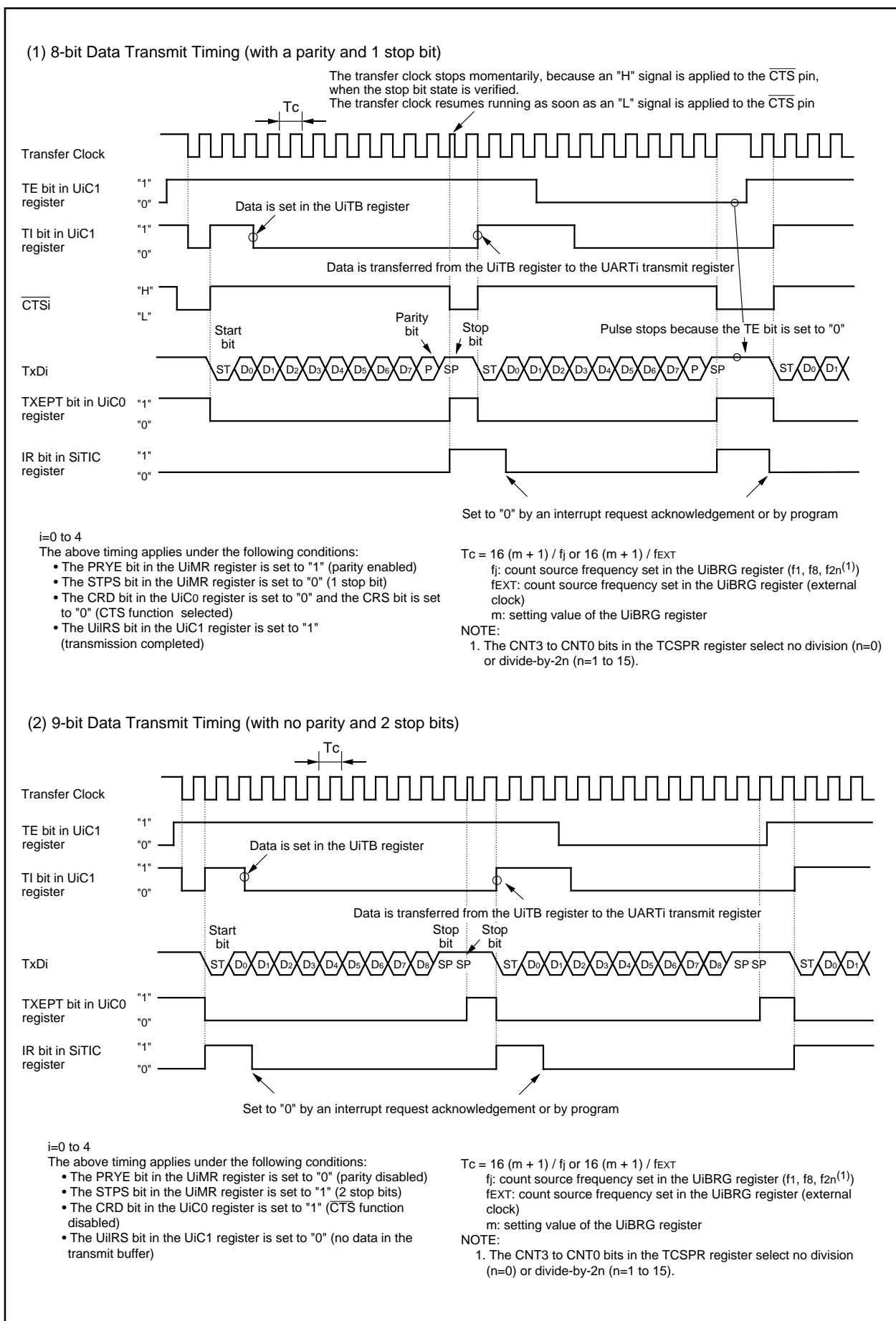
Figure 16.14 Transmit Operation
