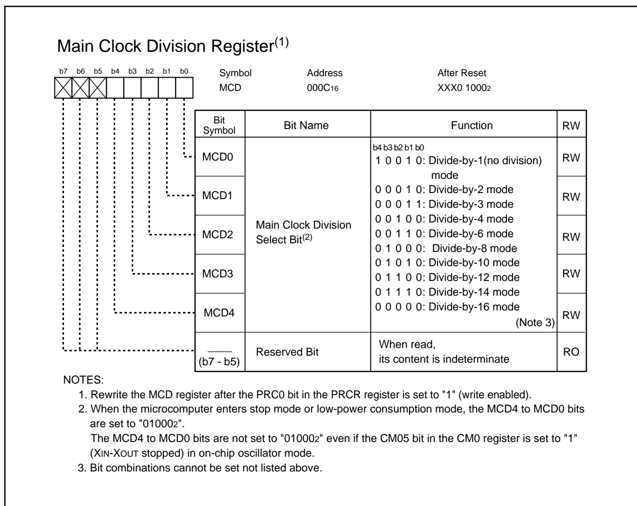
Figure 8.4 MCD Register
