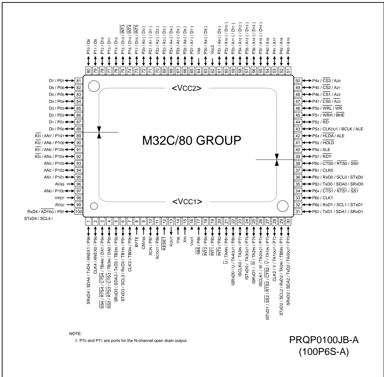
Figure 1.3 Pin Assignment
