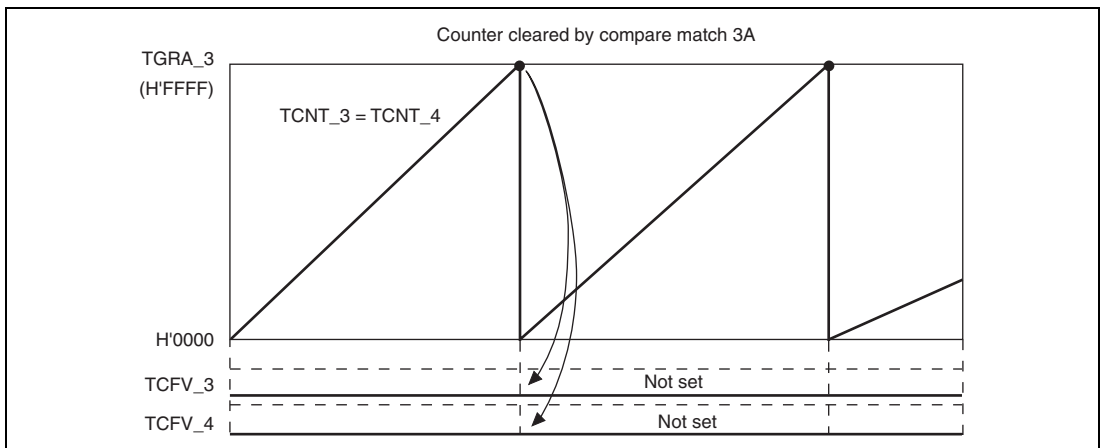
Figure 11.82 Reset Synchronous PWM Mode Overflow Flag
