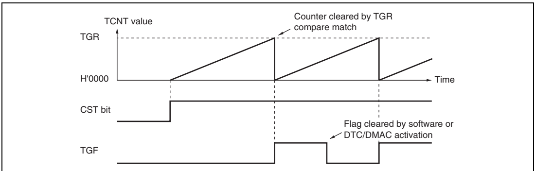
Figure 11.5 Periodic Counter Operation
