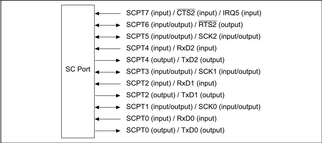
Figure 19.12 SC Port
