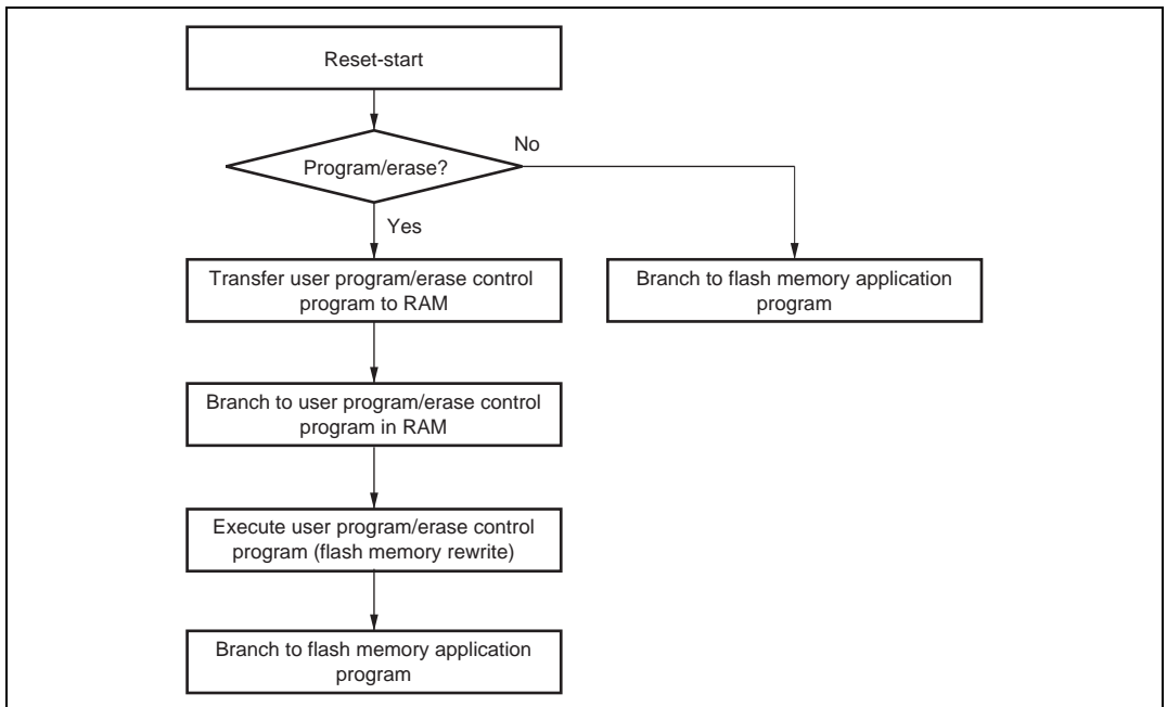
Figure 20.8 Programming/Erasing Flowchart Example in User Program Mode
