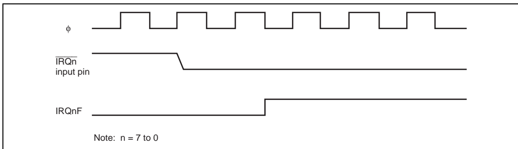
Figure 5.3 Set Timing for \text{IRQnF}
