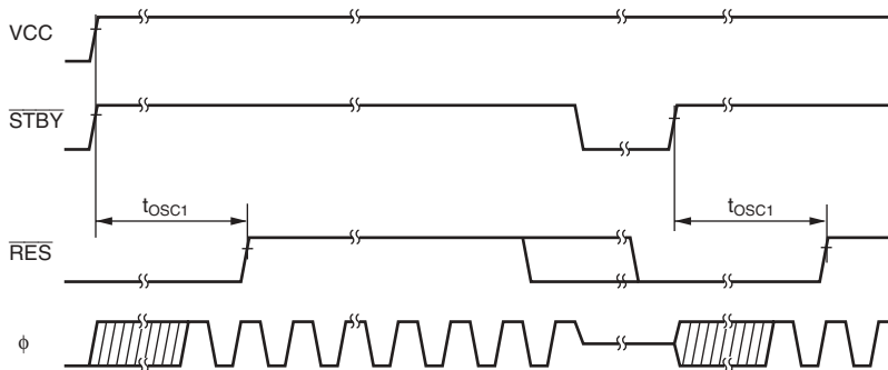
Figure 25.5 Oscillation Stabilization Timing
