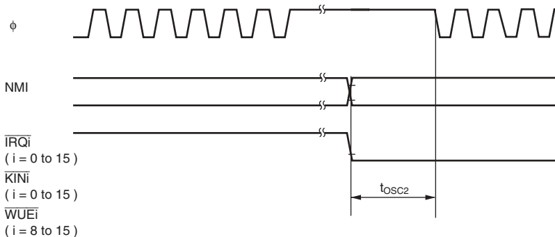
Figure 25.6 Oscillation Stabilization Timing (Exiting Software Standby Mode)
