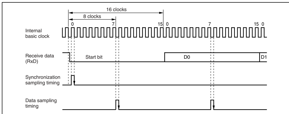
Figure 14.4 Receive Data Sampling Timing in Asynchronous Mode
