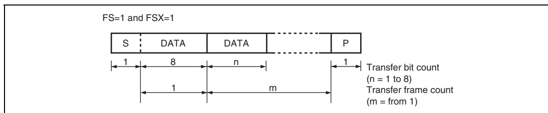
Figure 15.4 I 2 C Bus Data Formats (Serial Formats)
