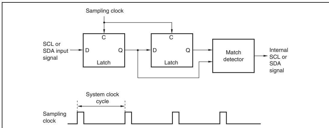
Figure 15.28 Block Diagram of Noise Canceler
