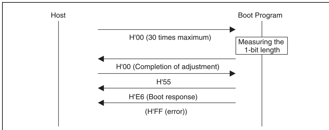
Figure 20.20 Bit-Rate-Adjustment Sequence
