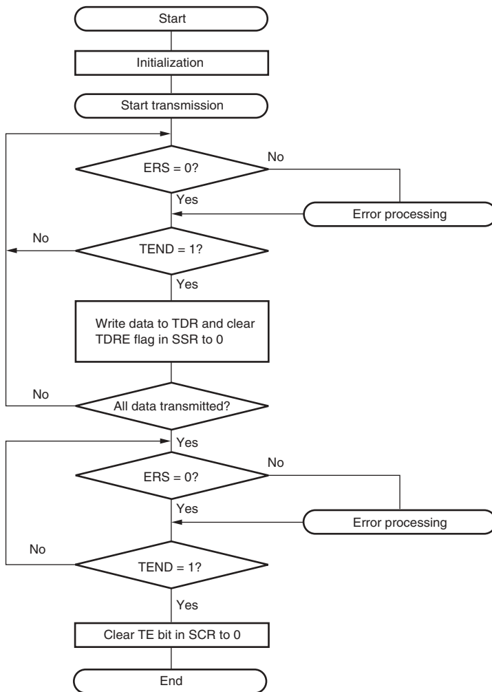
Figure 14.31 Sample Transmission Flowchart
