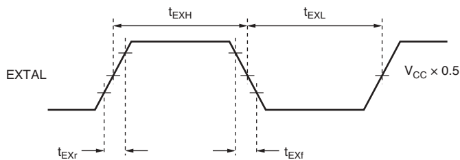
Figure 25.7 External Clock Input Timing
