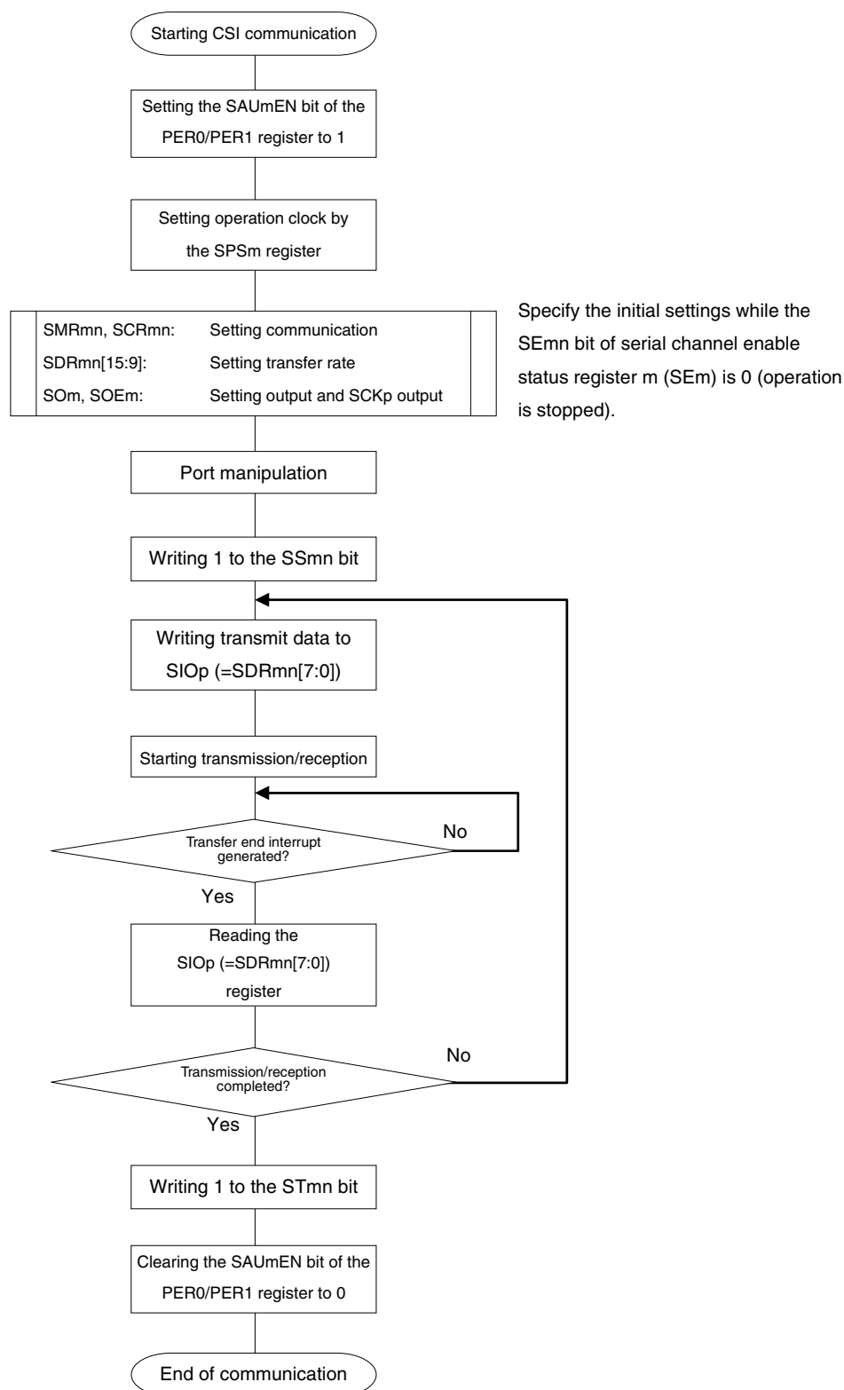
Figure 14-49. Flowchart of Master Transmission/Reception (in Single- Transmission/Reception Mode)
