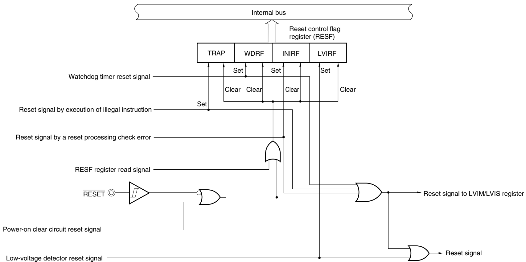
Figure 21-1. Block Diagram of Reset Function
