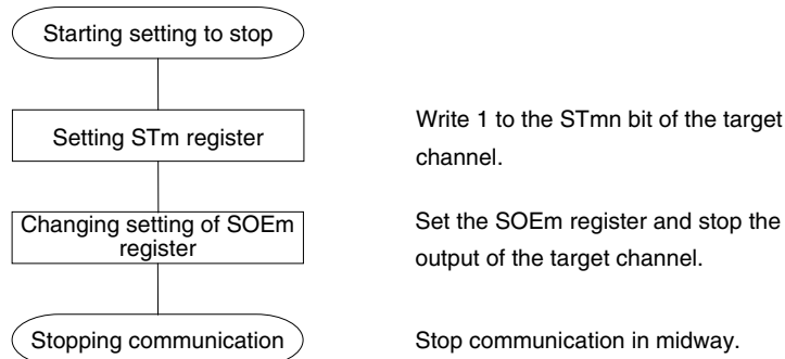
Figure 13-42. Procedure for Stopping Master Transmission/Reception
