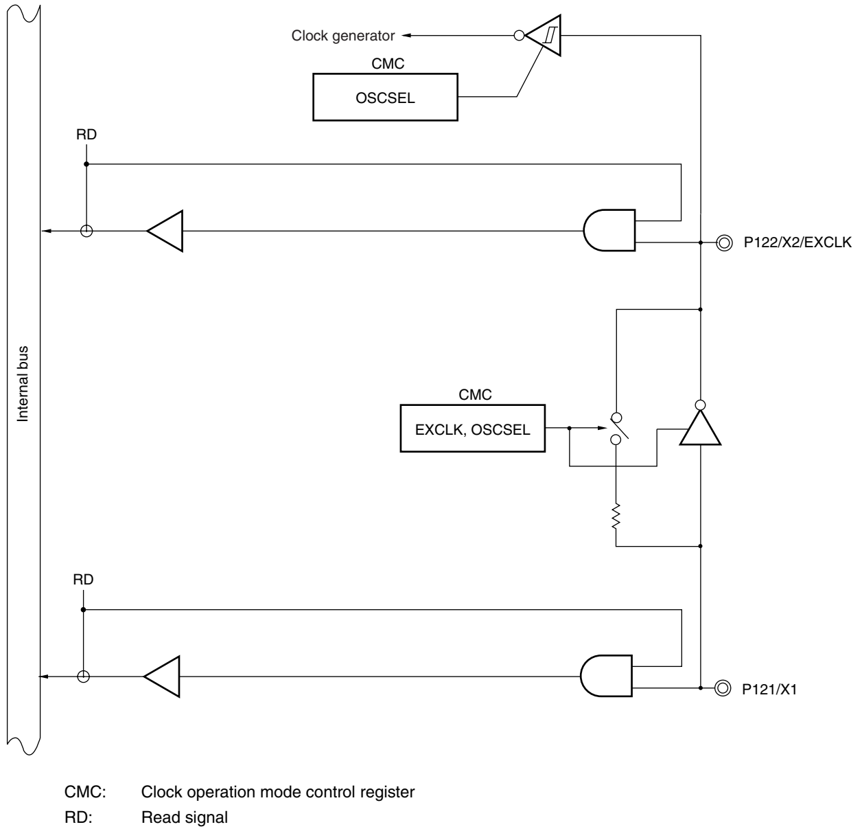
Figure 4-40. Block Diagram of P121 and P122
