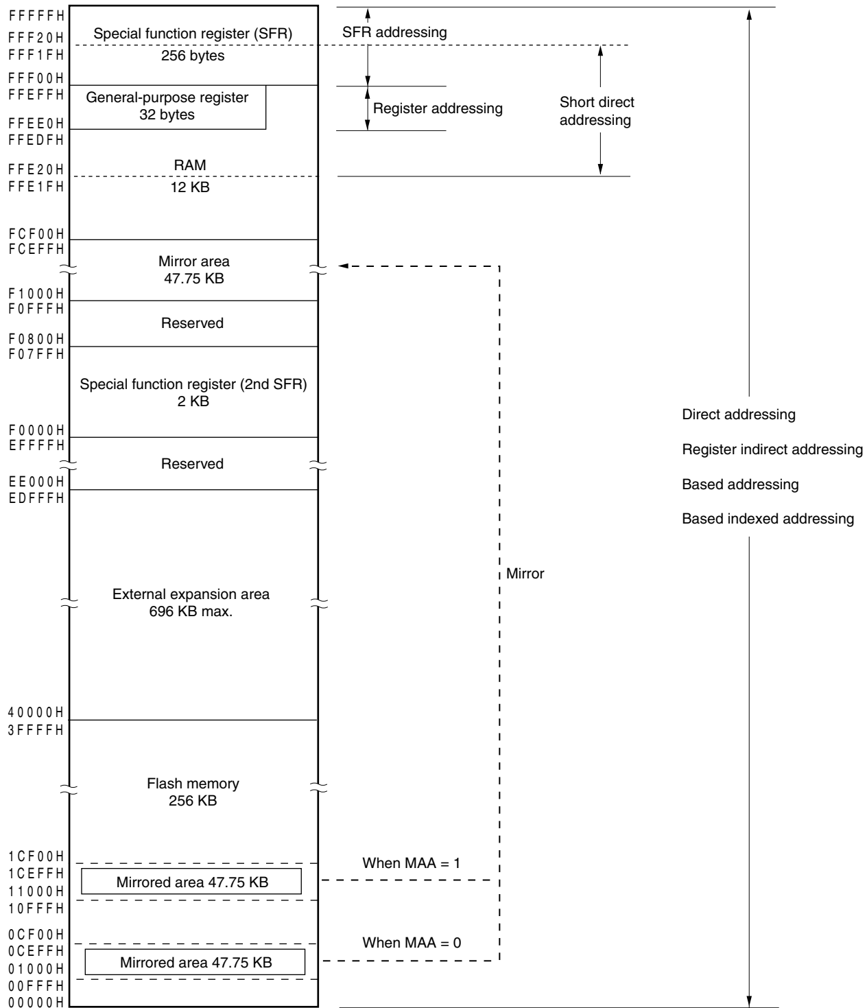
Figure 3-9. Correspondence Between Data Memory and Addressing ( \mu PD78F1186A)
