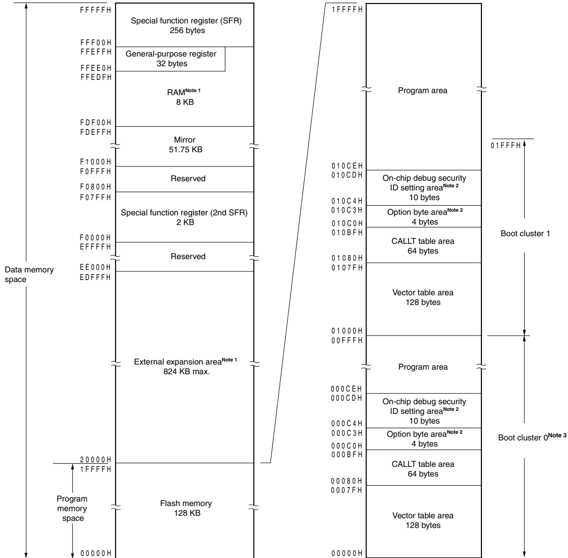
Figure 3-1. Memory Map (μPD78F1184A)
