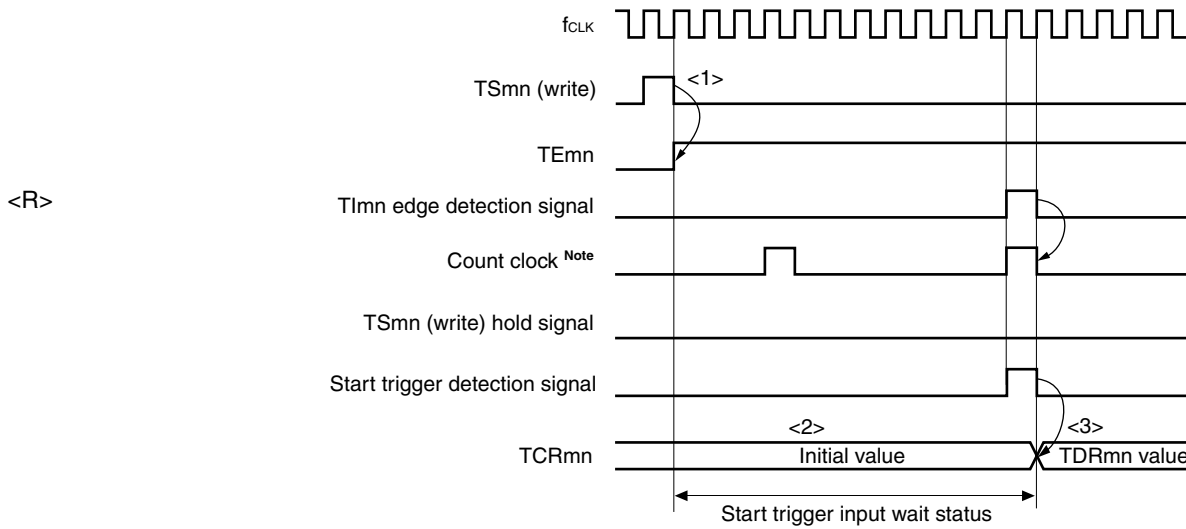
Figure 7-14. Start Timing (In One-count Mode)
