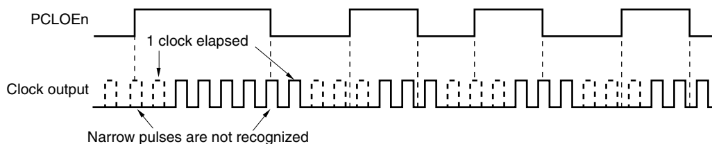
<R> Figure 10-4. Remote Control Output Application Example
