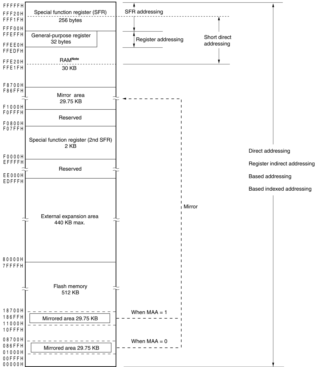
Figure 3-11. Correspondence Between Data Memory and Addressing ( \mu PD78F1188A)
