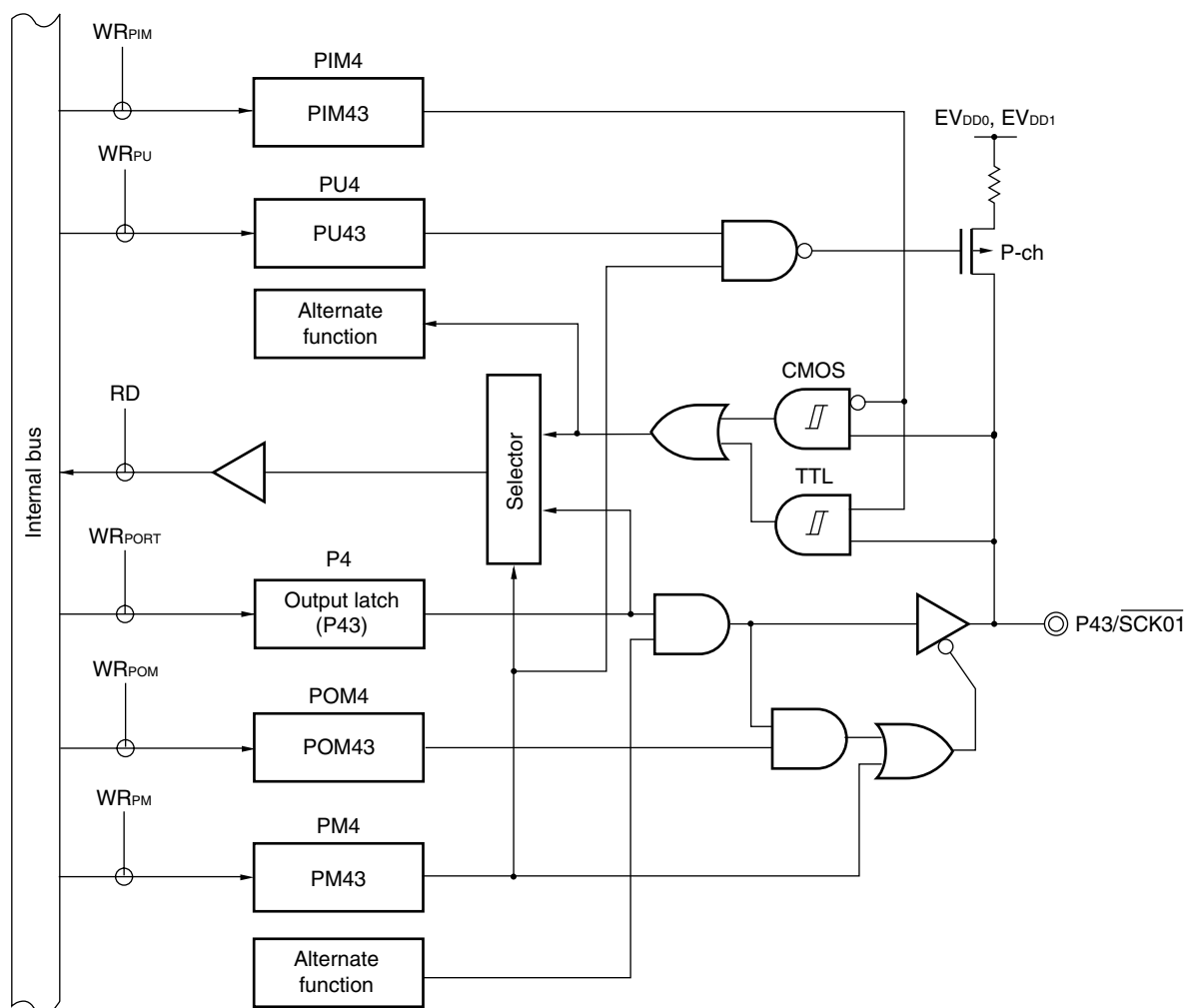
Figure 4-20. Block Diagram of P43
