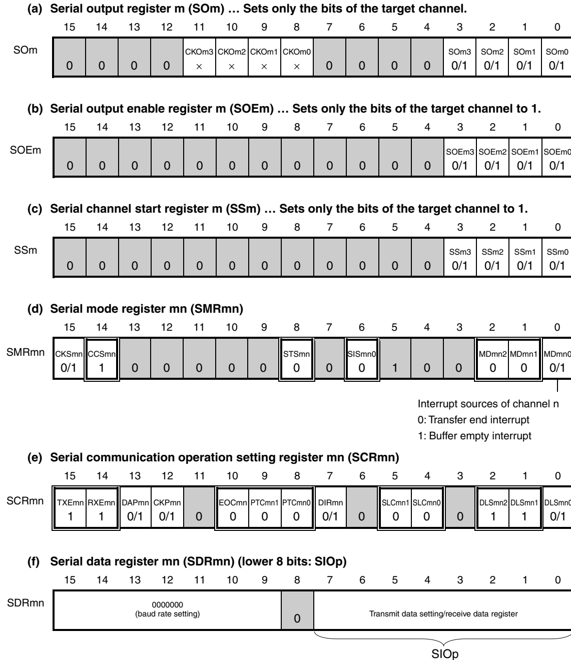
Figure 13-62. Example of Contents of Registers for Slave Transmission/Reception of 3-Wire Serial I/O (CSI00, CSI01, CSI10, CSI11, CSI20, CSI21)
