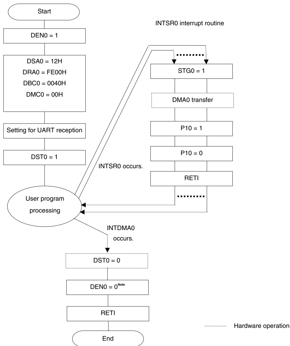
Figure 16-11. Example of Setting for UART Consecutive Reception + ACK Transmission
