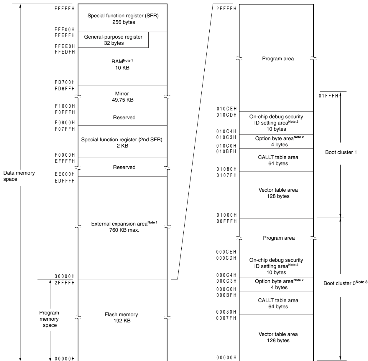
Figure 3-2. Memory Map (μPD78F1185A)
