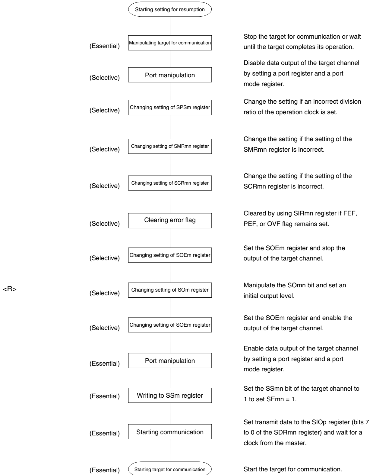
Figure 13-51. Procedure for Resuming Slave Transmission
