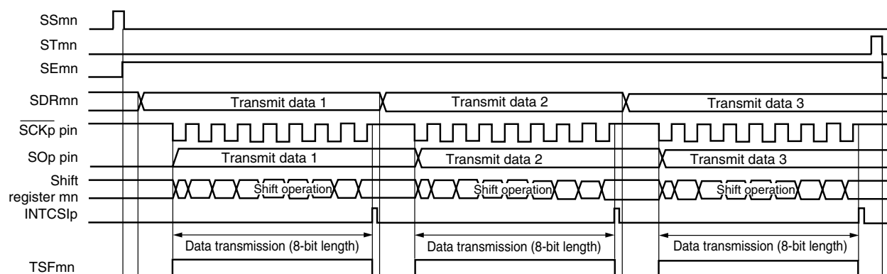
Figure 13-52. Timing Chart of Slave Transmission (in Single-Transmission Mode) (Type 1: DAPmn = 0, CKPmn = 0)
