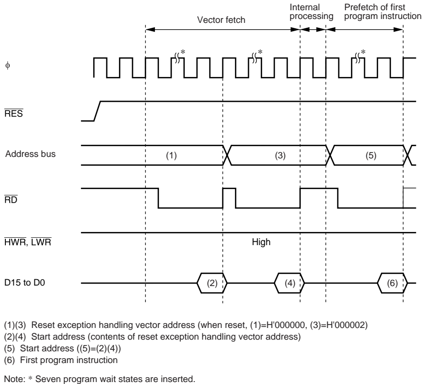
Figure 4.2 Reset Sequence (Advanced Mode with On-Chip ROM Disabled)
