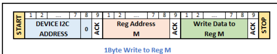
Figure 48. 1-Byte Write to Register M
