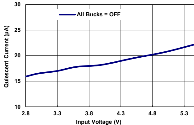
Figure 35. Quiescent Current (All Bucks Off) vs V_{IN}
