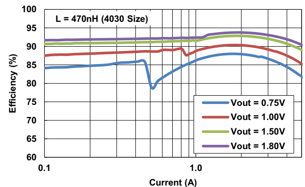
Figure 16. Single Phase Efficiency V_{IN} = 5.0V
