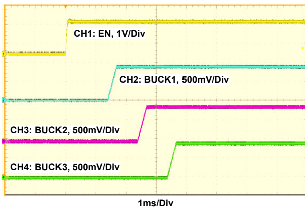
Figure 25. ISL91211AIK Startup by EN, V_{OUT1, 2, 3} = 0.9V
