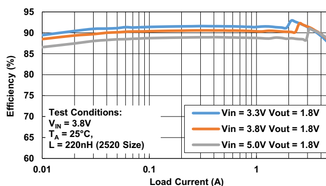
Figure 2. Single-Phase Efficiency vs Load Current
