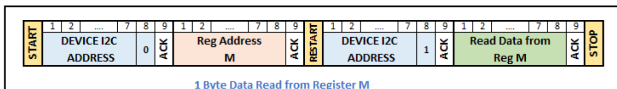
Figure 50. 1-Byte Data Read From Register M
