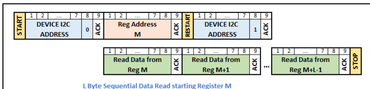
Figure 51. L-Byte Sequential Data Read Starting Register M
