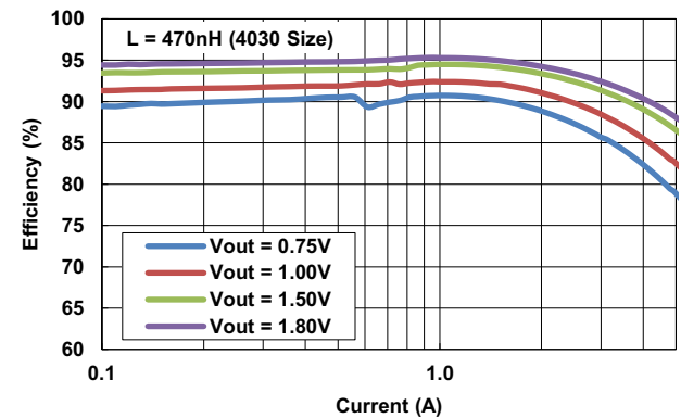
Figure 14. Single-Phase Efficiency V_{IN} = 3.3V
