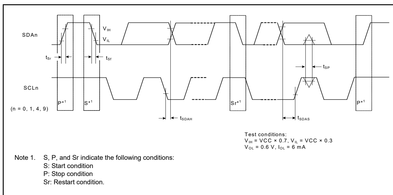
Figure 2.49 SCI simple IIC mode timing
