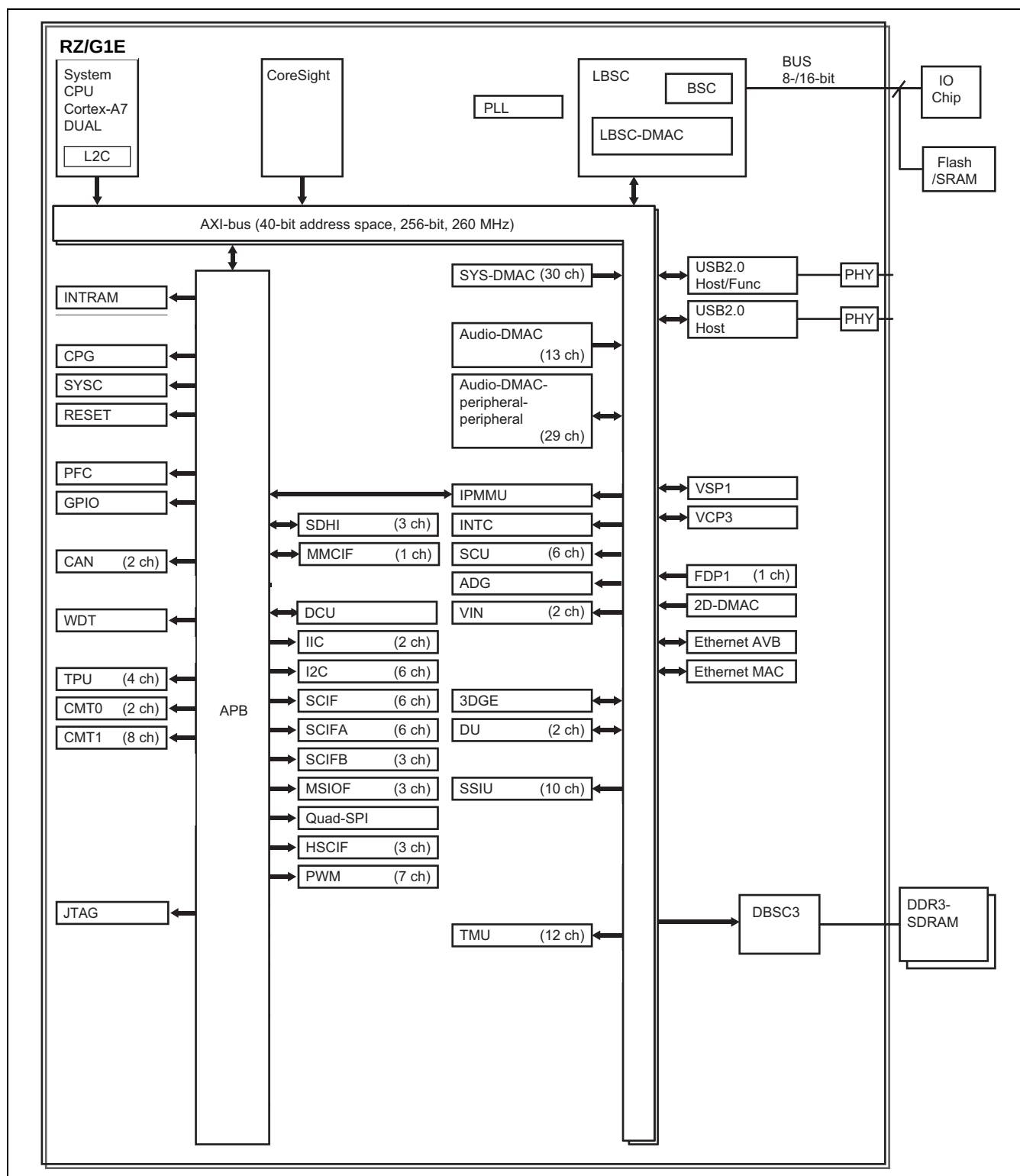
Figure 1.1 RZ/G1E System Configuration
