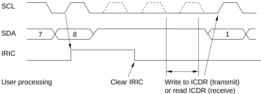
(c) When ACK = 1
