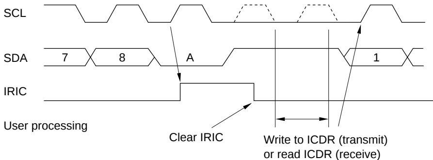
(b) When WAIT = 1 and ACK = 0
