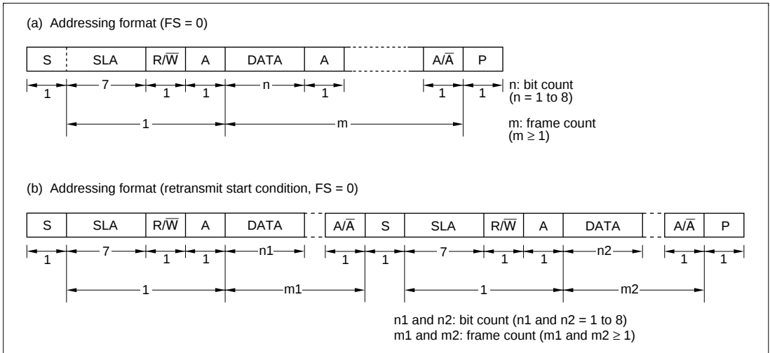
Figure 13.3 I 2 C Bus Data Formats (Acknowledge Formats)
