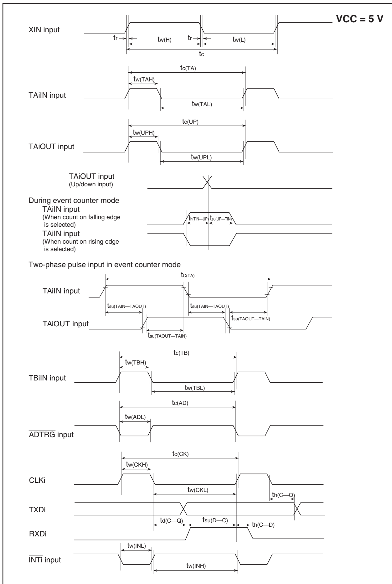
Figure 5.21 Timing Diagram
