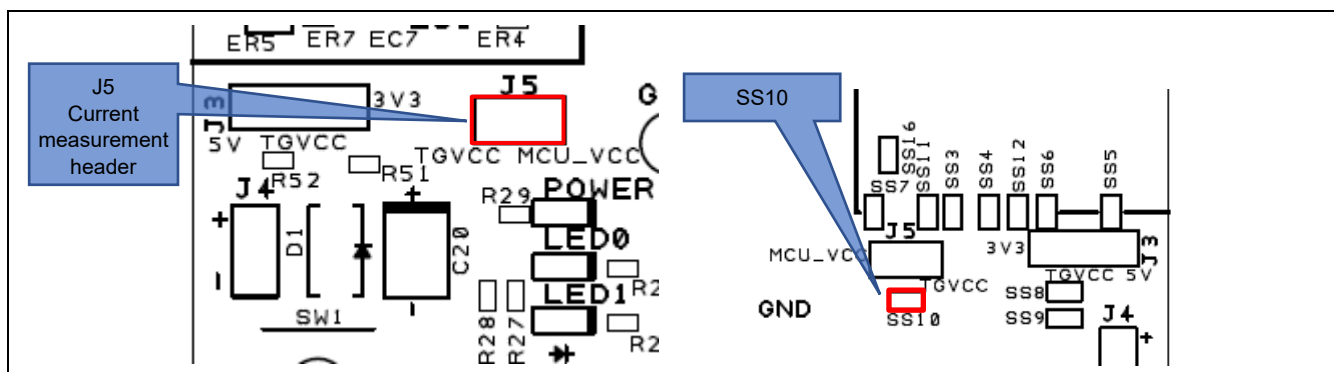
Figure 5-4 Positions of the Current Measurement Header (J5) (Top Side) & Pattern for Cutting (SS10) (Soldered Side)
