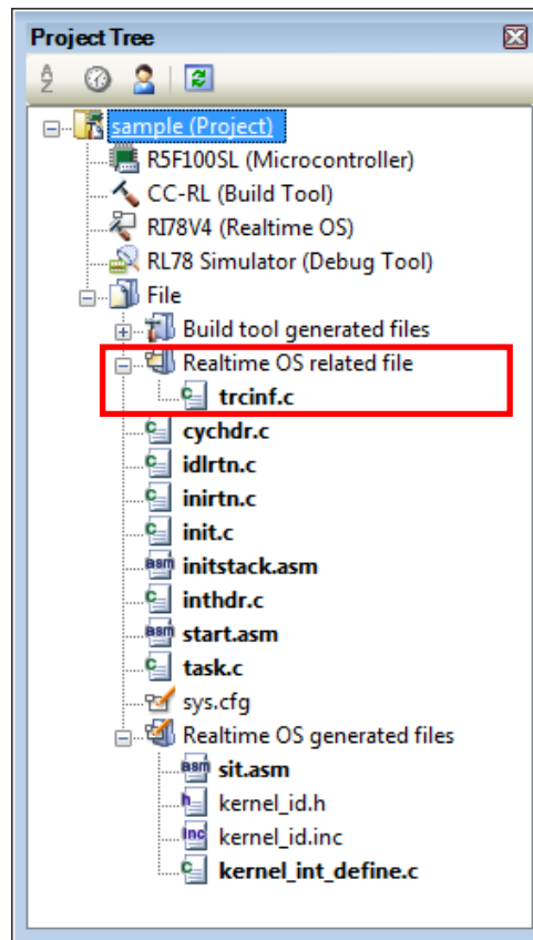
Figure 6-3 Project Tree
