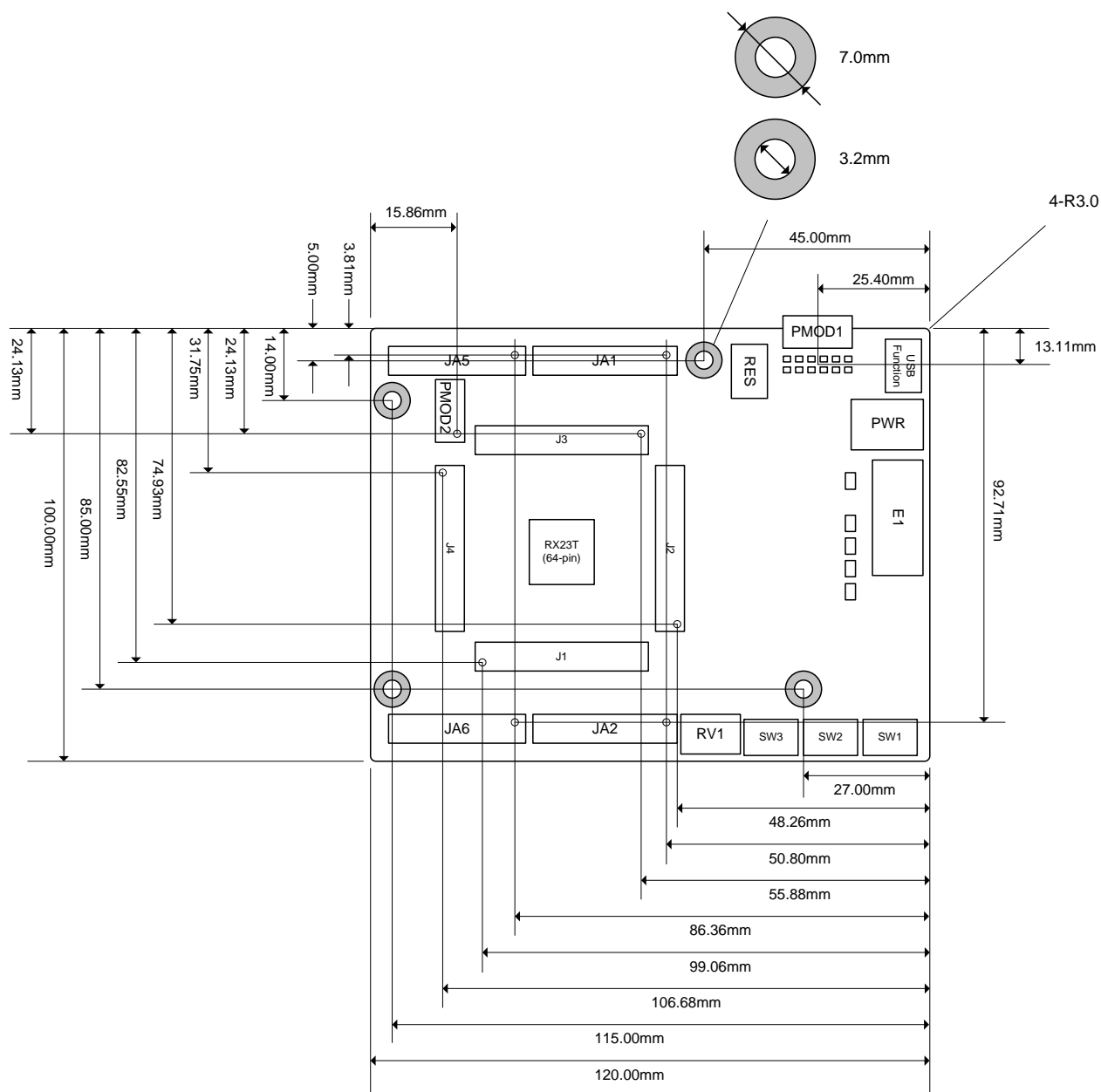
Figure 3-2: Board Dimensions
