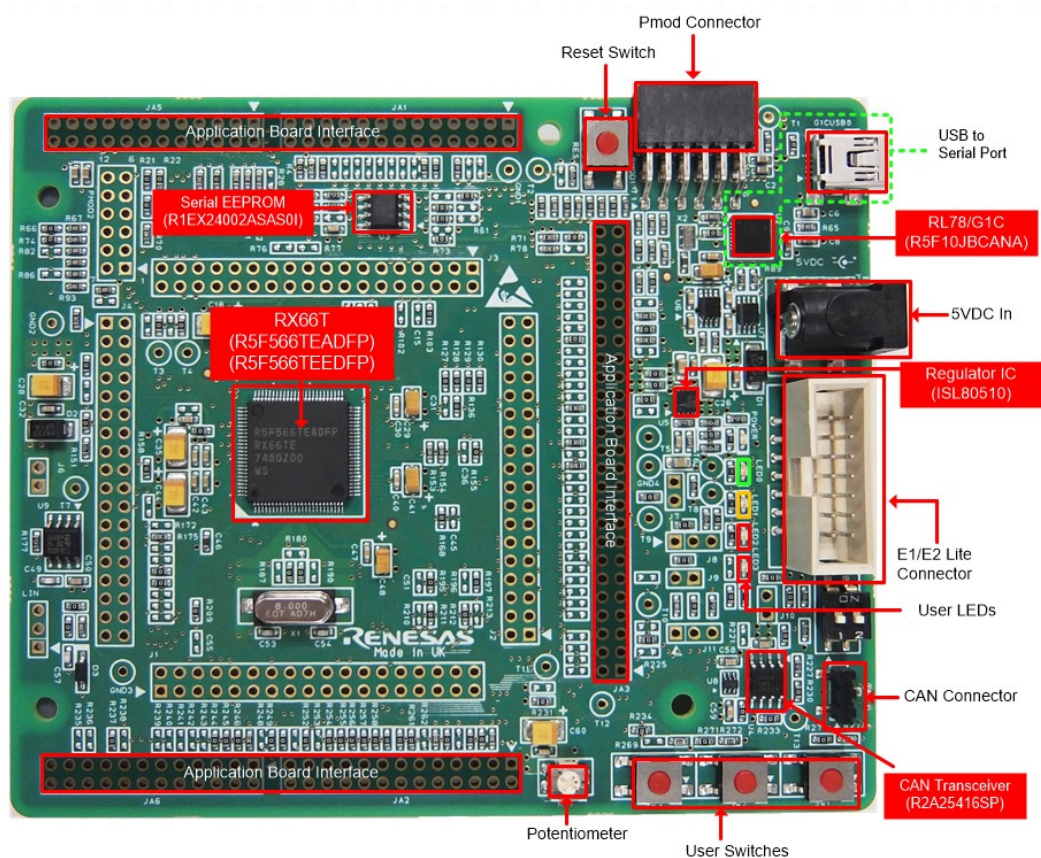
Figure 2 CPU Board
