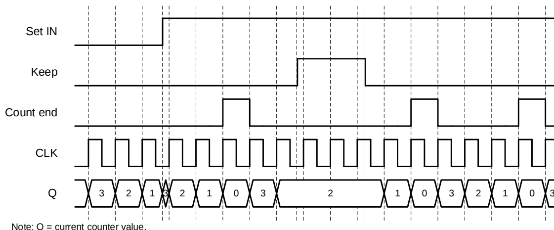
Figure 42. CNT/FSM Timing Diagram (Set Rising Edge Mode, OSC is Forced On, UP = 0) for CNT Data = 3
