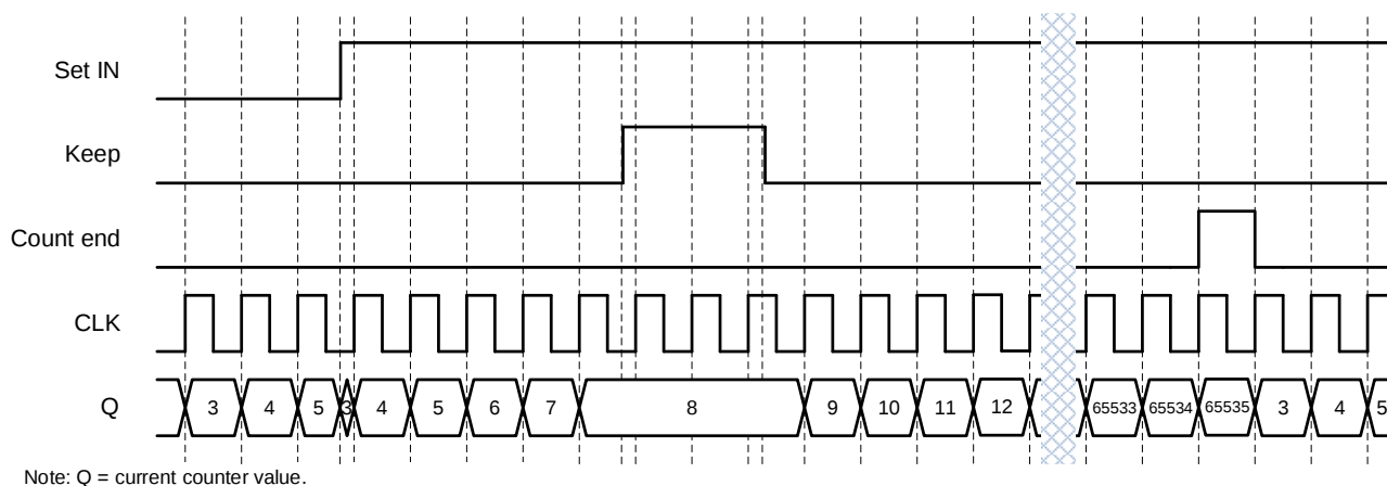
Figure 44. CNT/FSM Timing Diagram (Set Rising Edge Mode, Oscillator is Forced On, UP = 1) for CNT Data = 3
