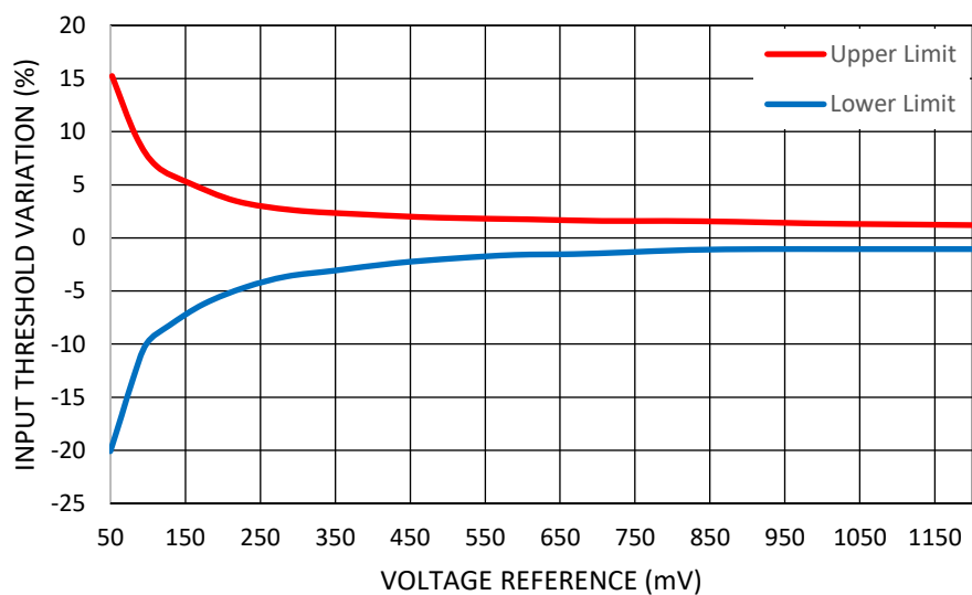
Figure 57. Typical Input Threshold Variation (Including V_{REF} Variation, ACMP Offset) vs. Voltage Reference at T = -40^{\circ}\text{C} to +85^{\circ}\text{C} , LMB Mode - Disable, V_{HYS} = 0\text{ mV}
