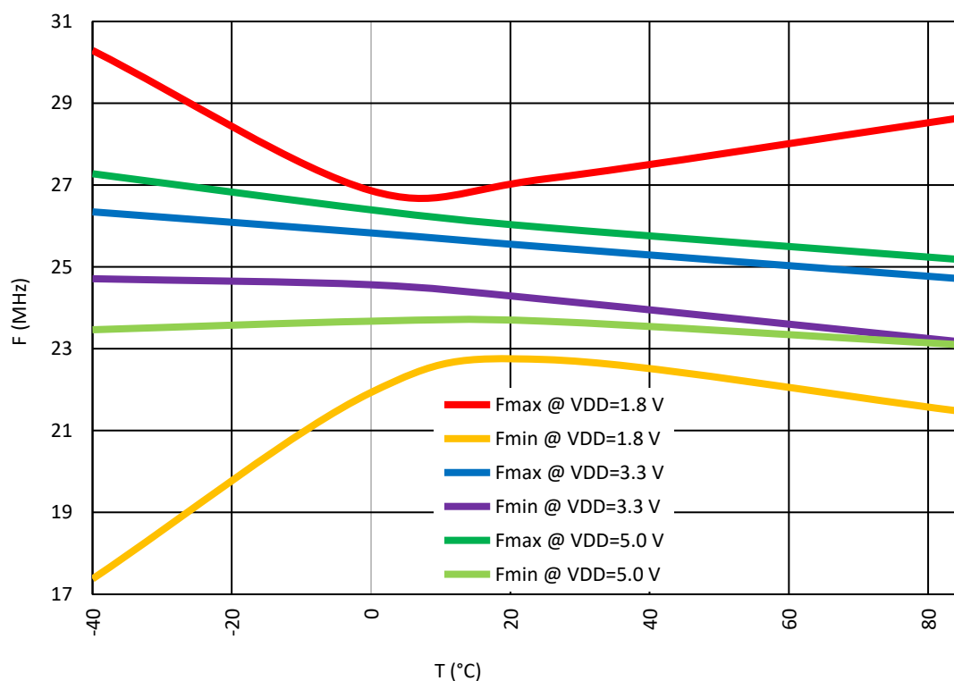
Figure 74. OSC1 (25 MHz) Frequency vs. Temperature
