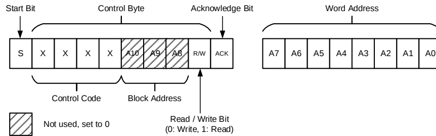
Figure 97. Basic Command Structure
