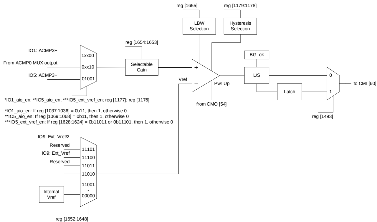
Figure 52. ACMP3 Block Diagram
