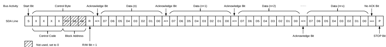
Figure 103. Sequential Read Command
