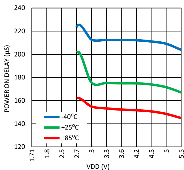
Figure 53. Maximum Power-On Delay vs. V_{DD} , BG = Auto-Delay
