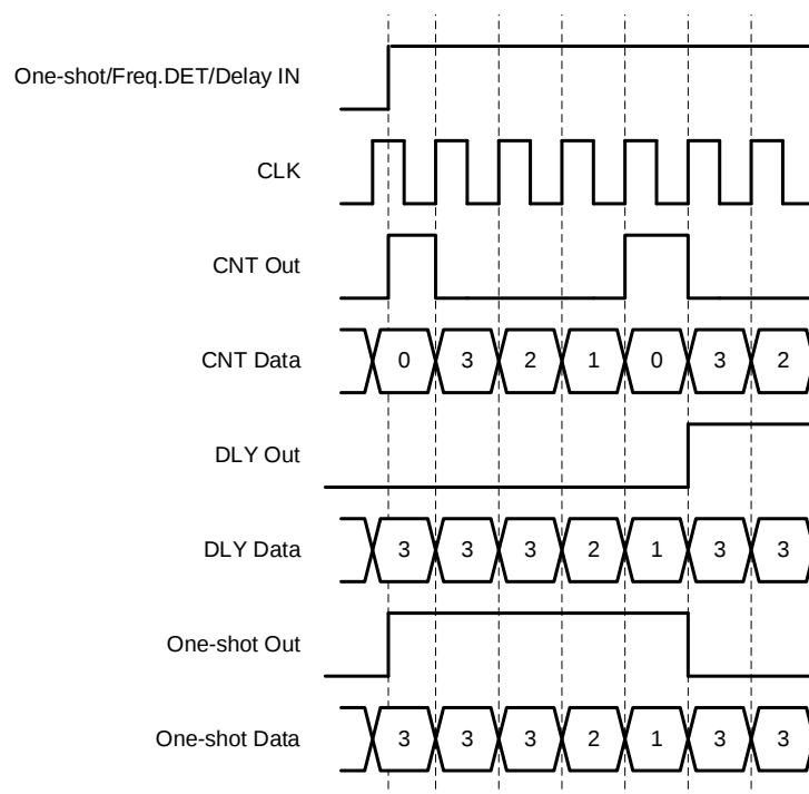
Figure 45. Counter Value, Counter Data = 3
