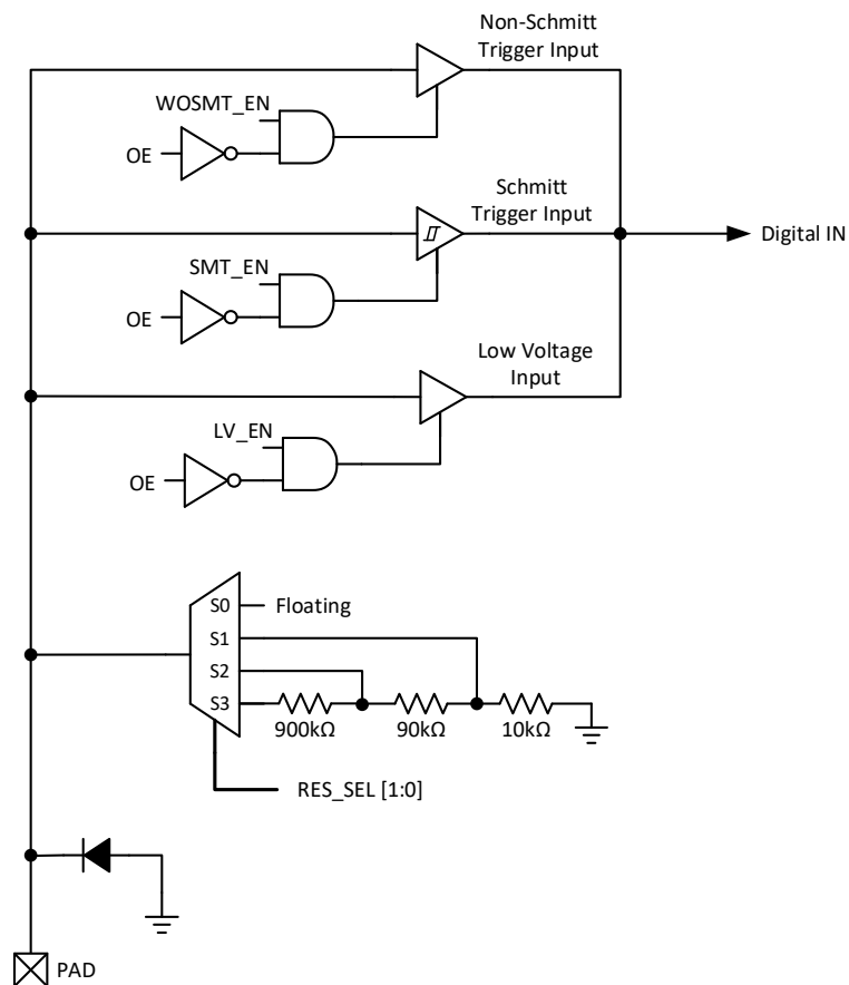
Figure 5. IO0 GPI Structure Diagram
