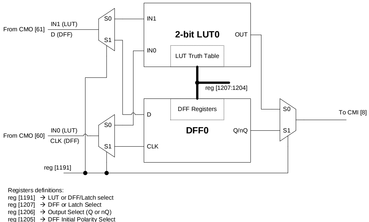
Figure 16. 2-bit LUT0 or DFF0
