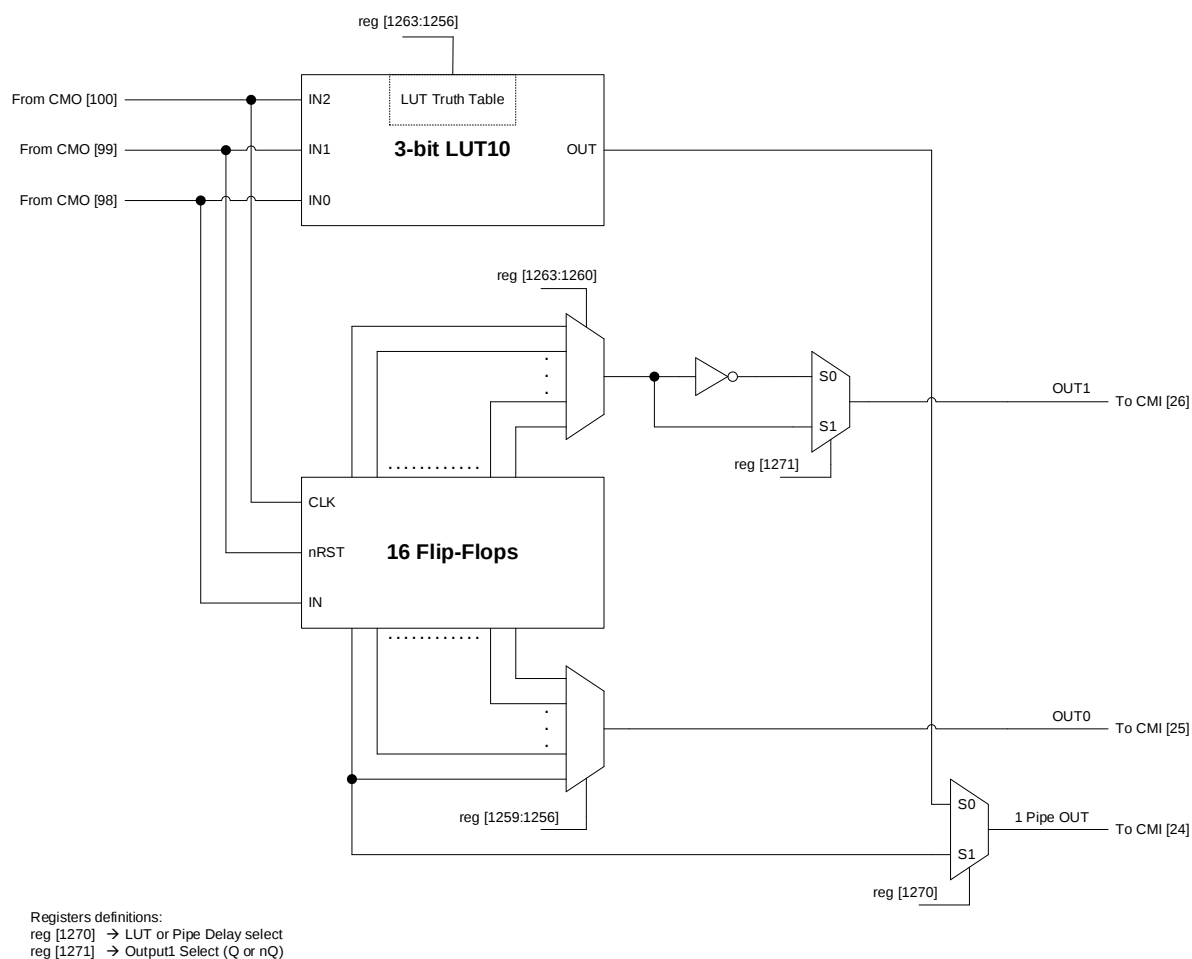
Figure 27. 3-bit LUT10 or Pipe Delay
