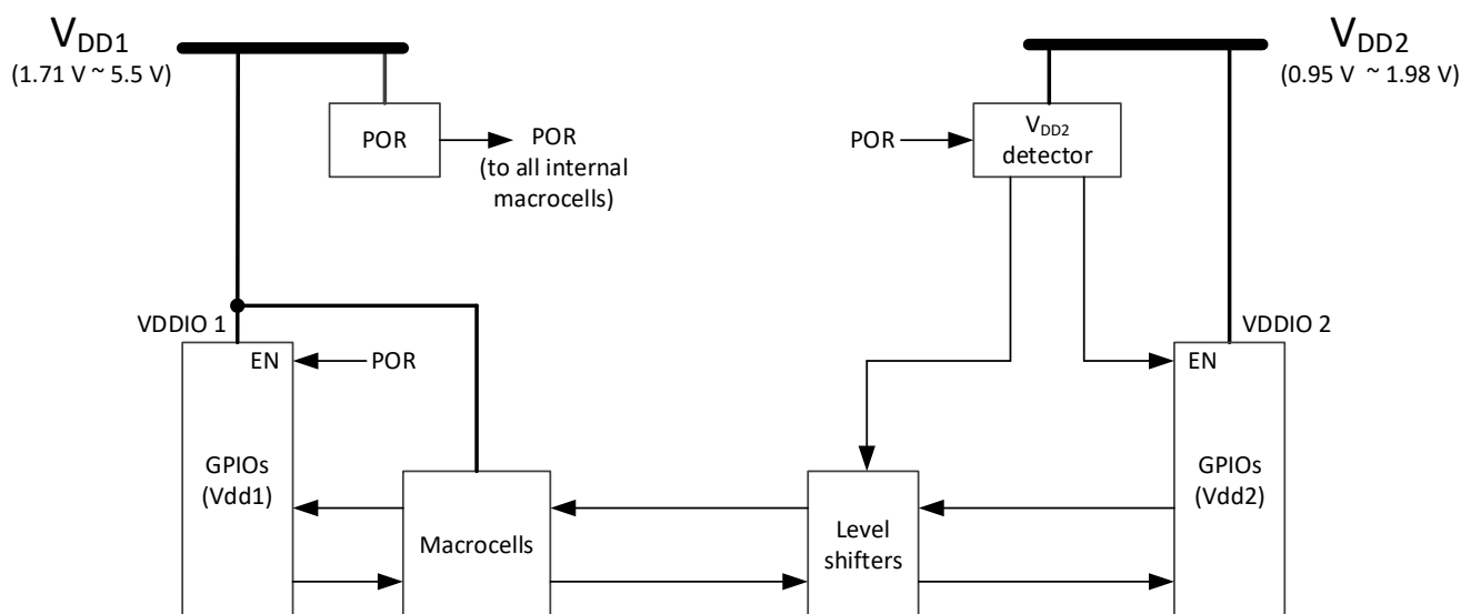
Figure 13. Power Architecture
