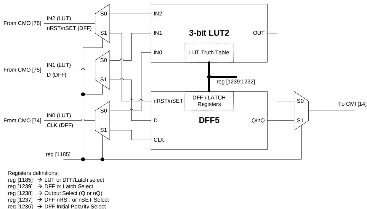
Figure 21. 3-bit LUT2 or DFF5 with RST/SET
