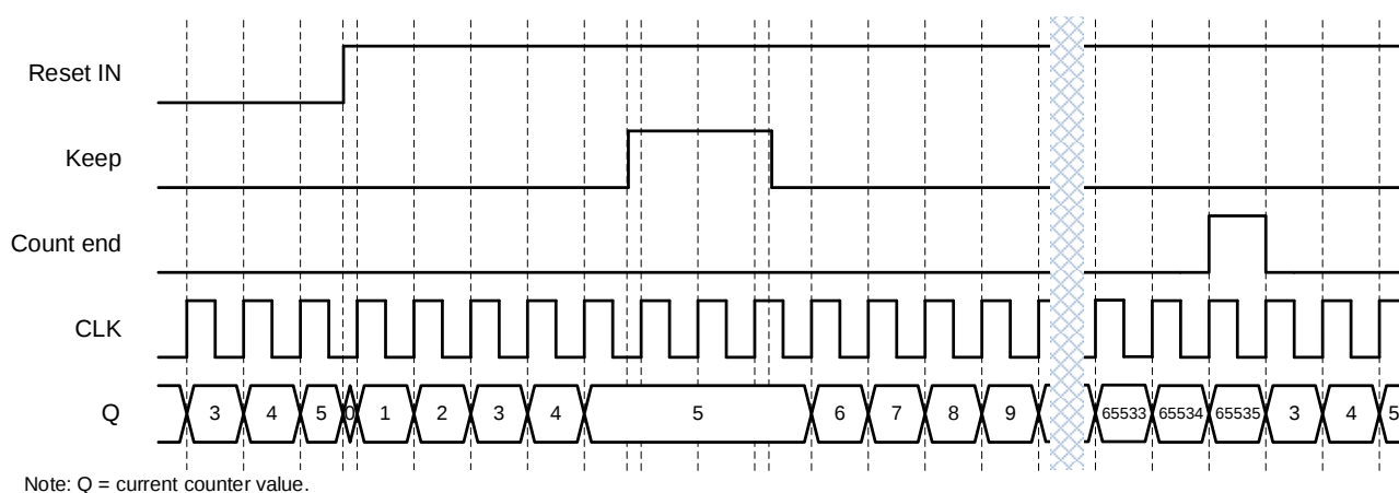
Figure 43. CNT/FSM Timing Diagram (Reset Rising Edge Mode, OSC is Forced On, UP = 1) for CNT Data = 3
