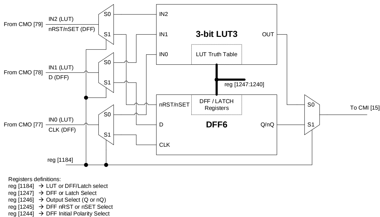
Figure 22. 3-bit LUT3 or DFF6 with RST/SET
