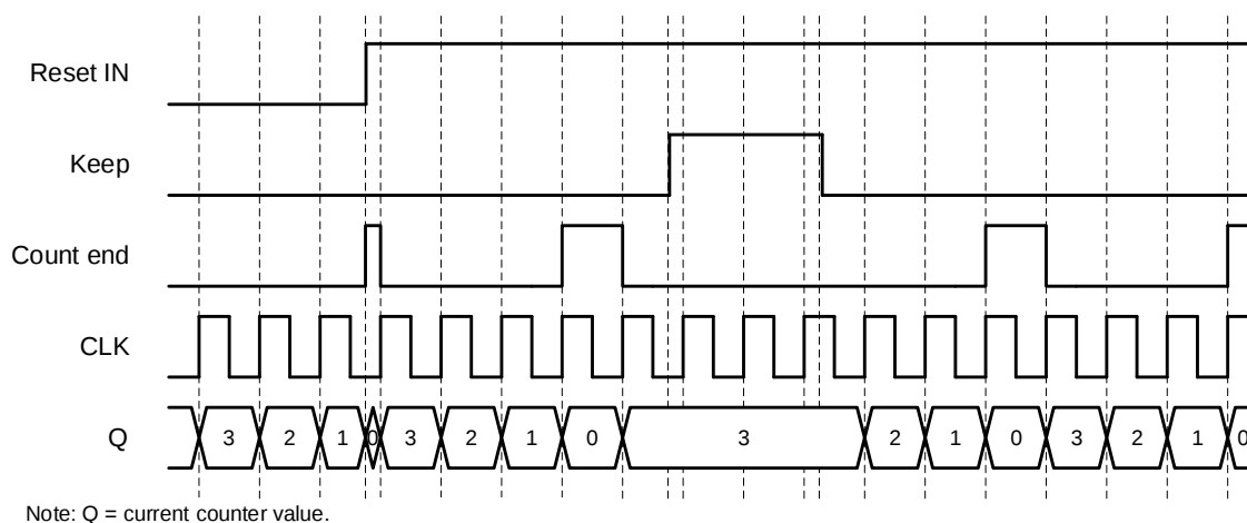
Figure 41. CNT/FSM Timing Diagram (Reset Rising Edge Mode, OSC is Forced On, UP = 0) for CNT Data = 3
