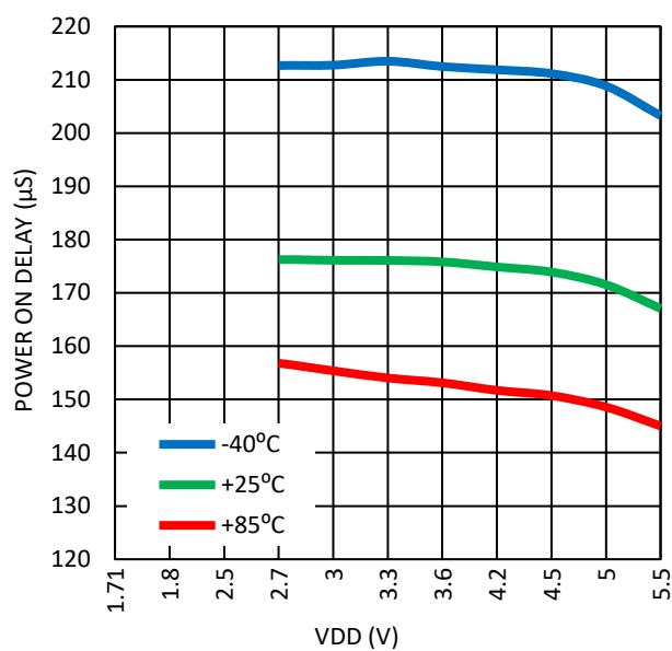
Figure 55. Maximum Power-On Delay vs. V_{DD} , BG = 100 \mu s
