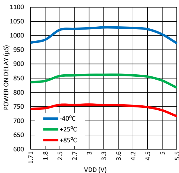
Figure 54. Maximum Power-On Delay vs. V_{DD} , BG = 550 \mu s
