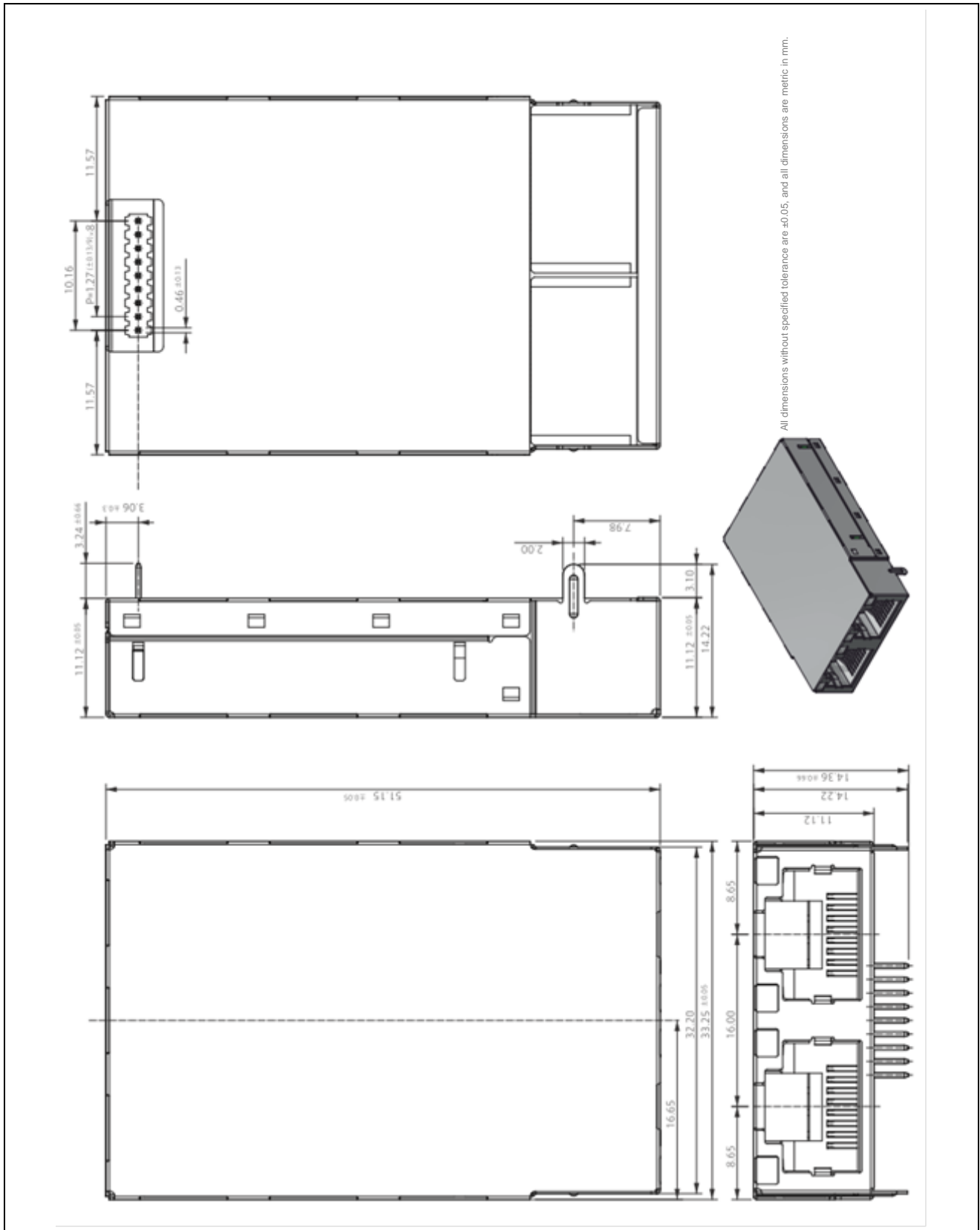
Figure 6.1 Package Dimensions
