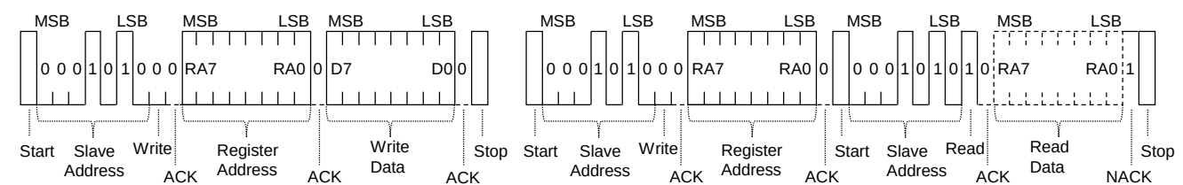
Figure 8.8.1(a) SDA data format (Slave, Write)
