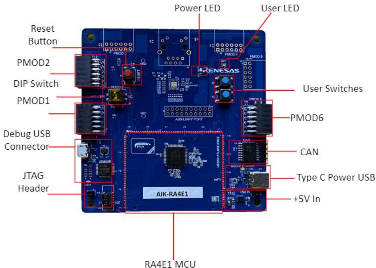
Figure 1. AIK-RA4E1 Top Side
