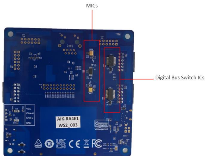
Figure 2. AIK-RA4E1 Bottom Side
